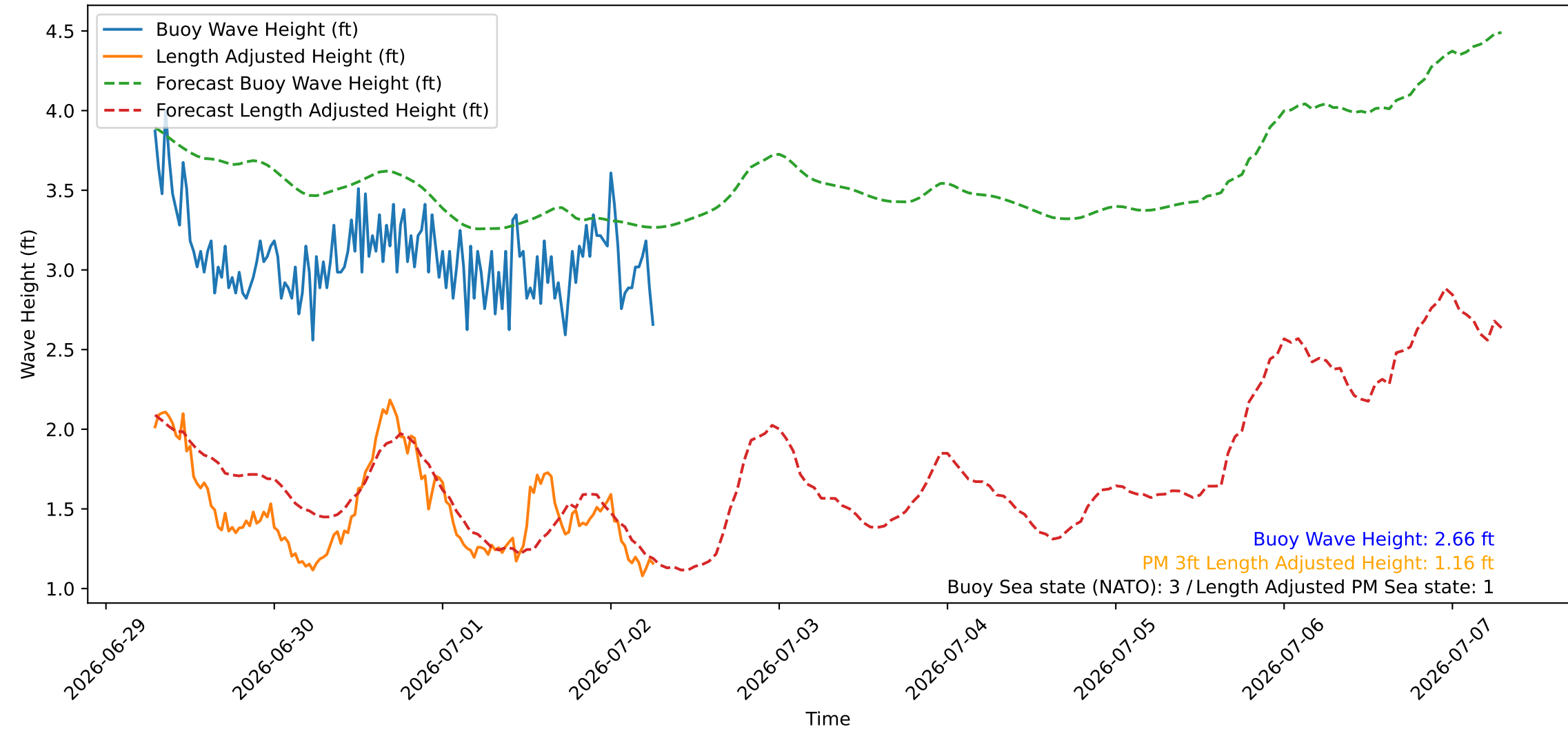
Wave Heights over Time for Oceanside Harbor at 2026-07-02 06:50:26
