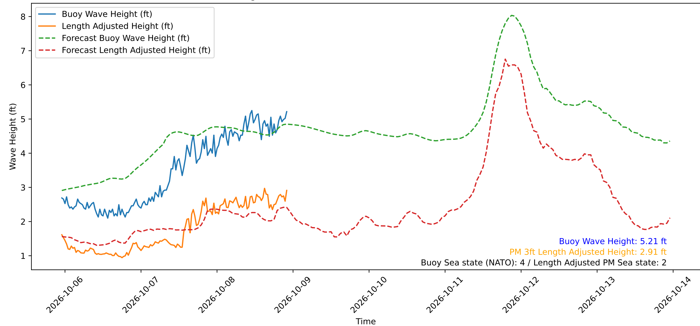
Wave Heights over Time for Green Beach at 2026-10-08 22:41:11
