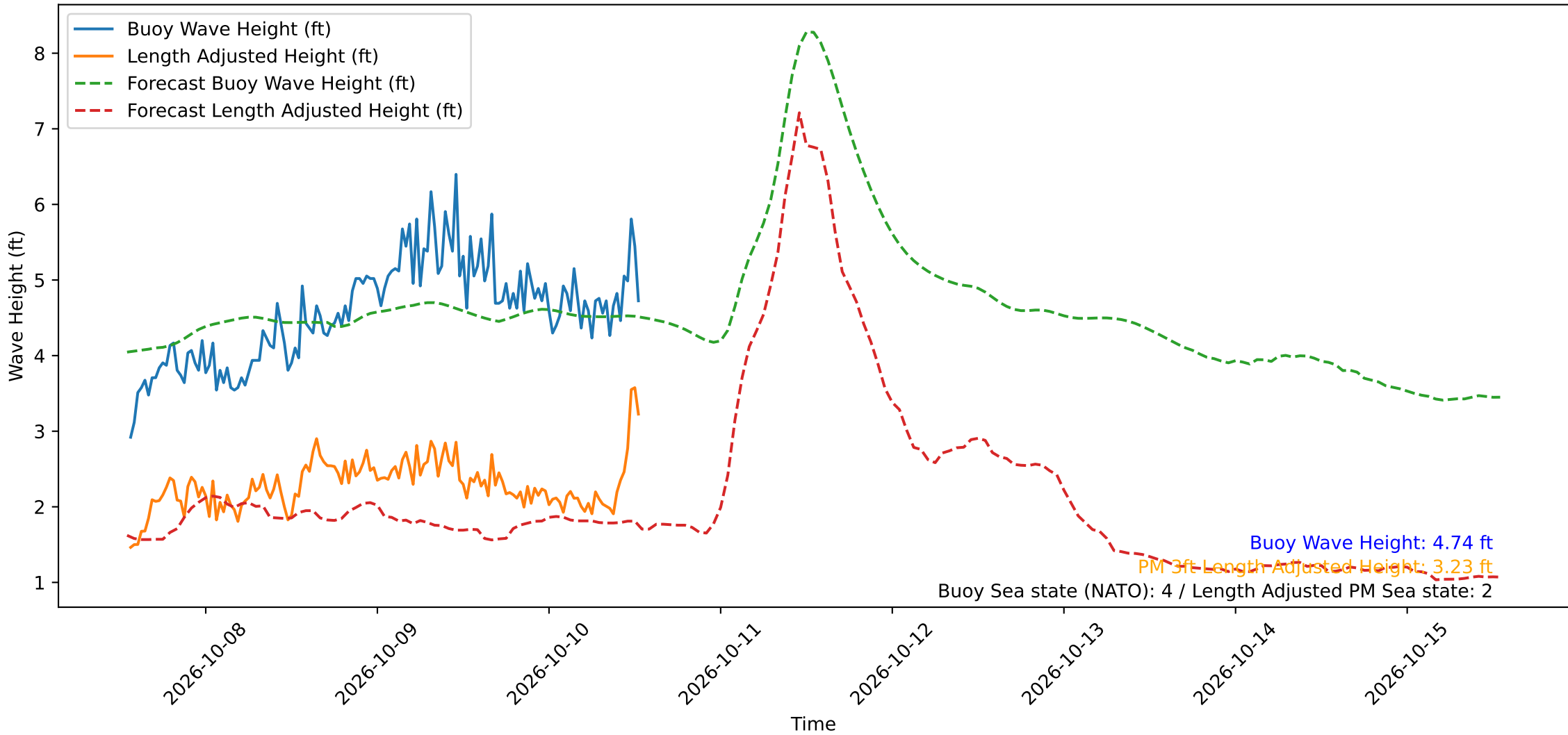
Wave Heights over Time for Oceanside Harbor at 2026-10-10 13:20:29
