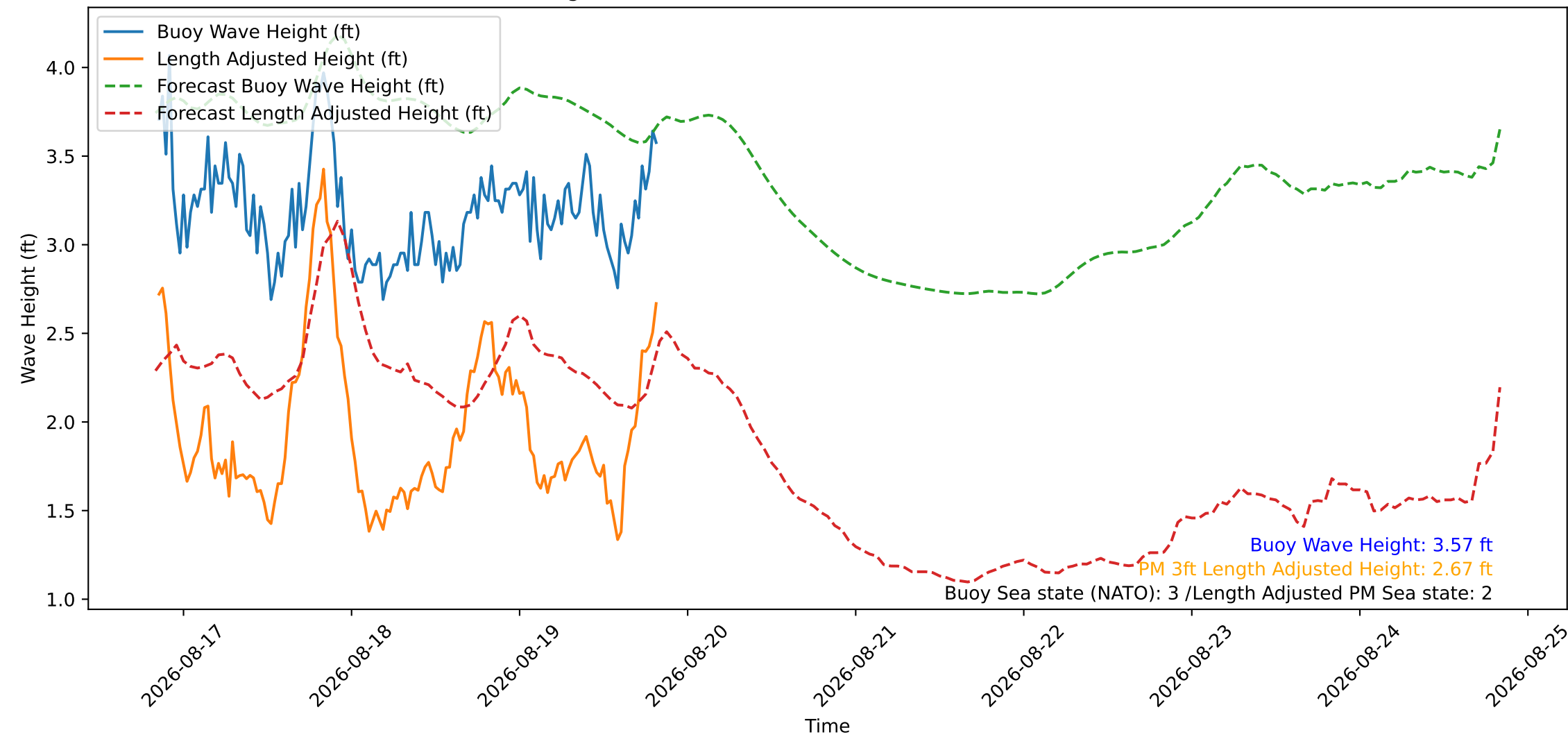
Wave Heights over Time for Green Beach at 2026-08-19 20:21:13
