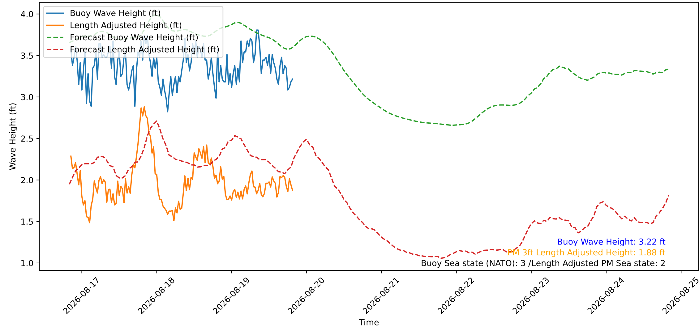
Wave Heights over Time for Oceanside Harbor at 2026-08-19 20:20:28
