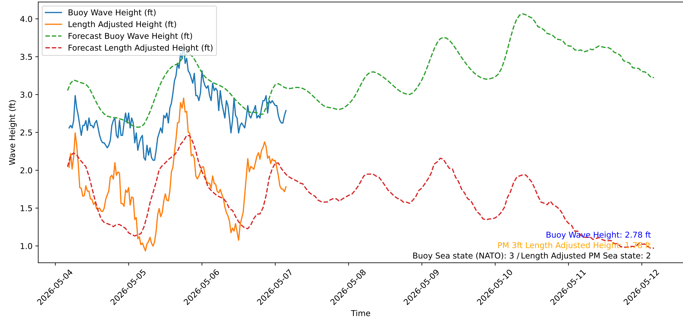
Wave Heights over Time for Green Beach at 2026-05-07 04:21:13
