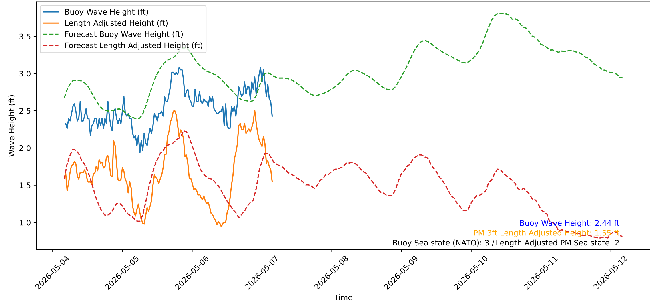
Wave Heights over Time for Red Beach at 2026-05-07 04:20:51
