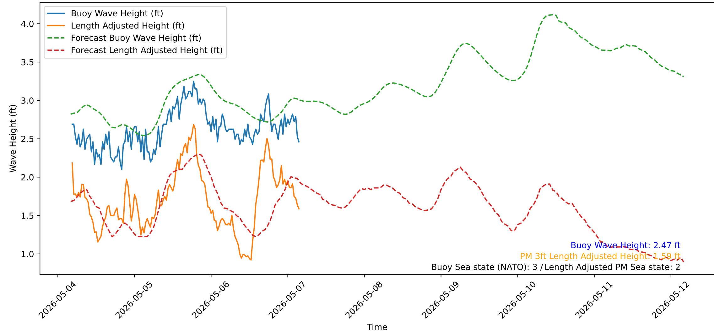
Wave Heights over Time for Oceanside Harbor at 2026-05-07 04:20:31
