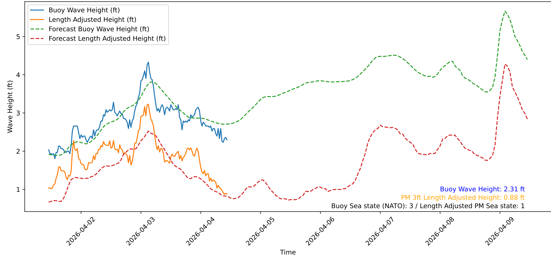
Wave Heights over Time for Green Beach at 2026-04-04 11:11:10
