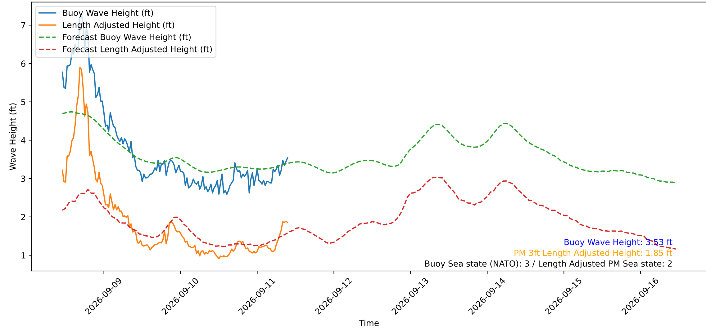
Wave Heights over Time for Green Beach at 2026-09-11 10:31:14
