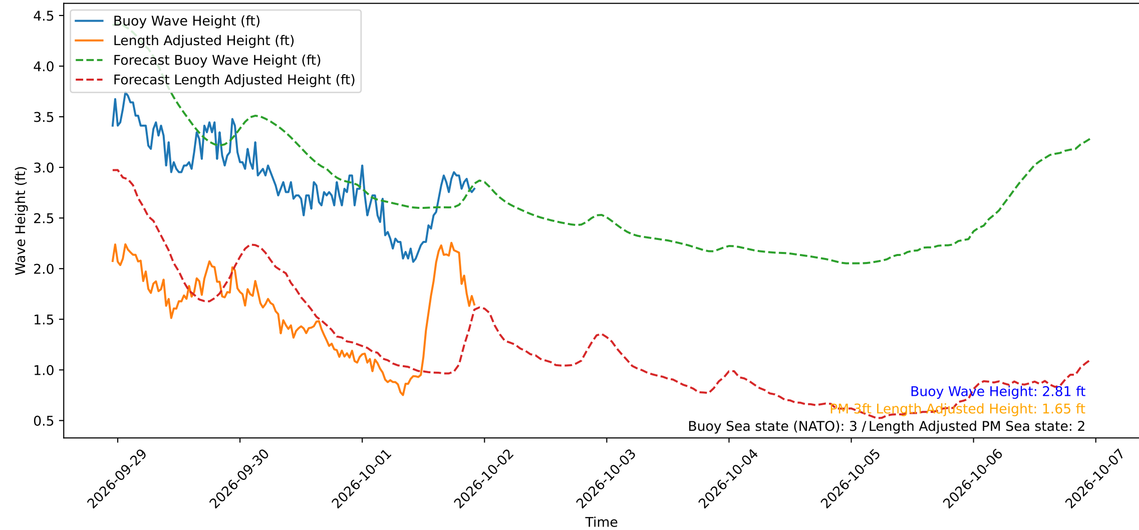
Wave Heights over Time for Red Beach at 2026-10-01 22:40:49
