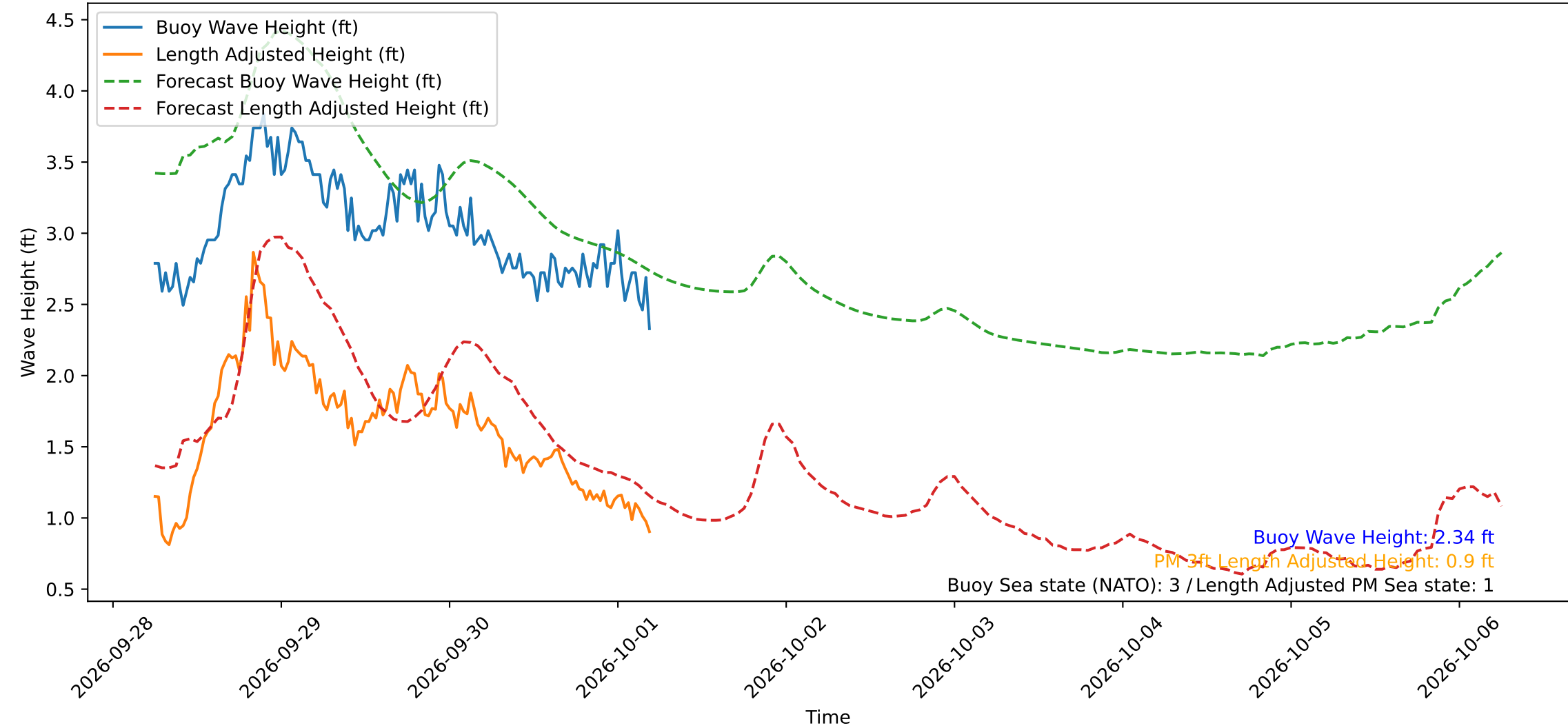
Wave Heights over Time for Red Beach at 2026-10-01 05:30:50
