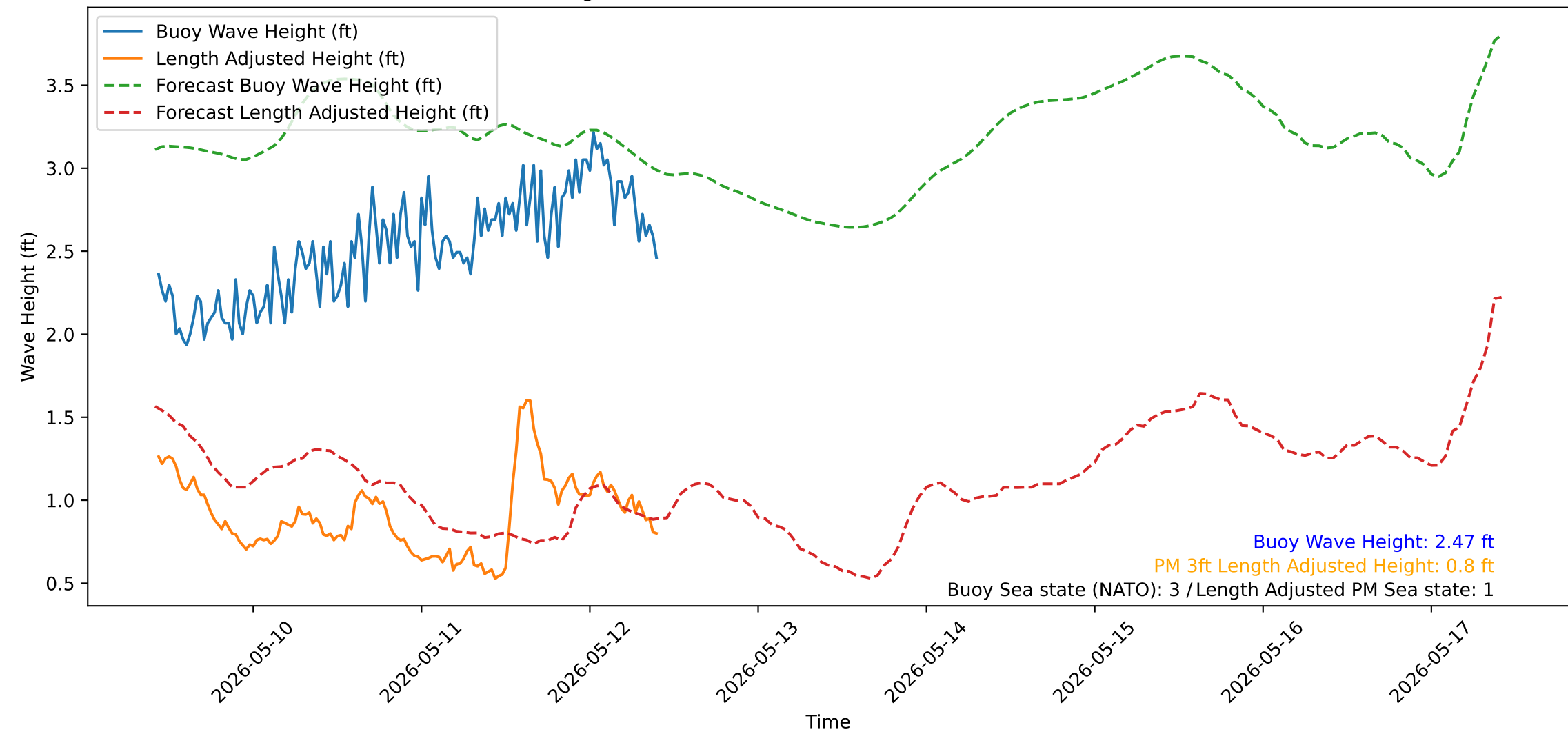
Wave Heights over Time for Red Beach at 2026-05-12 10:20:52
