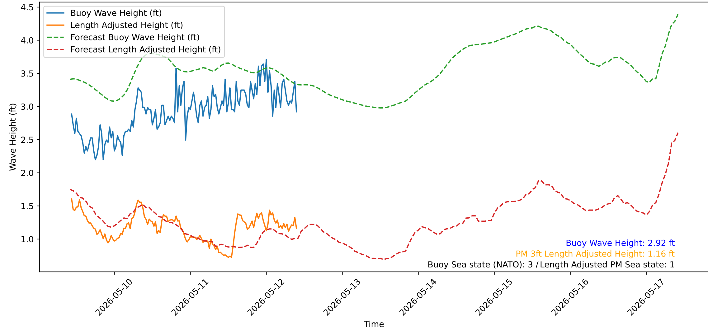
Wave Heights over Time for Oceanside Harbor at 2026-05-12 10:20:32
