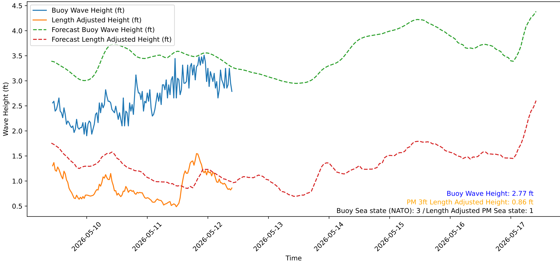
Wave Heights over Time for Green Beach at 2026-05-12 10:21:14
