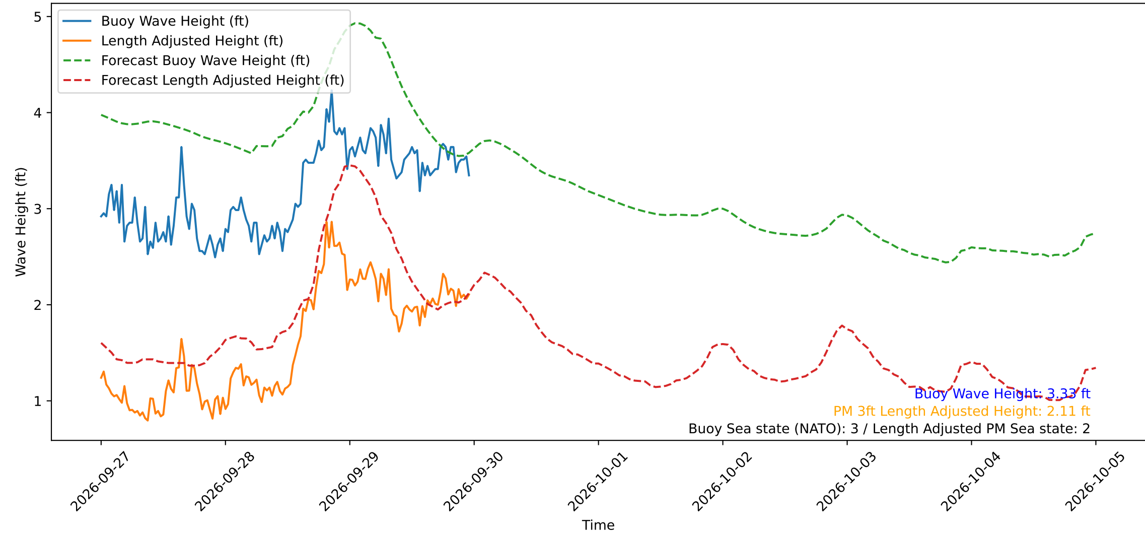
Wave Heights over Time for Oceanside Harbor at 2026-09-30 00:00:29
