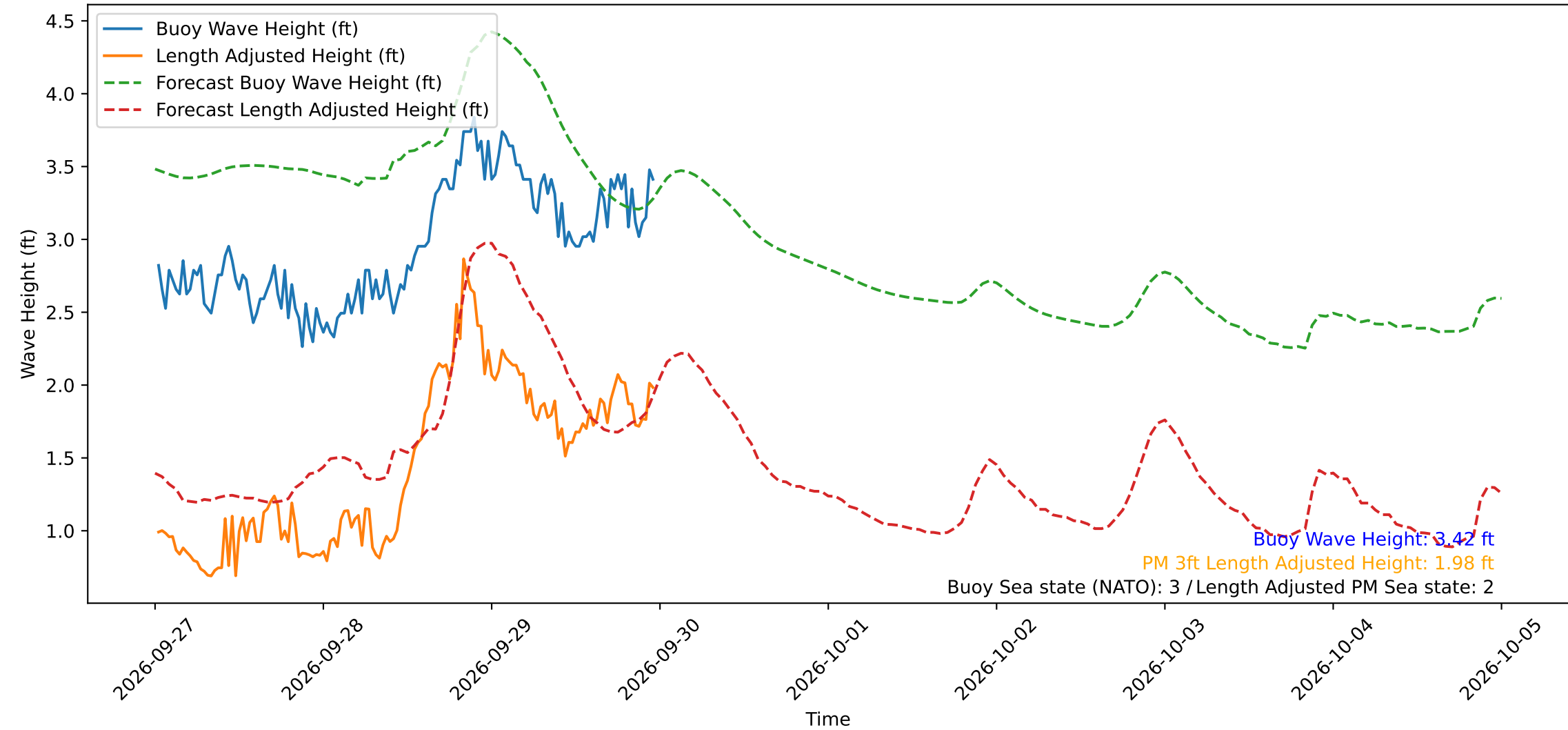
Wave Heights over Time for Red Beach at 2026-09-30 00:00:49
