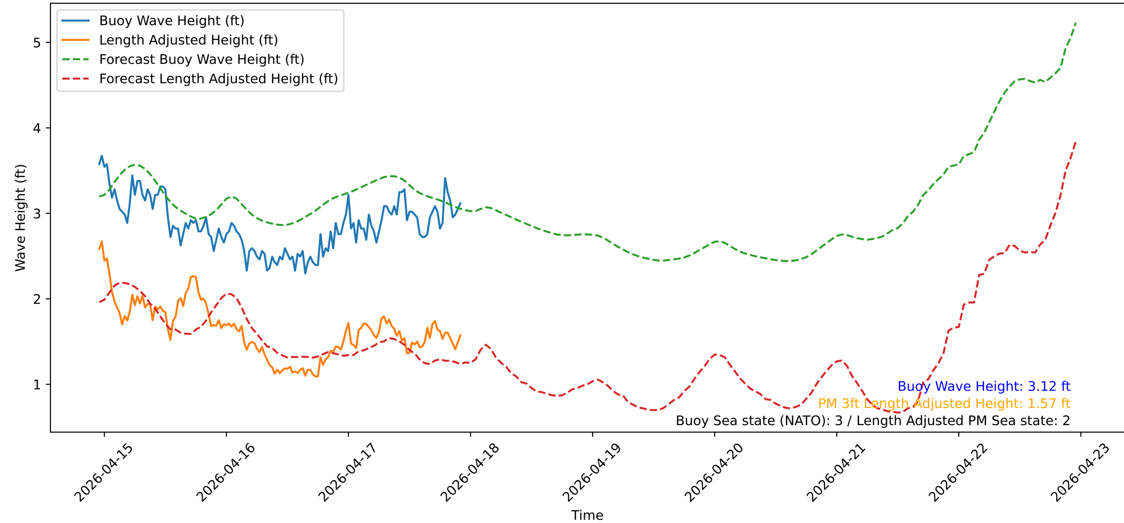
Wave Heights over Time for Oceanside Harbor at 2026-04-17 22:50:31
