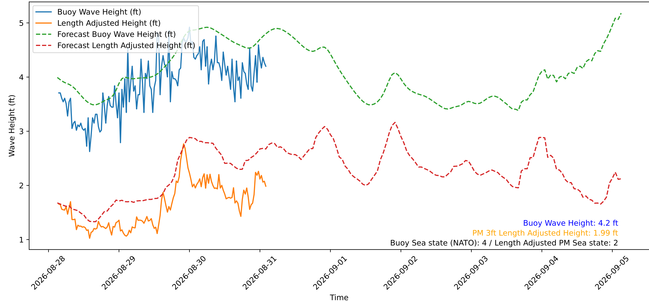
Wave Heights over Time for Green Beach at 2026-08-31 03:01:12
