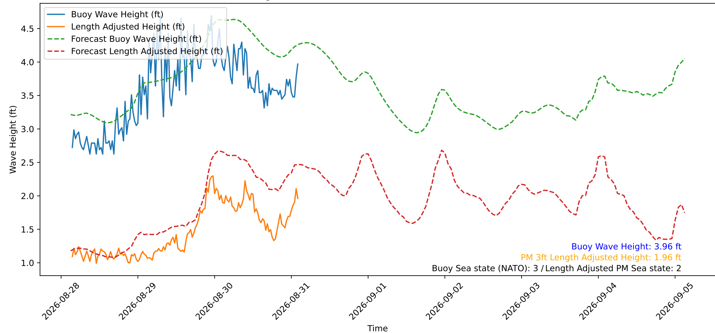
Wave Heights over Time for Red Beach at 2026-08-31 03:00:49
