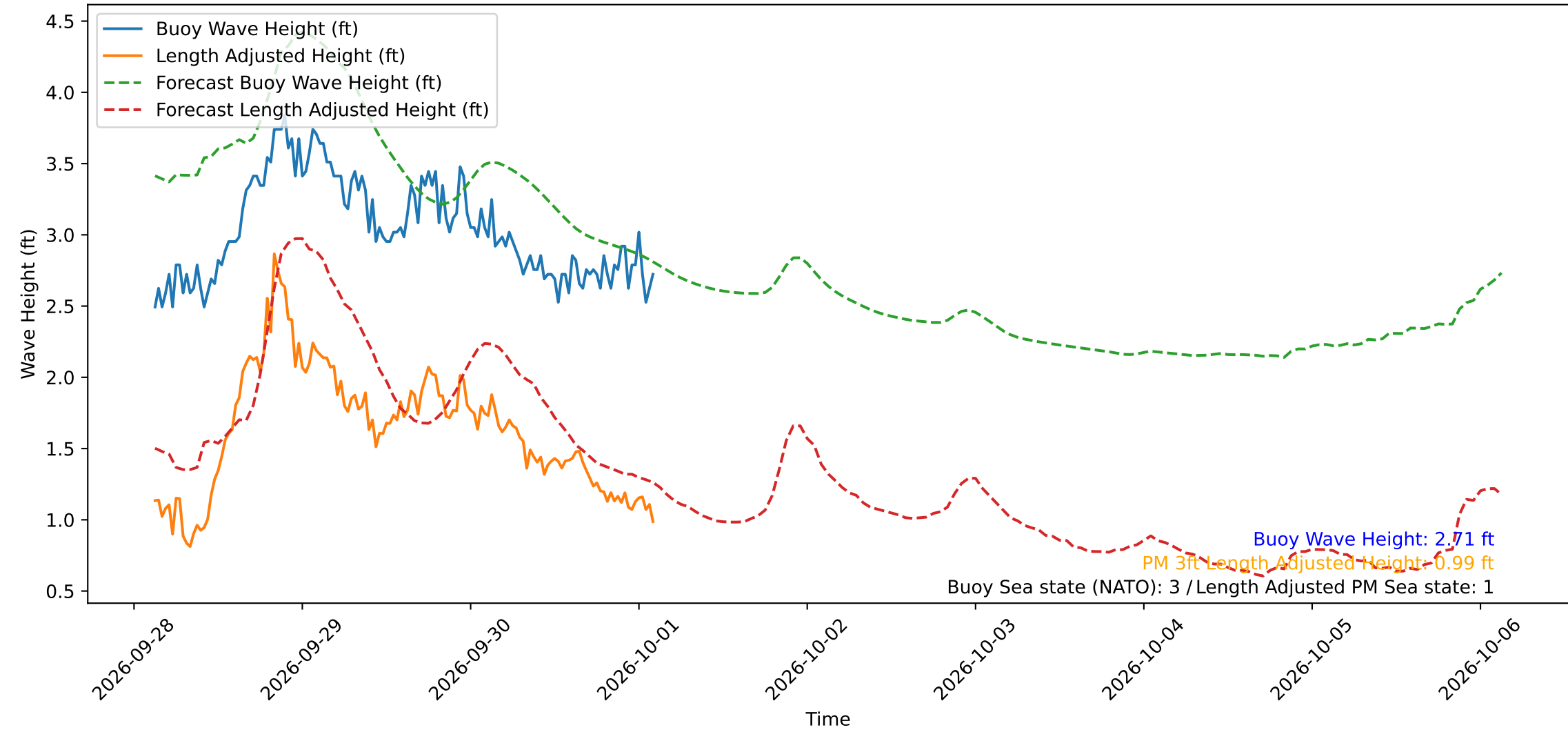
Wave Heights over Time for Red Beach at 2026-10-01 02:50:51
