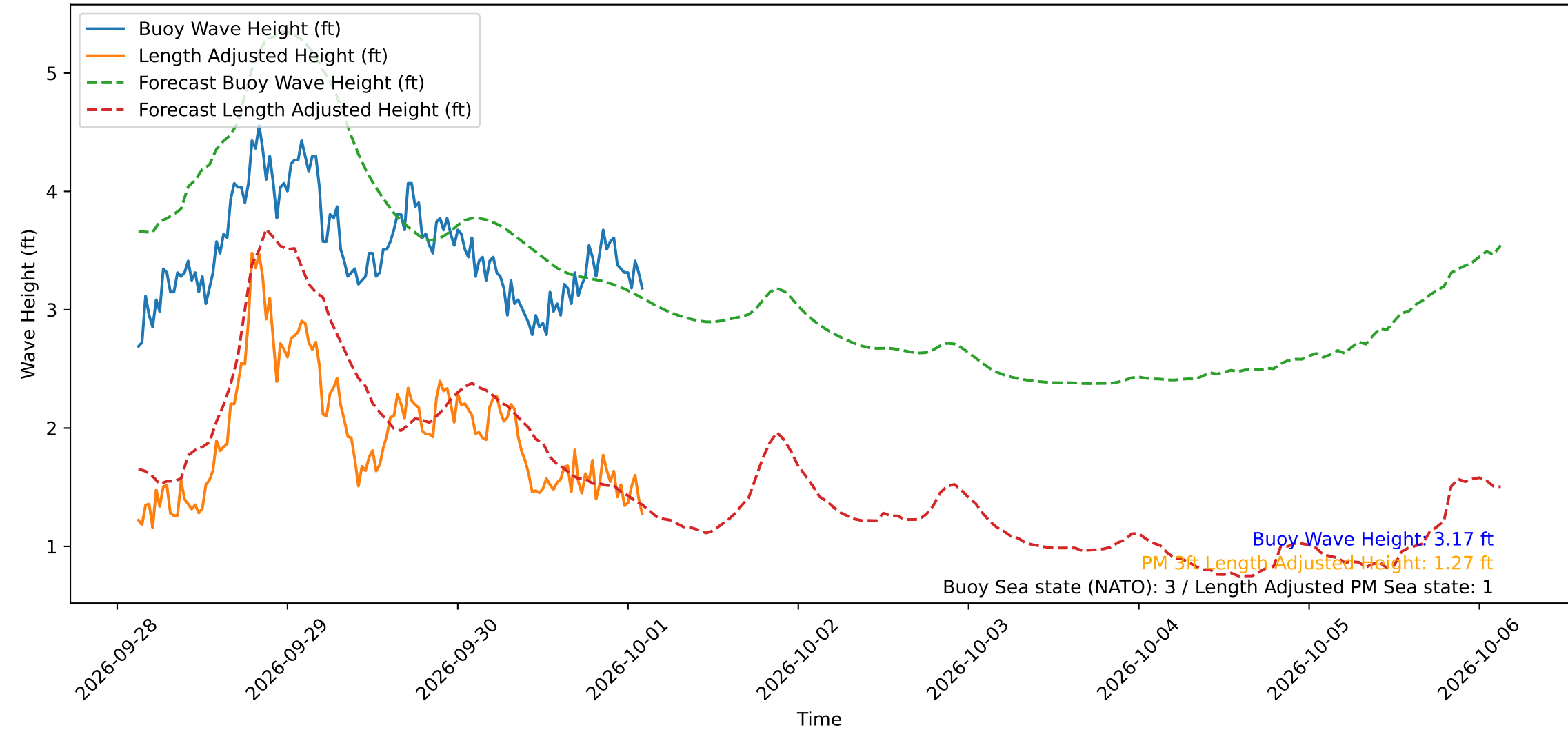
Wave Heights over Time for Green Beach at 2026-10-01 02:51:15
