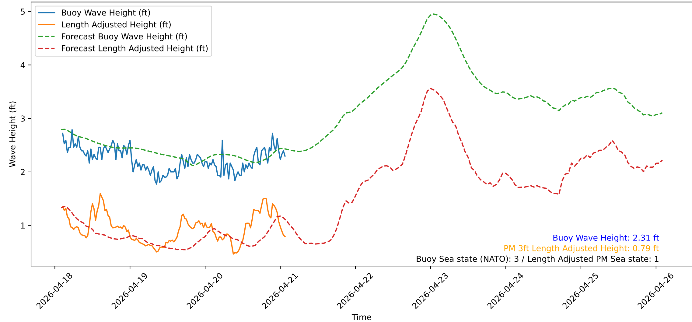
Wave Heights over Time for Red Beach at 2026-04-21 02:10:51
