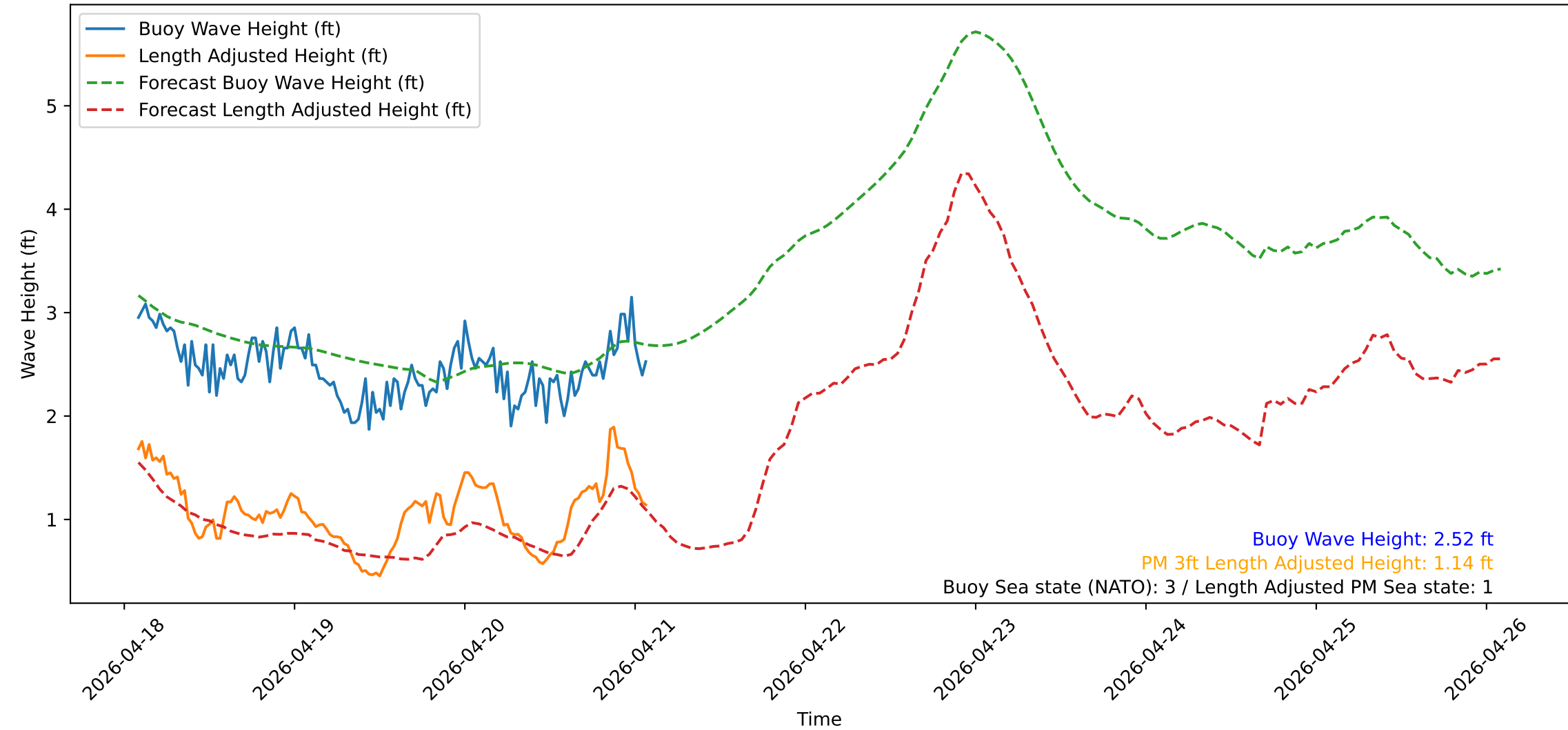
Wave Heights over Time for Green Beach at 2026-04-21 02:11:14
