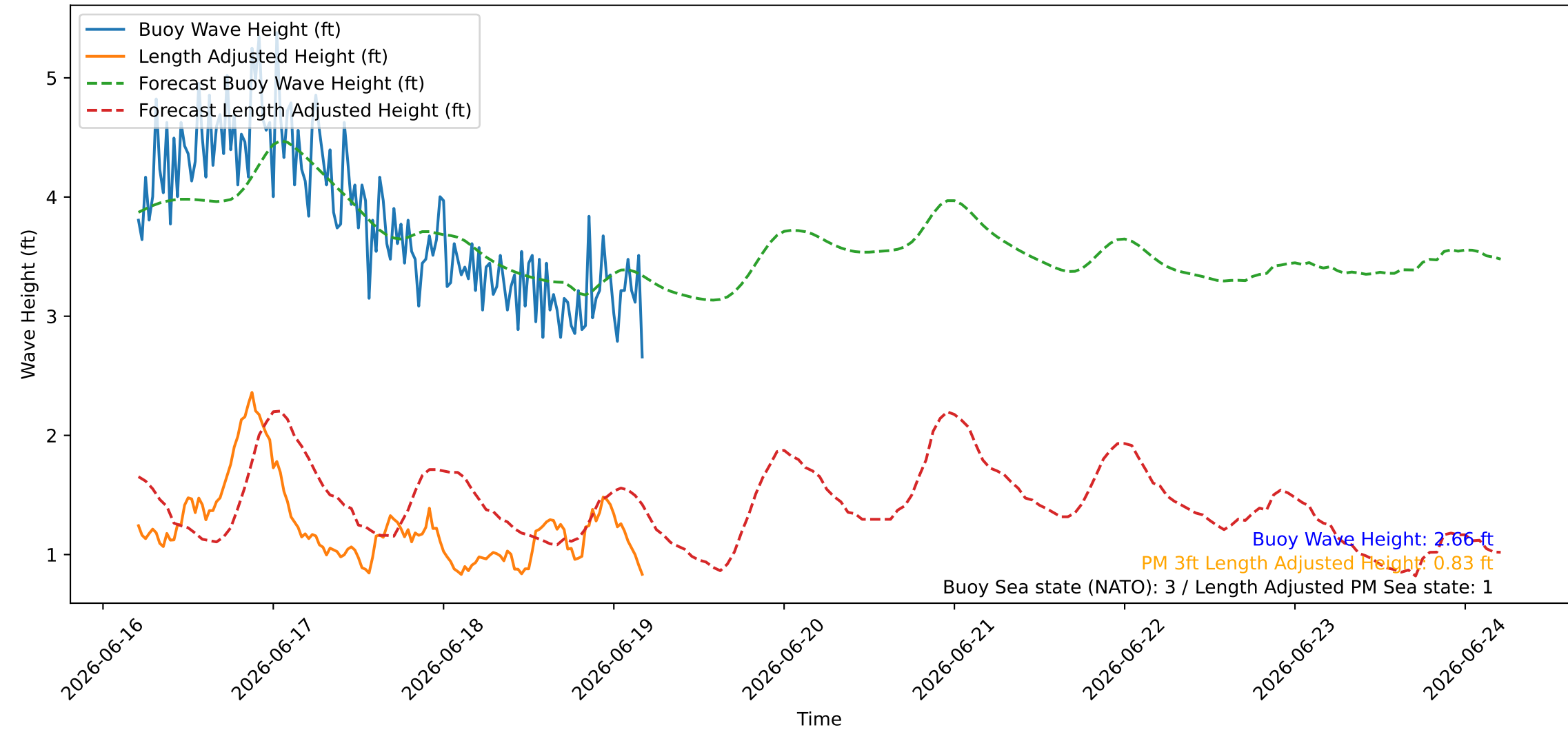
Wave Heights over Time for Red Beach at 2026-06-19 04:50:47
