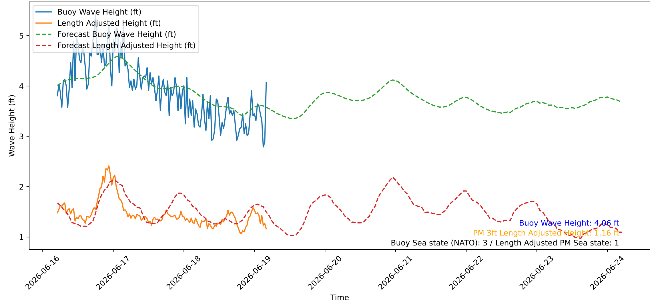
Wave Heights over Time for Oceanside Harbor at 2026-06-19 04:50:26
