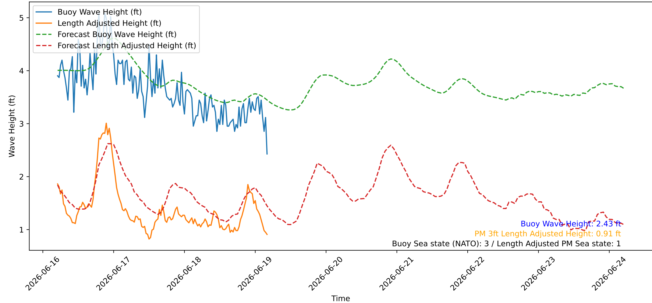
Wave Heights over Time for Green Beach at 2026-06-19 04:51:09
