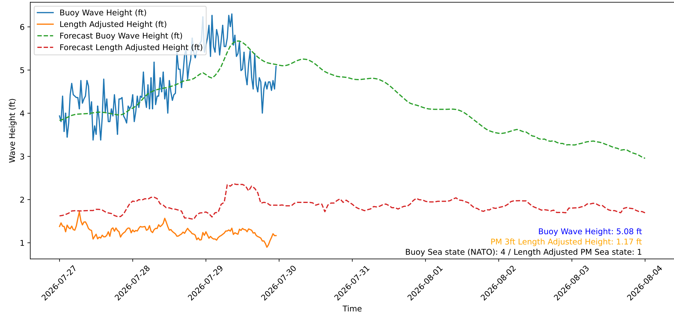
Wave Heights over Time for Green Beach at 2026-07-30 00:01:09
