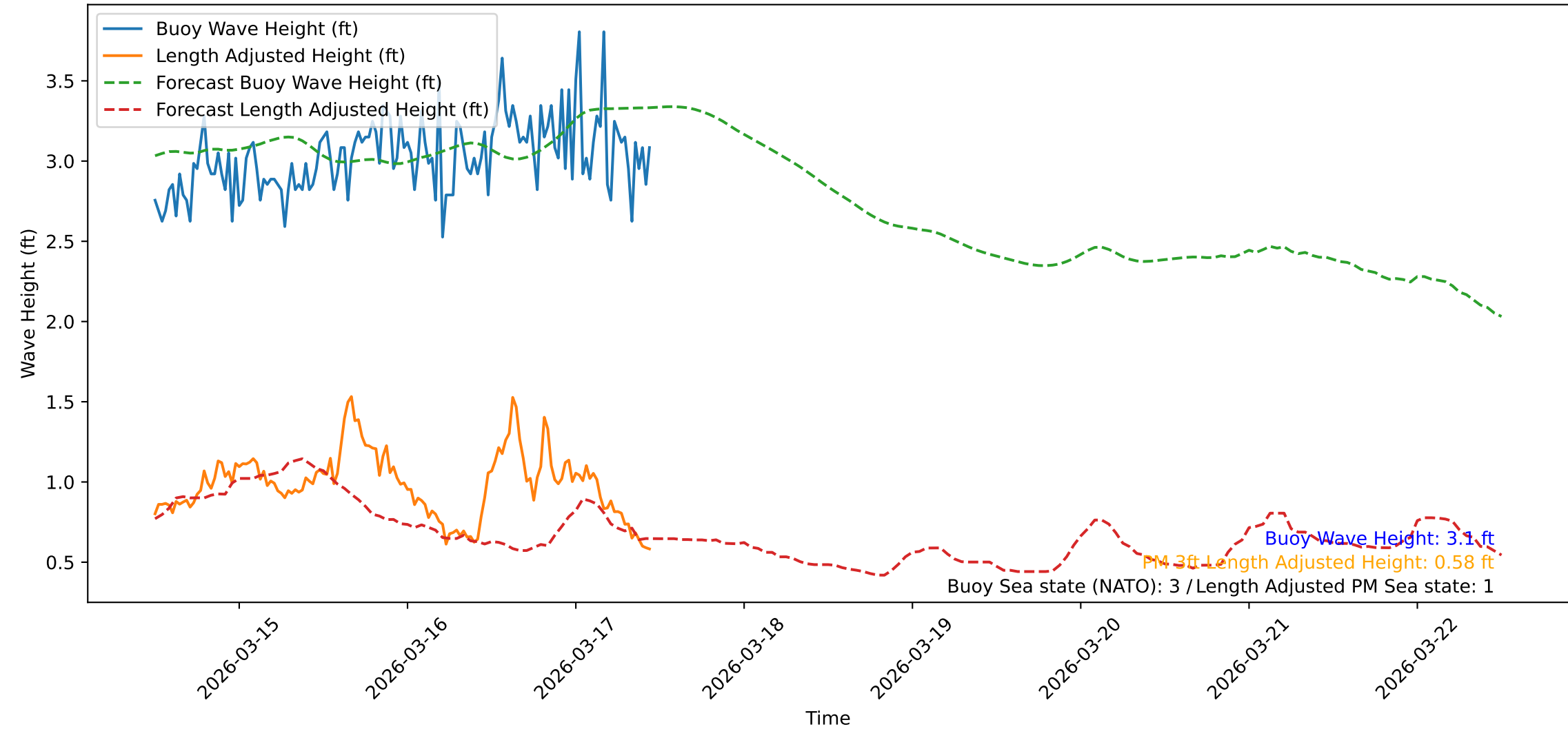
Wave Heights over Time for Red Beach at 2026-03-17 11:31:05
