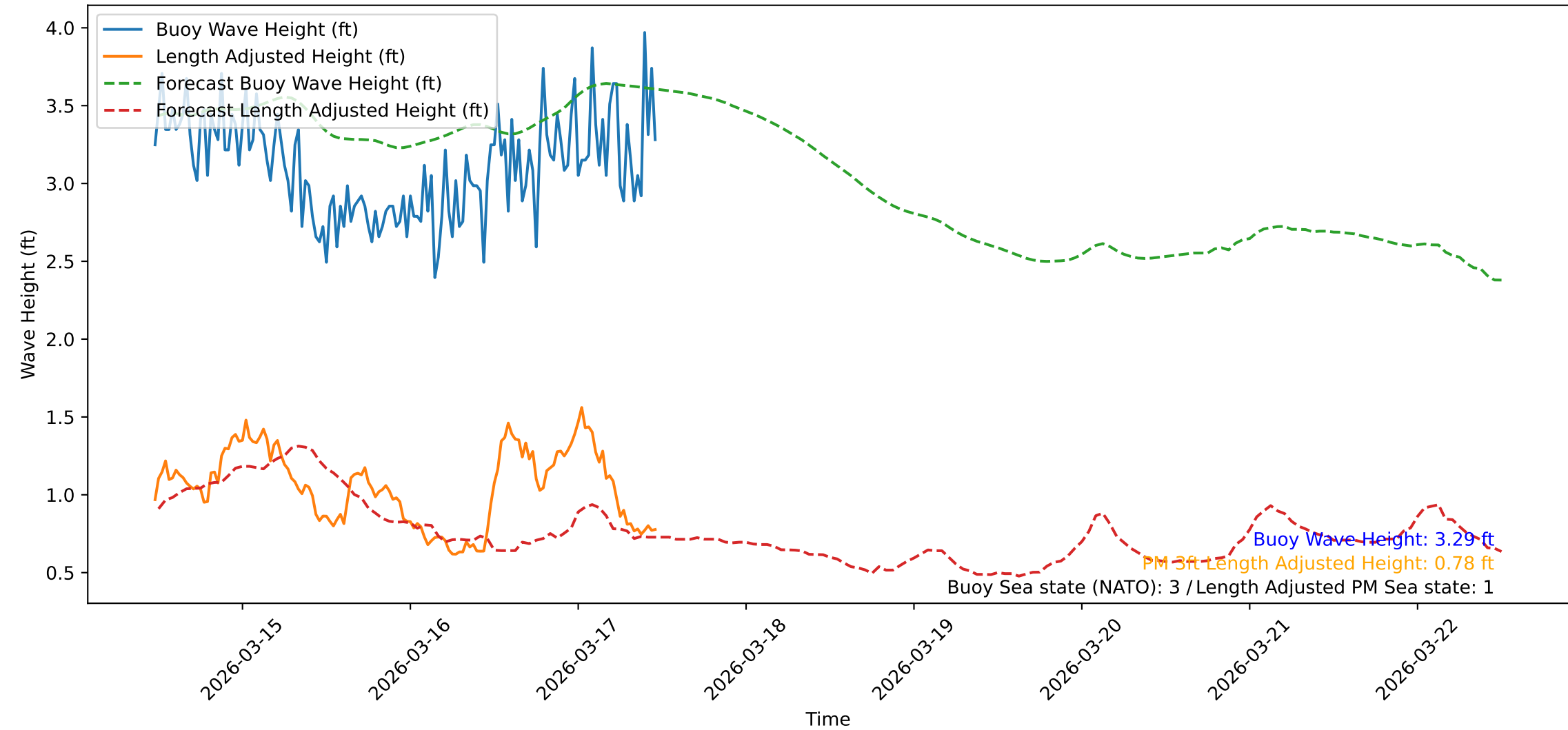
Wave Heights over Time for Oceanside Harbor at 2026-03-17 11:30:43
