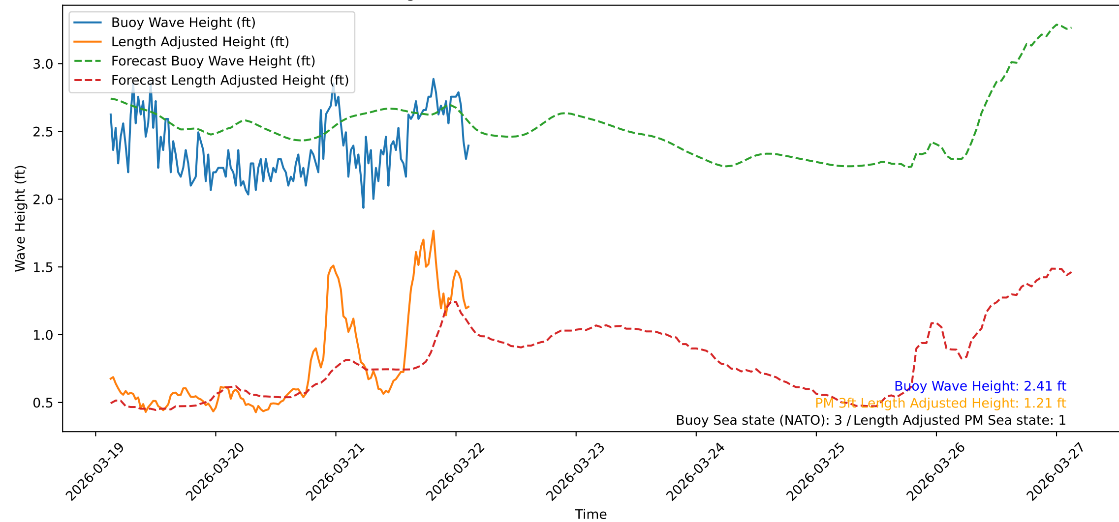
Wave Heights over Time for Green Beach at 2026-03-22 03:11:11
