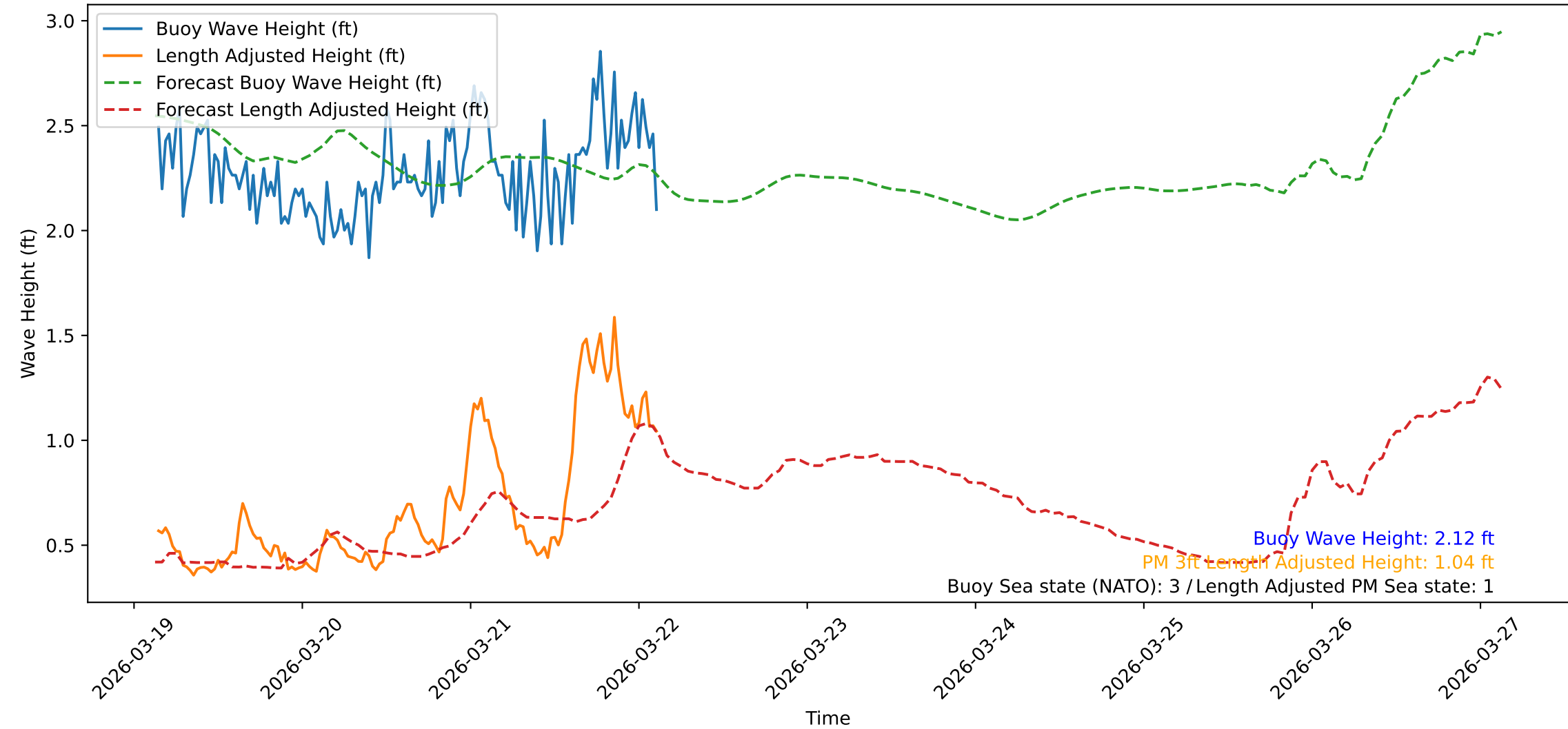
Wave Heights over Time for Red Beach at 2026-03-22 03:10:48
