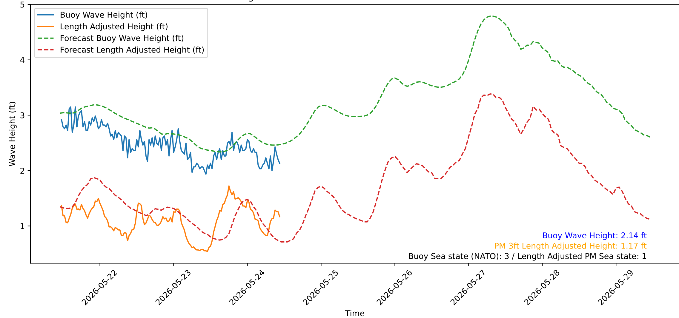
Wave Heights over Time for Red Beach at 2026-05-24 11:20:53
