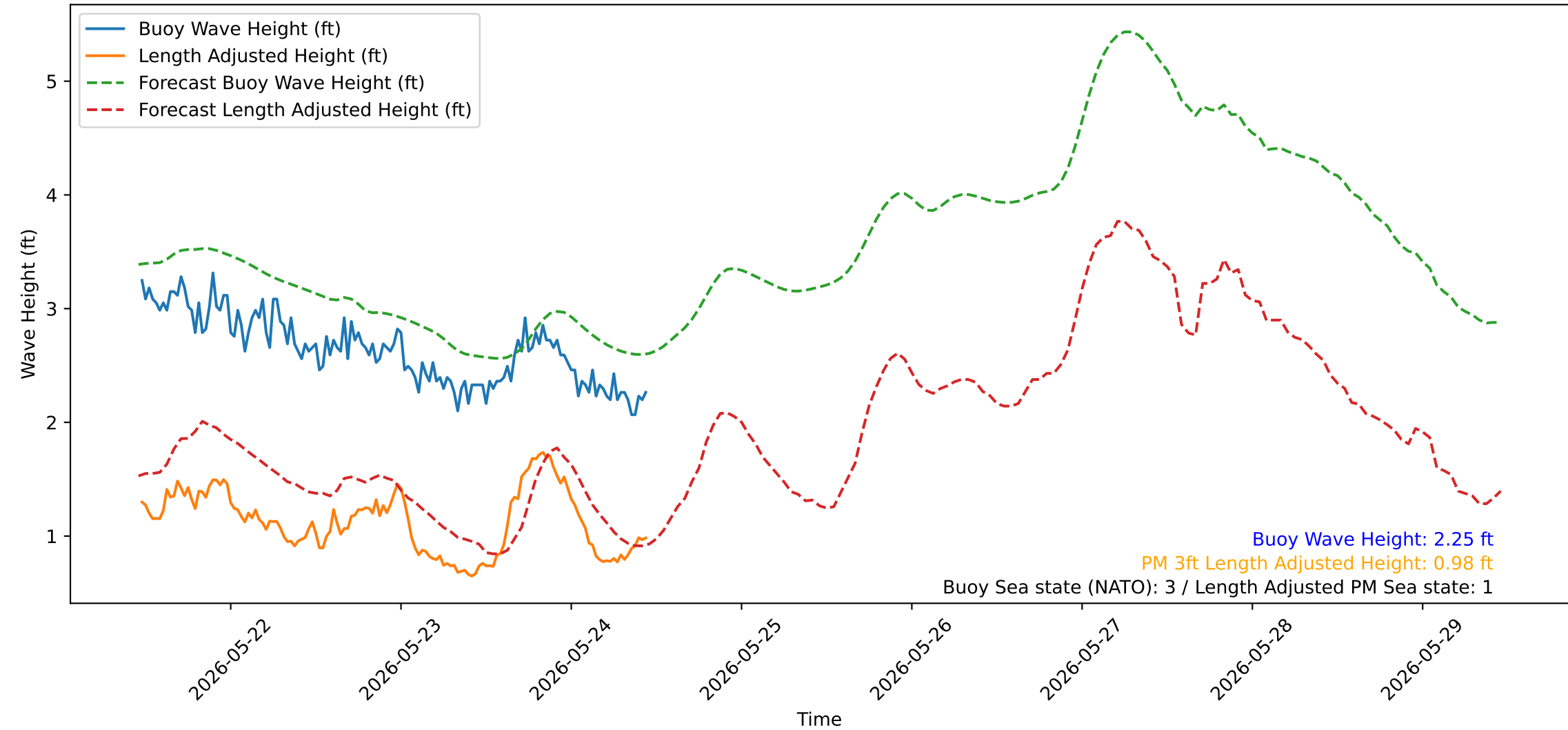
Wave Heights over Time for Green Beach at 2026-05-24 11:21:16
