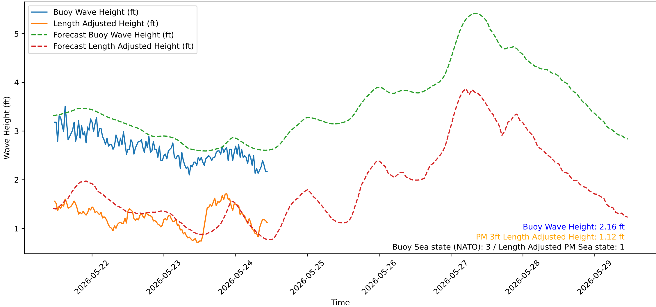
Wave Heights over Time for Oceanside Harbor at 2026-05-24 11:20:32
