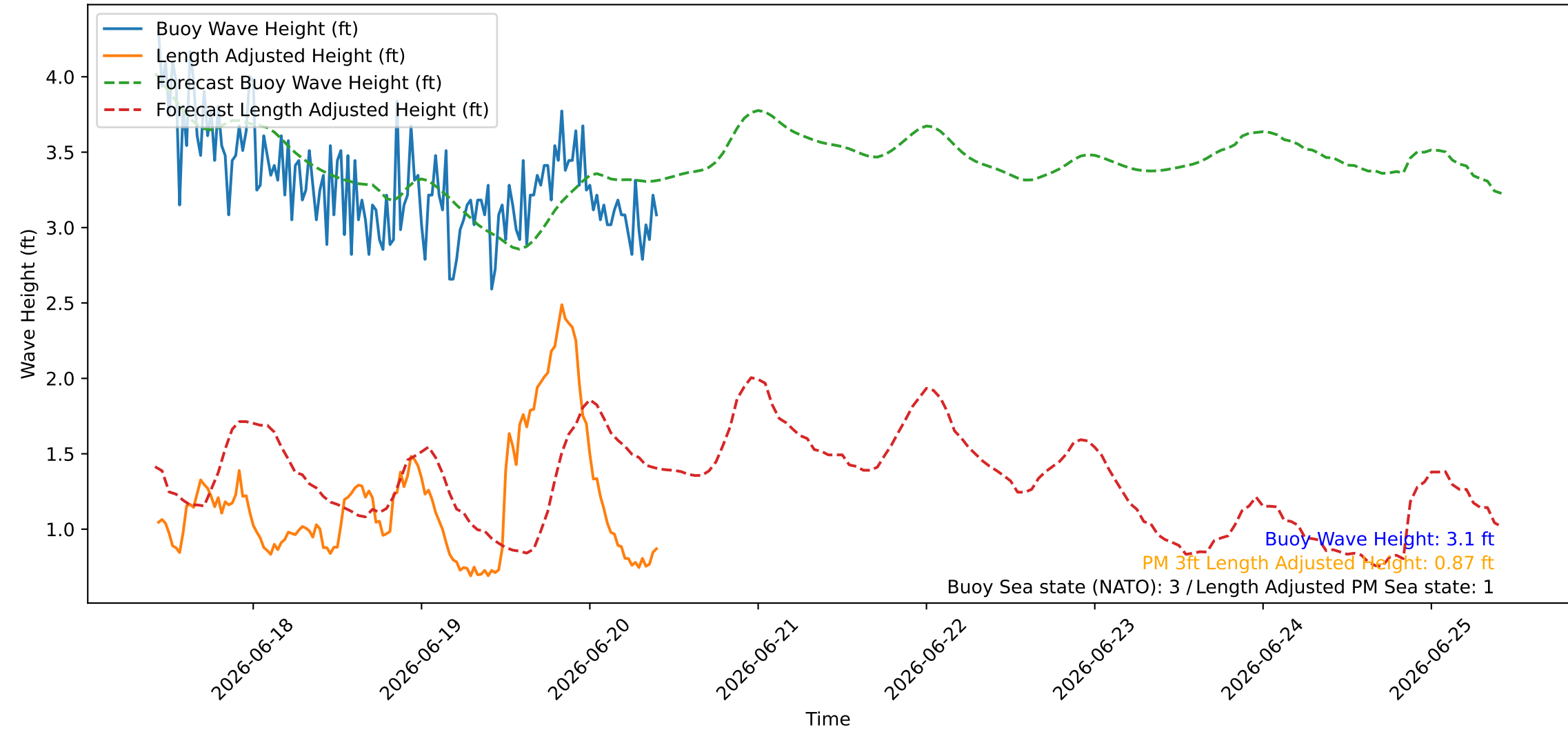
Wave Heights over Time for Red Beach at 2026-06-20 10:20:47
