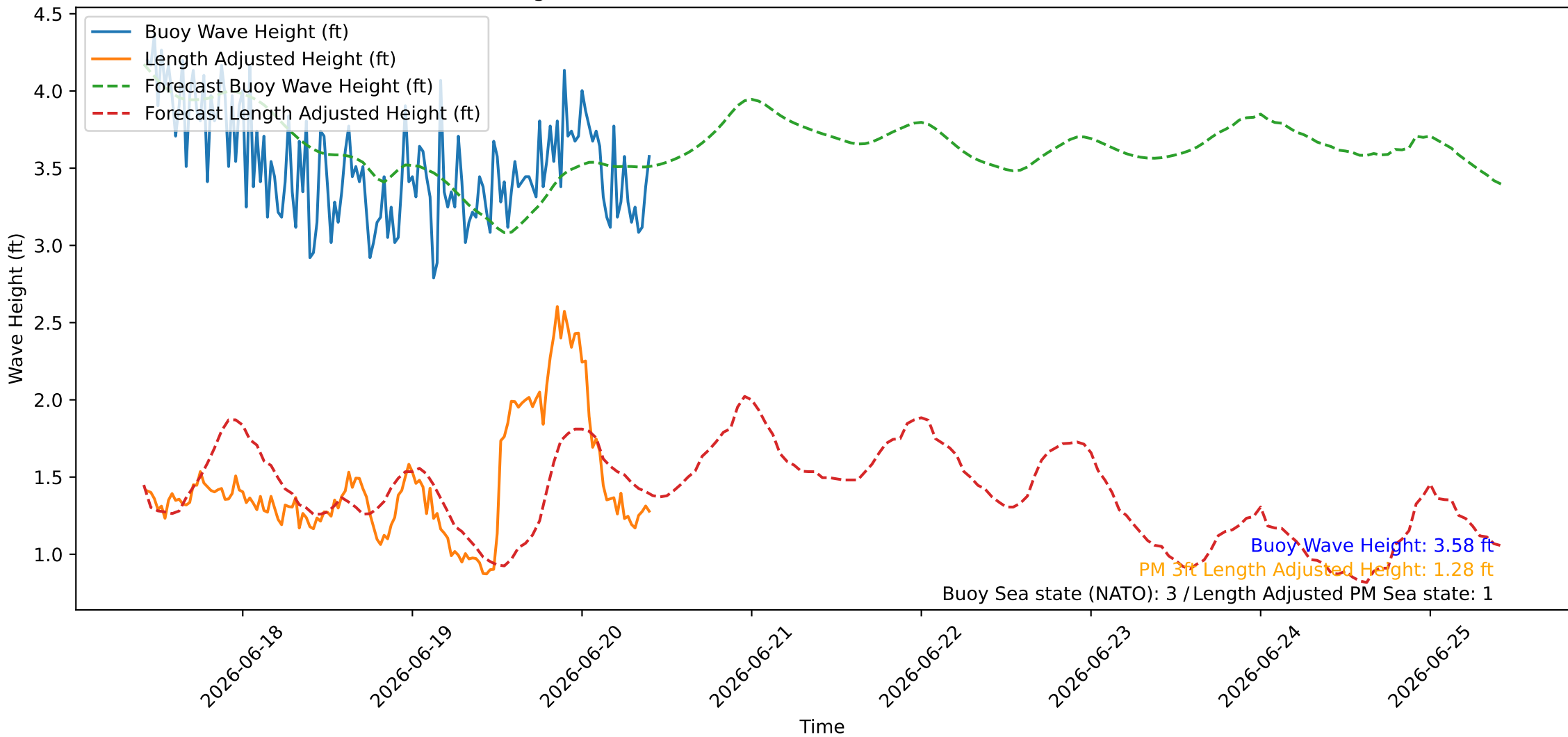
Wave Heights over Time for Oceanside Harbor at 2026-06-20 10:20:26
