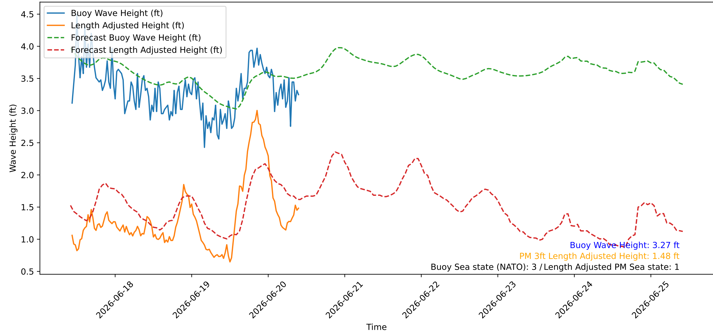
Wave Heights over Time for Green Beach at 2026-06-20 10:21:09
