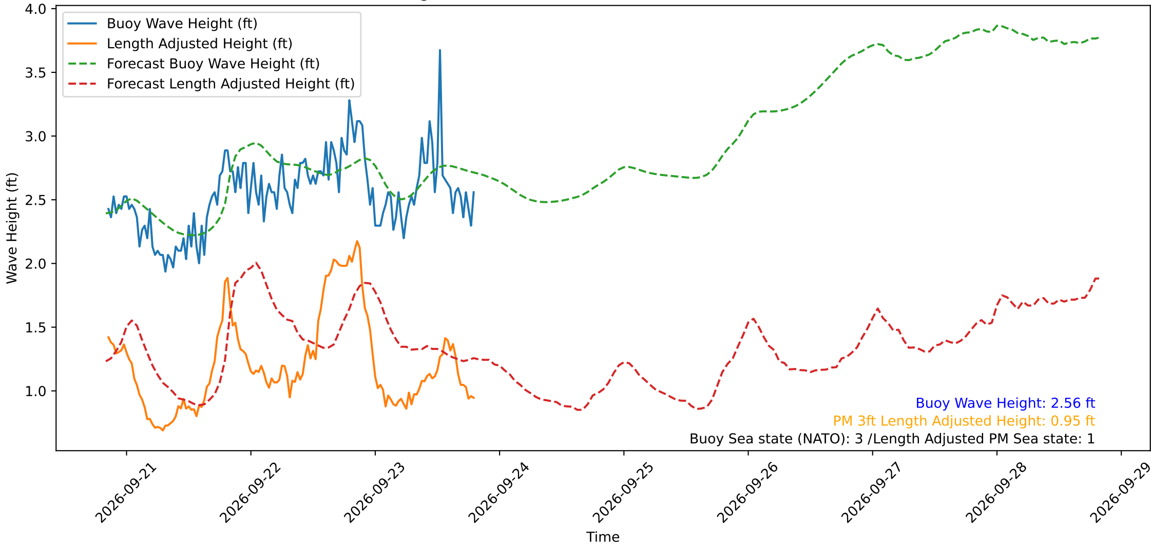
Wave Heights over Time for Red Beach at 2026-09-23 20:00:49
