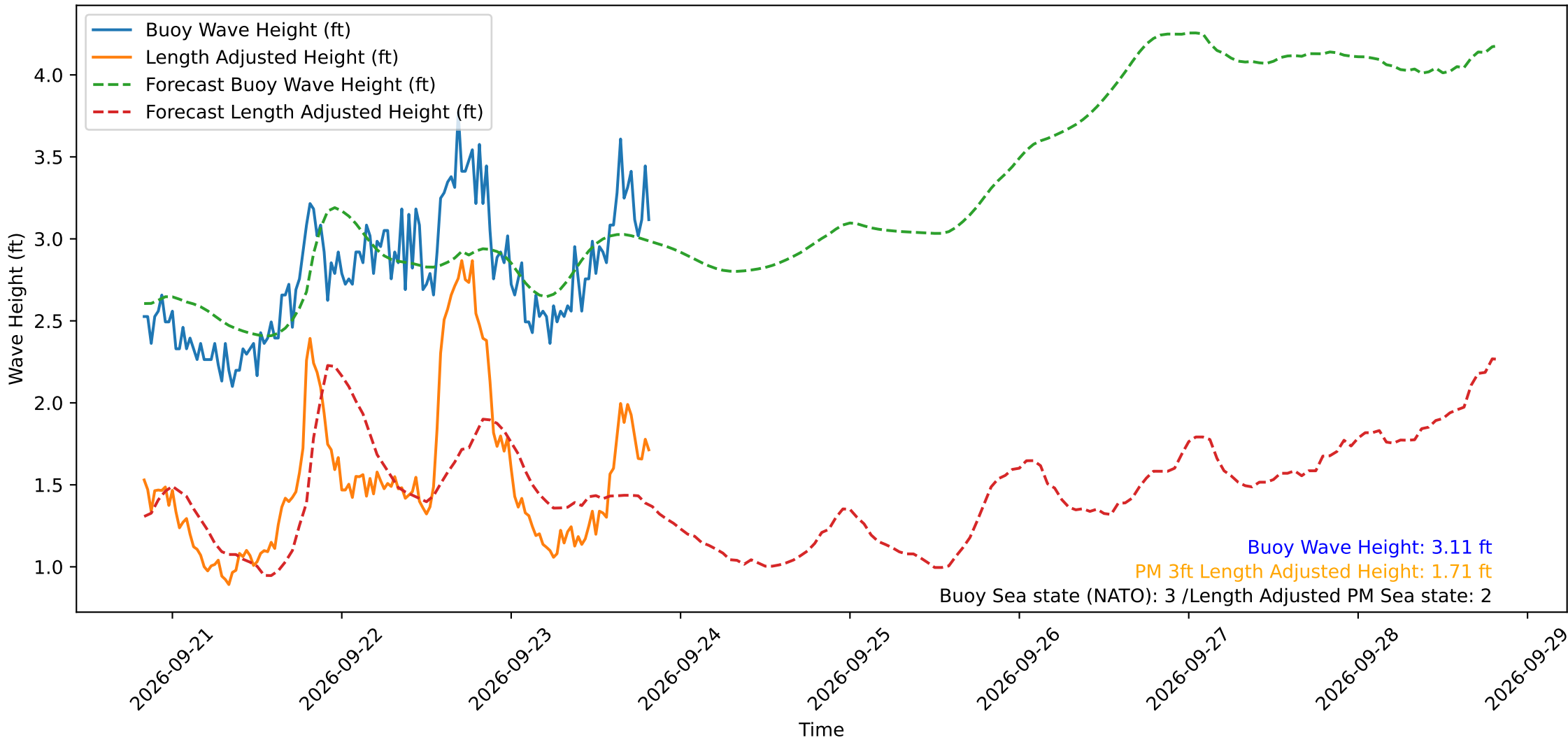
Wave Heights over Time for Oceanside Harbor at 2026-09-23 20:00:29
