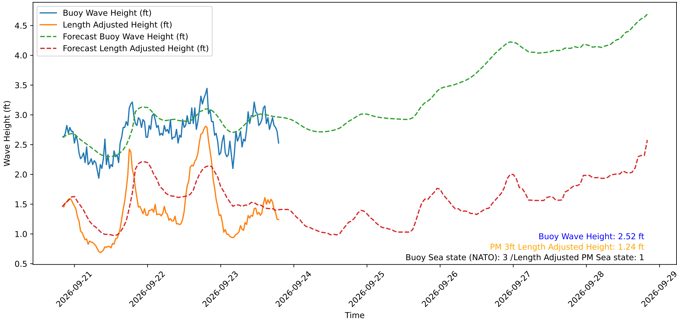
Wave Heights over Time for Green Beach at 2026-09-23 20:01:11
