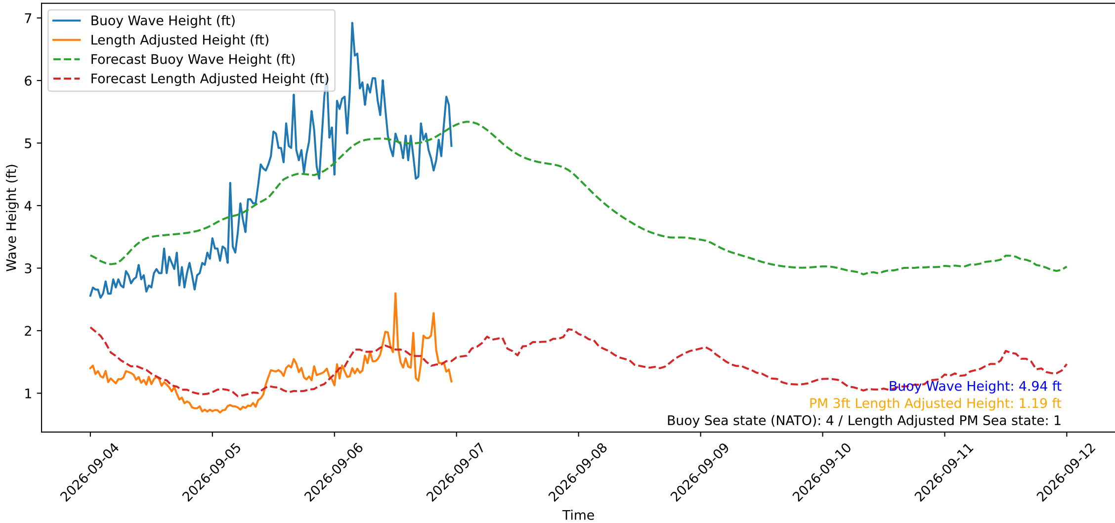
Wave Heights over Time for Red Beach at 2026-09-06 23:40:49
