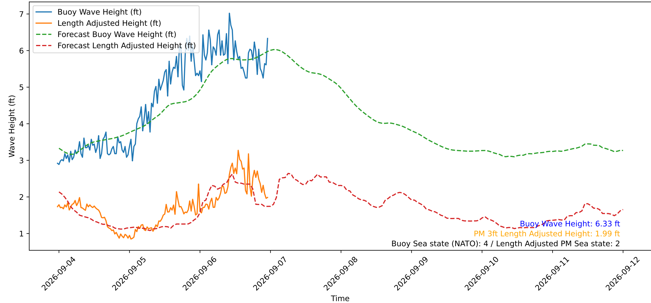
Wave Heights over Time for Oceanside Harbor at 2026-09-06 23:40:29
