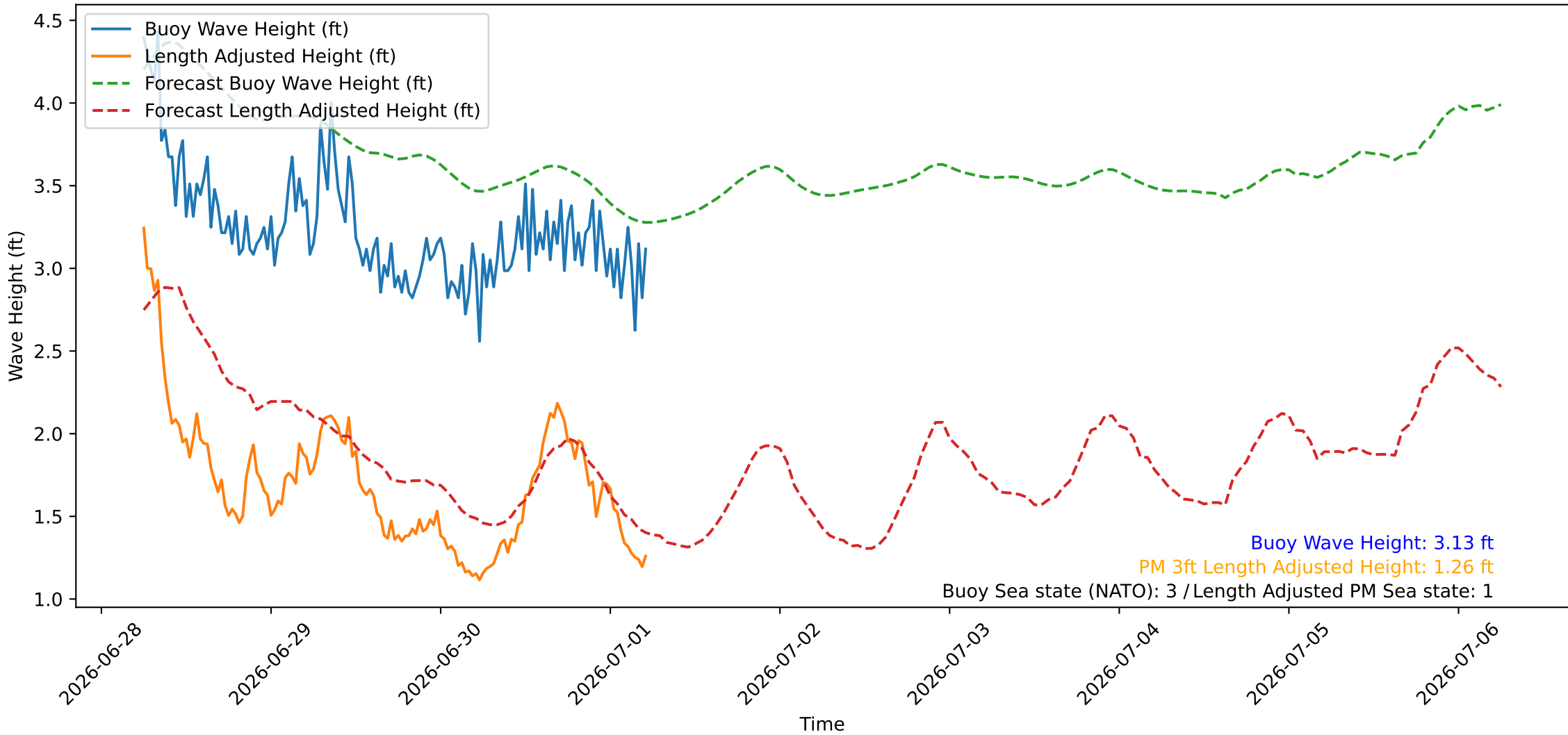
Wave Heights over Time for Oceanside Harbor at 2026-07-01 06:00:26
