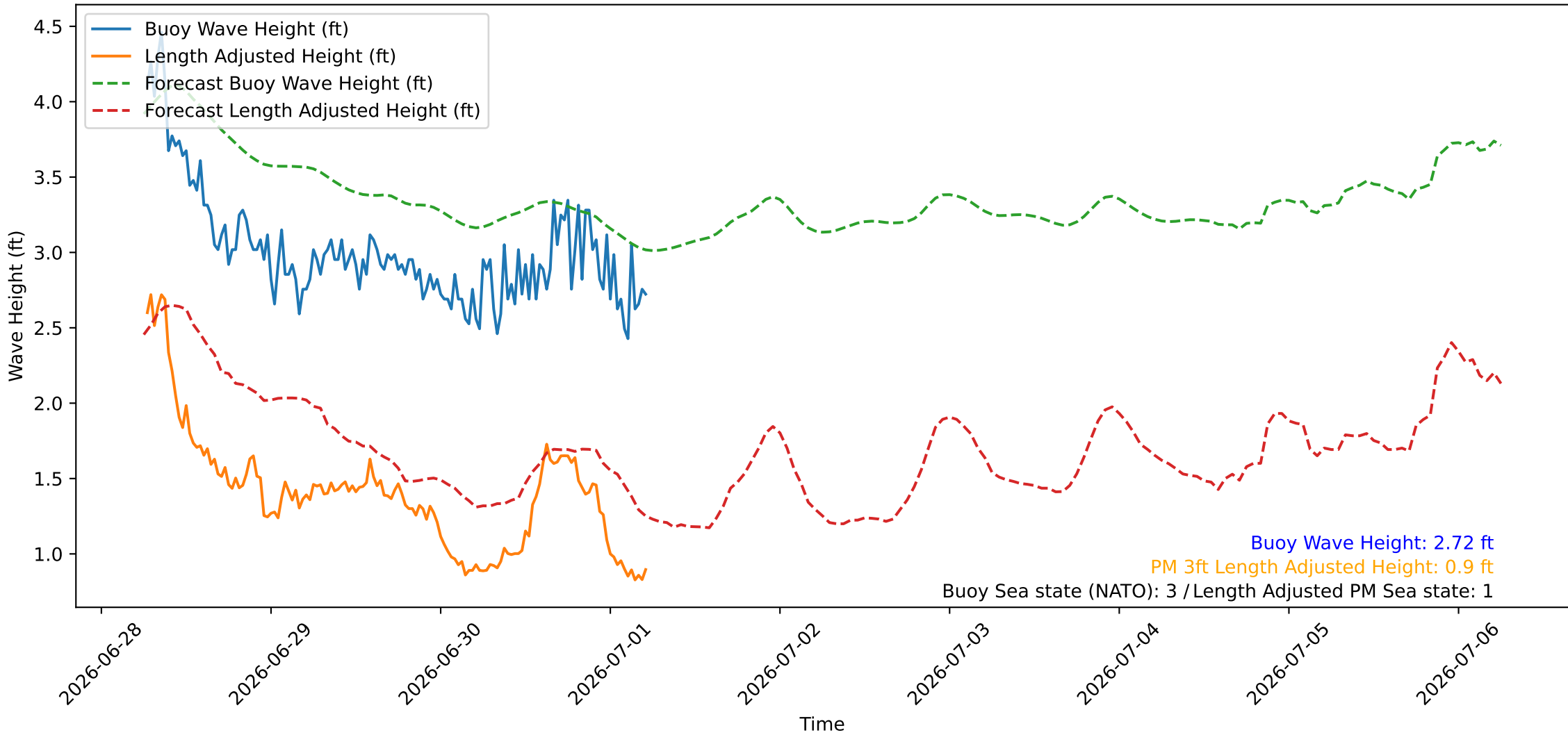
Wave Heights over Time for Red Beach at 2026-07-01 06:00:46
