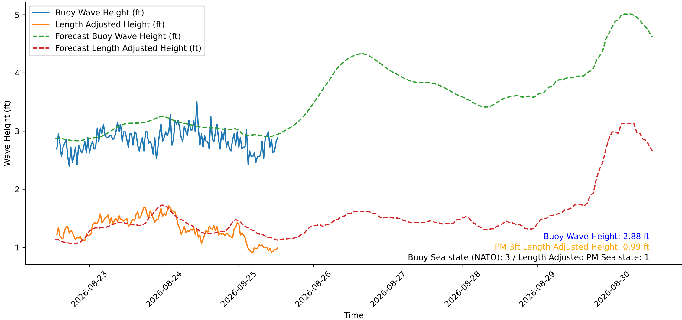
Wave Heights over Time for Oceanside Harbor at 2026-08-25 13:20:30
