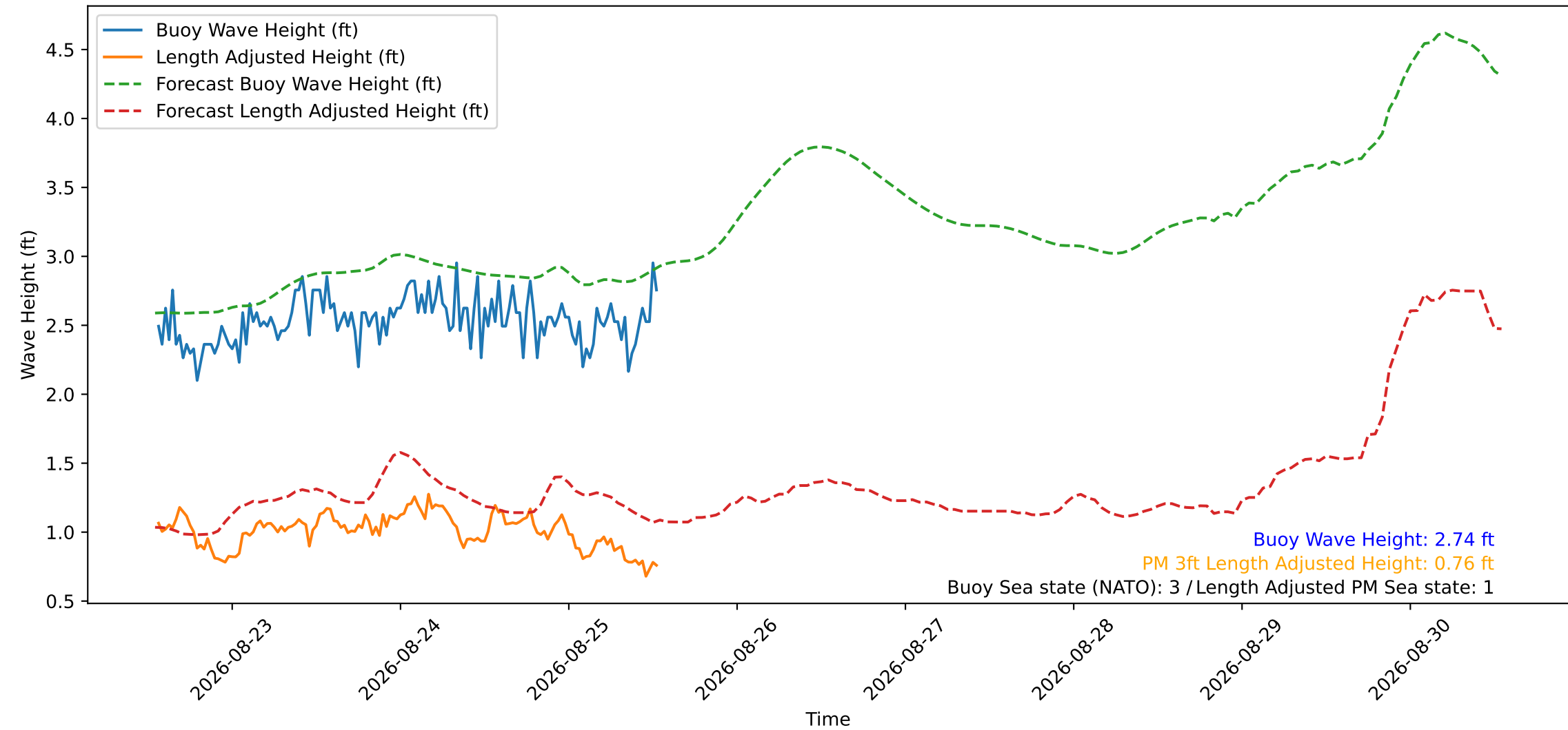
Wave Heights over Time for Red Beach at 2026-08-25 13:20:51
