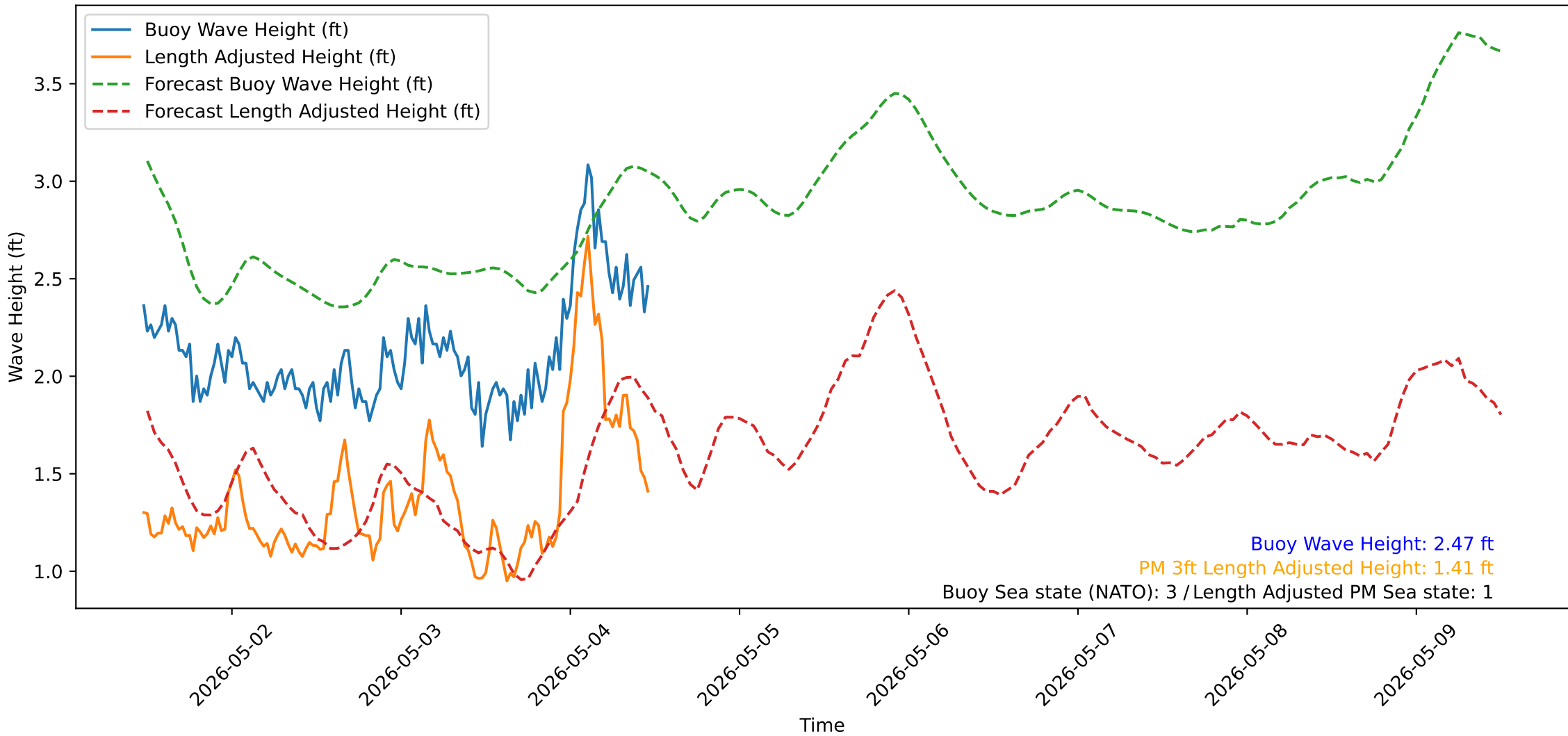
Wave Heights over Time for Oceanside Harbor at 2026-05-04 11:40:32
