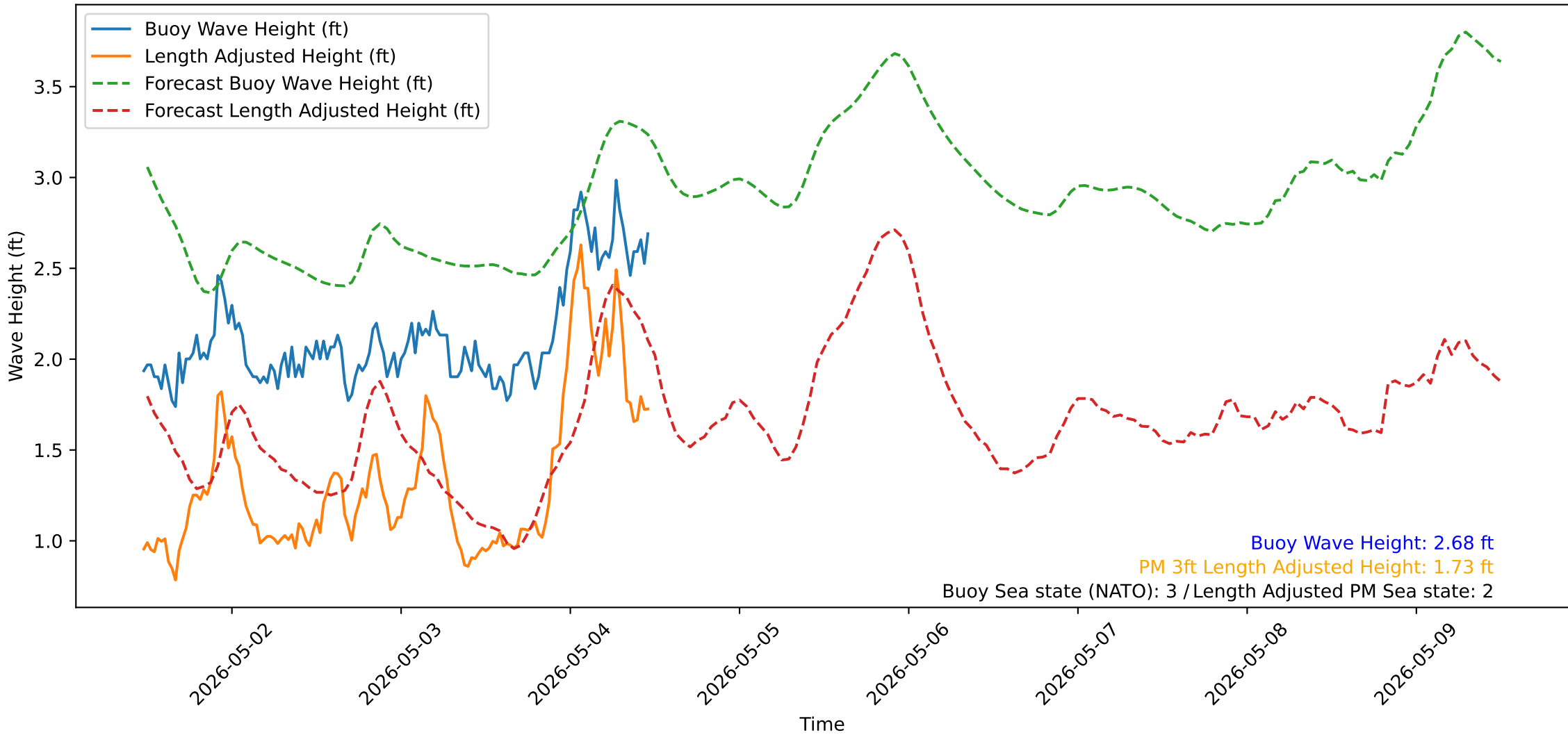
Wave Heights over Time for Green Beach at 2026-05-04 11:41:13
