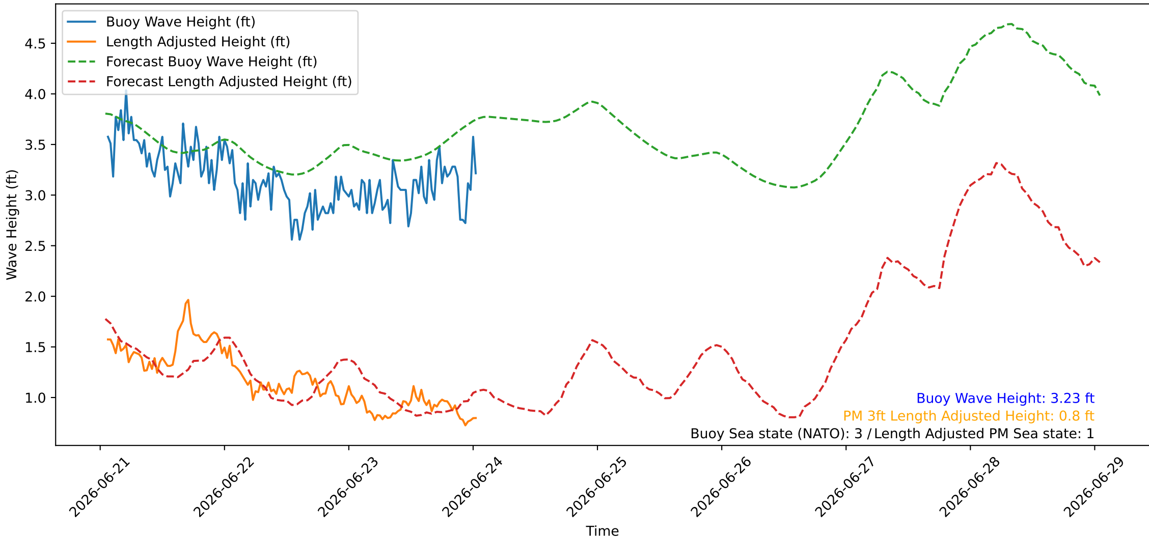
Wave Heights over Time for Oceanside Harbor at 2026-06-24 01:20:25
