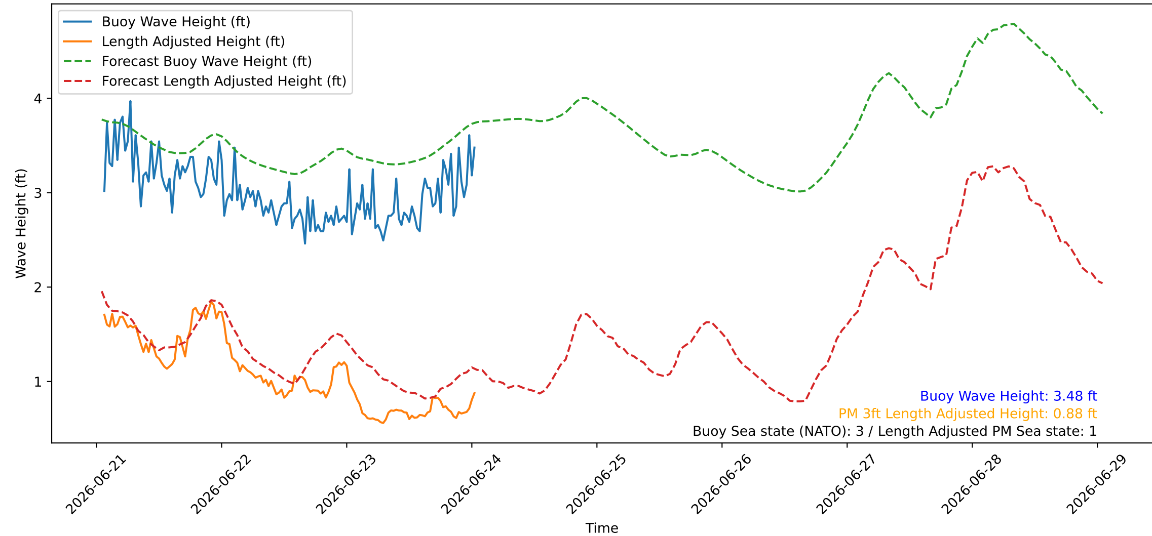
Wave Heights over Time for Green Beach at 2026-06-24 01:21:08
