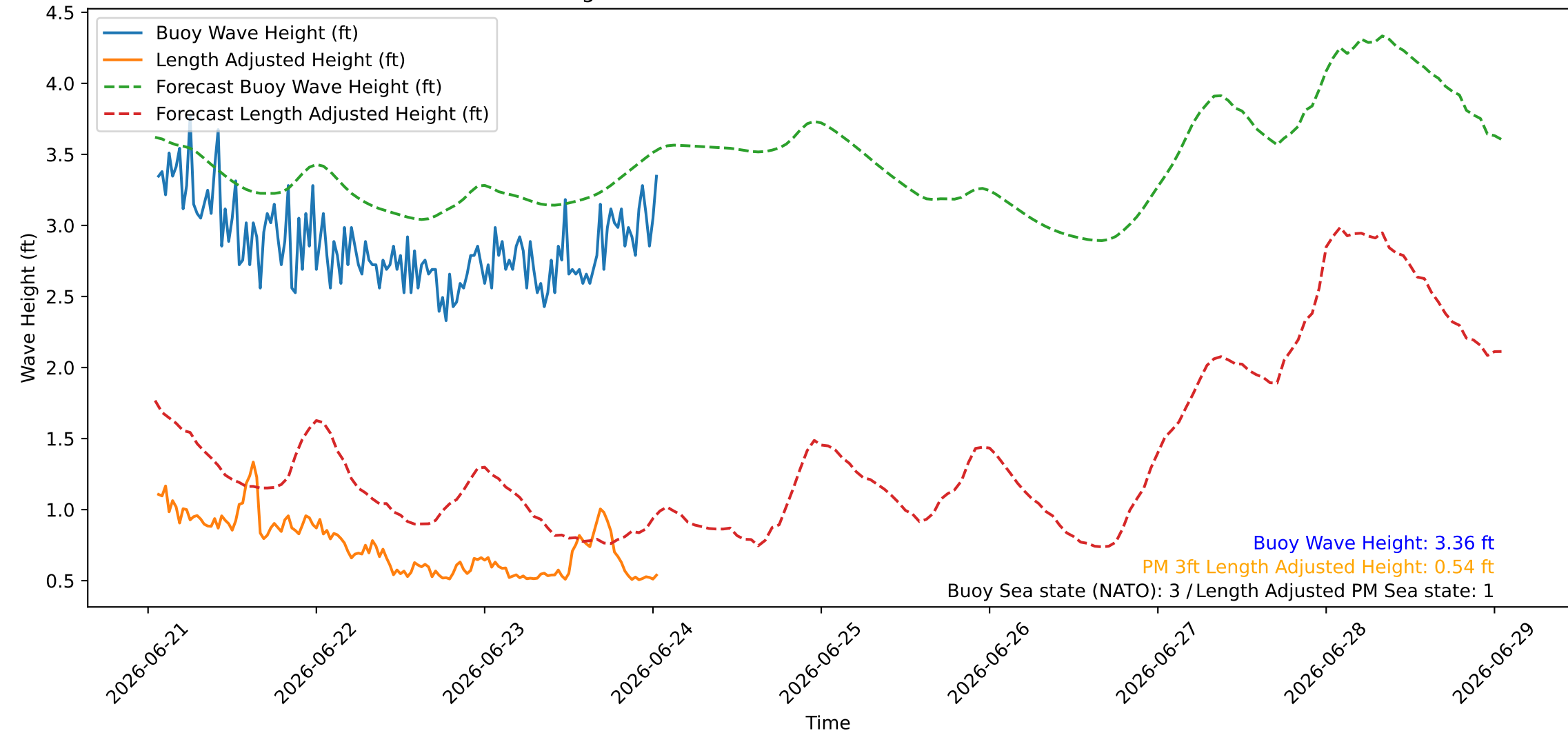
Wave Heights over Time for Red Beach at 2026-06-24 01:20:46
