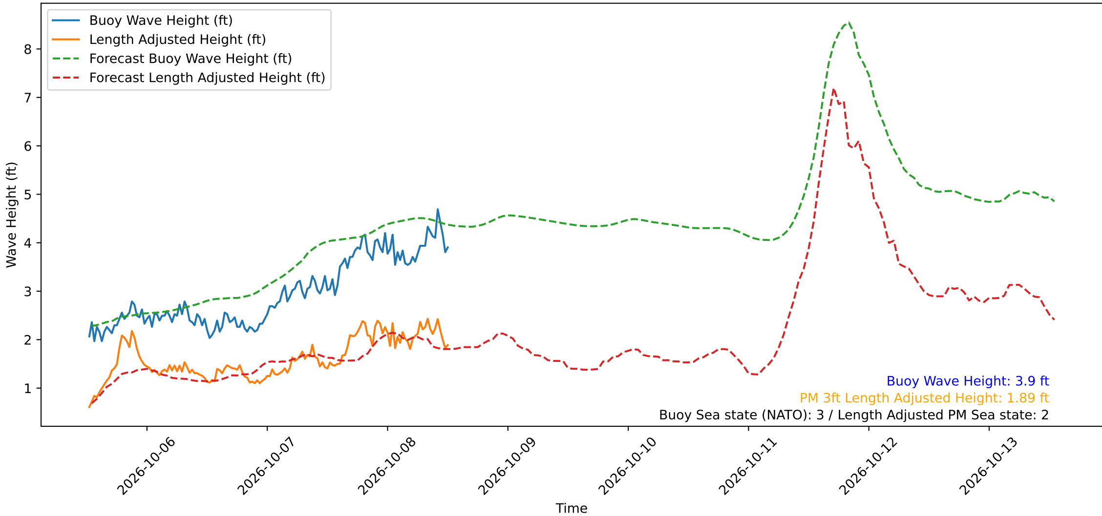
Wave Heights over Time for Oceanside Harbor at 2026-10-08 12:30:30
