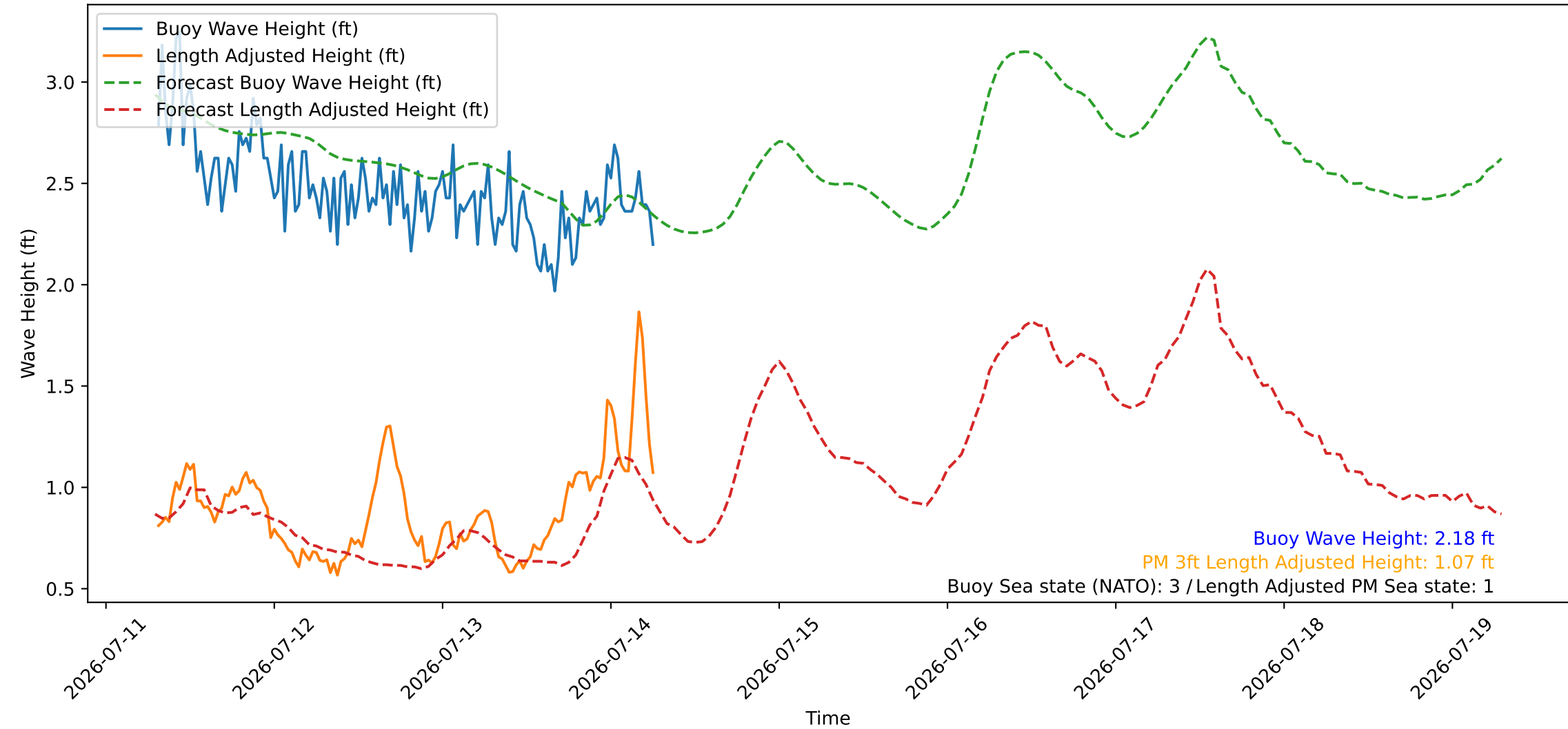
Wave Heights over Time for Red Beach at 2026-07-14 07:10:46
