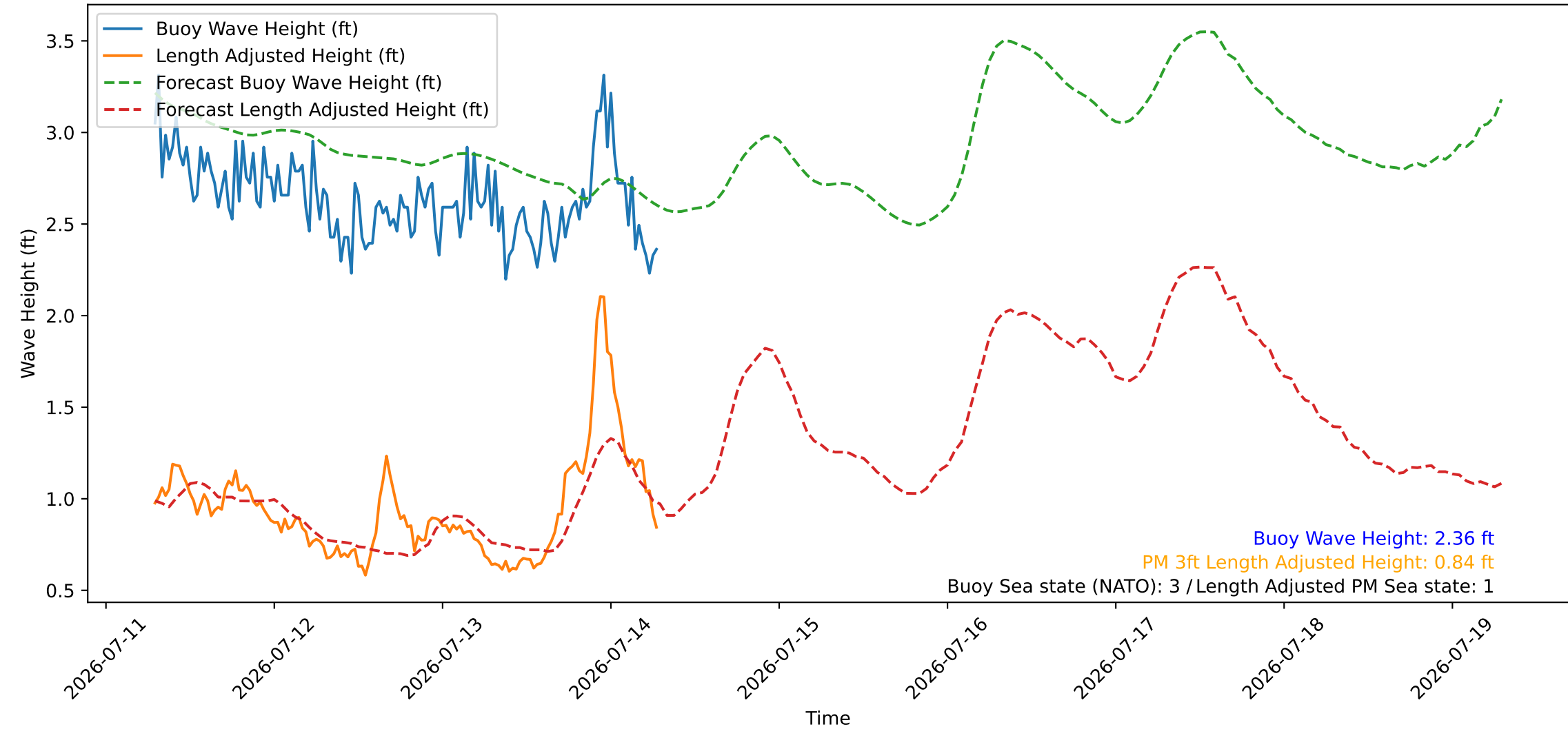
Wave Heights over Time for Green Beach at 2026-07-14 07:11:09
