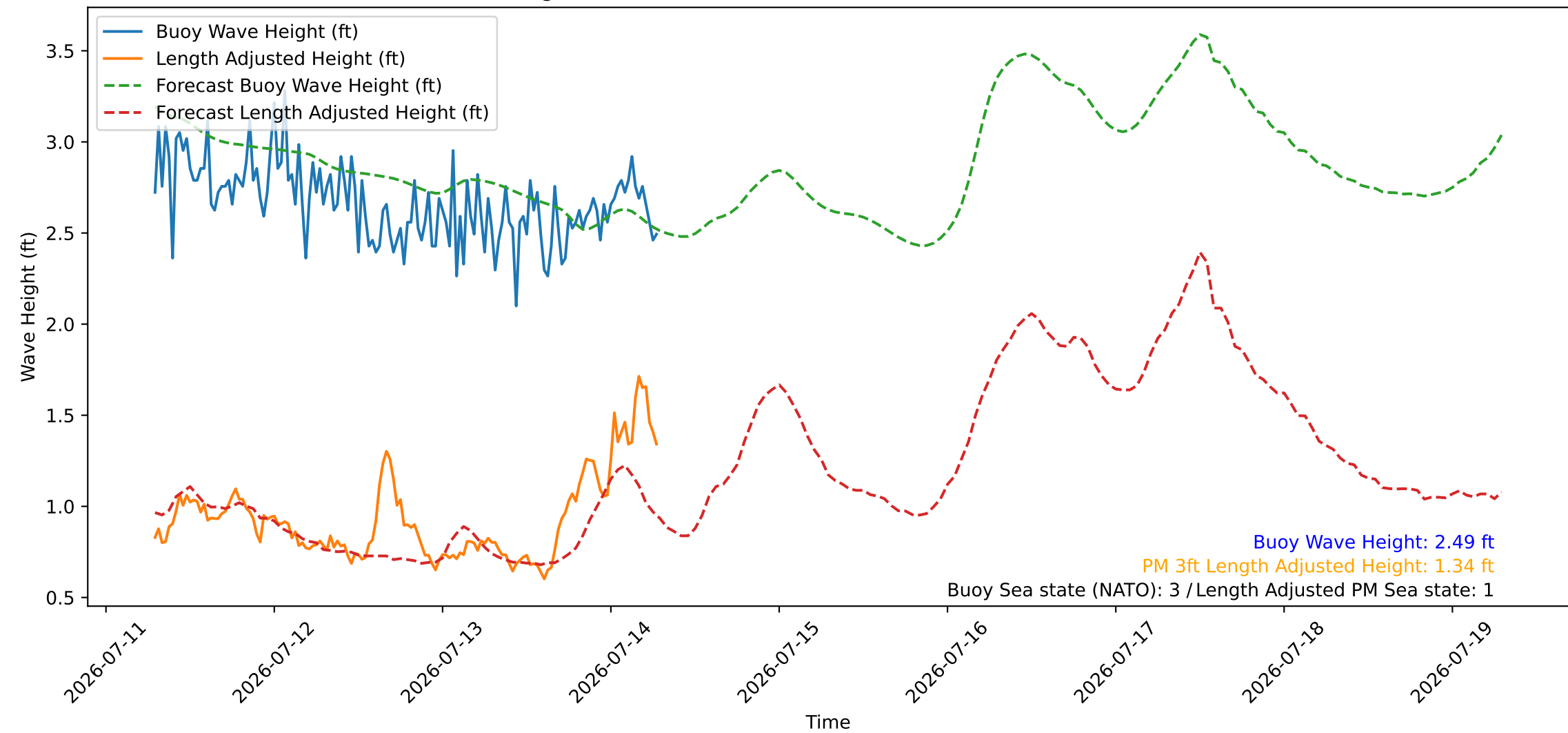
Wave Heights over Time for Oceanside Harbor at 2026-07-14 07:10:27
