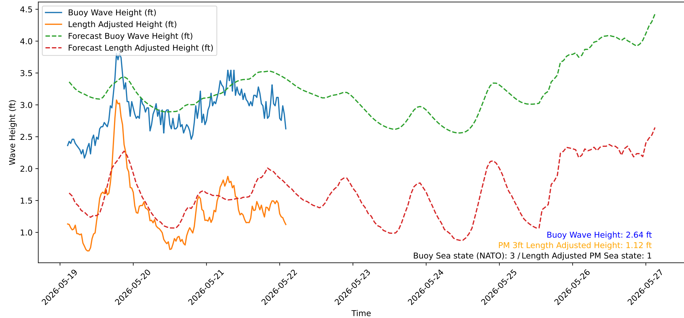
Wave Heights over Time for Green Beach at 2026-05-22 02:41:13
