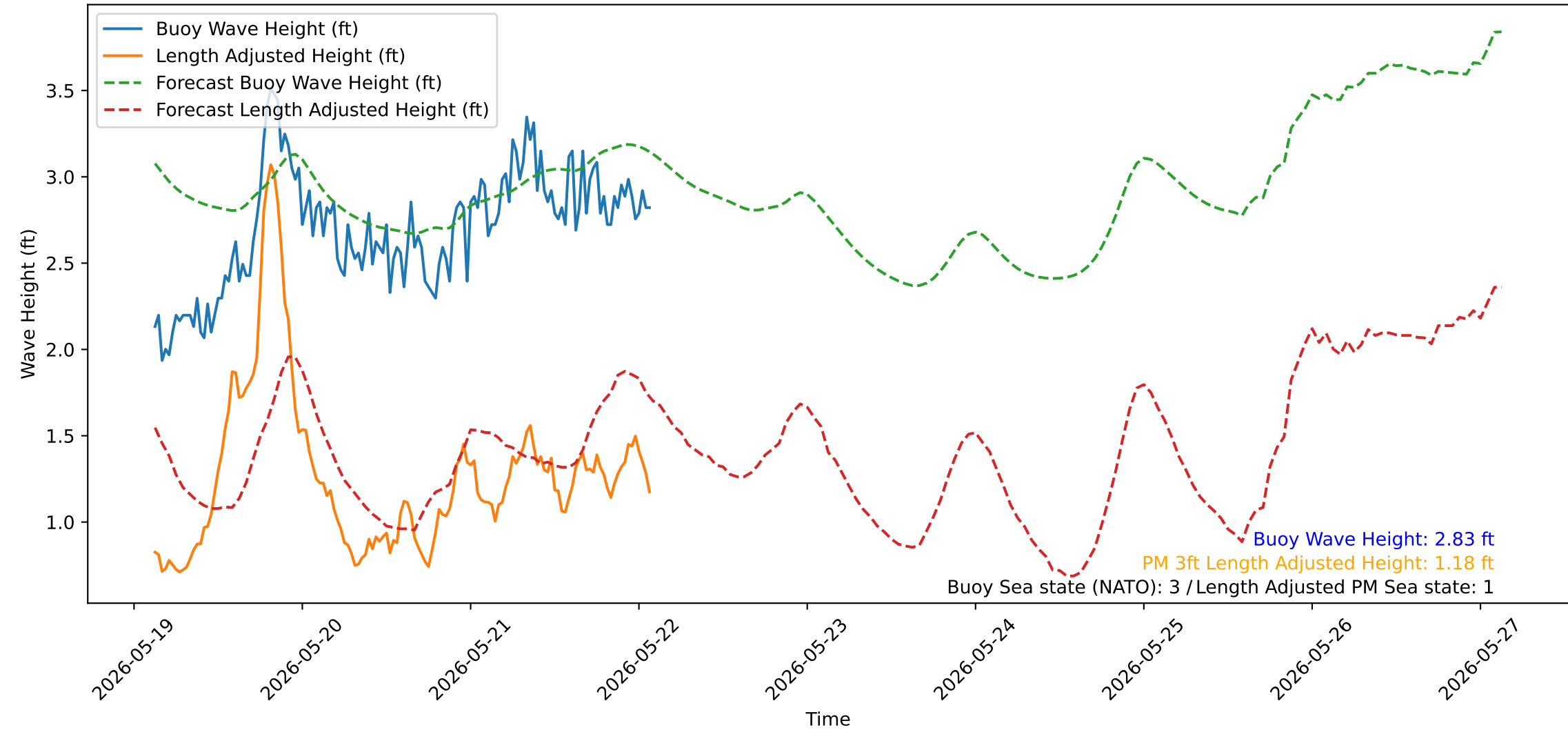
Wave Heights over Time for Red Beach at 2026-05-22 02:40:51
