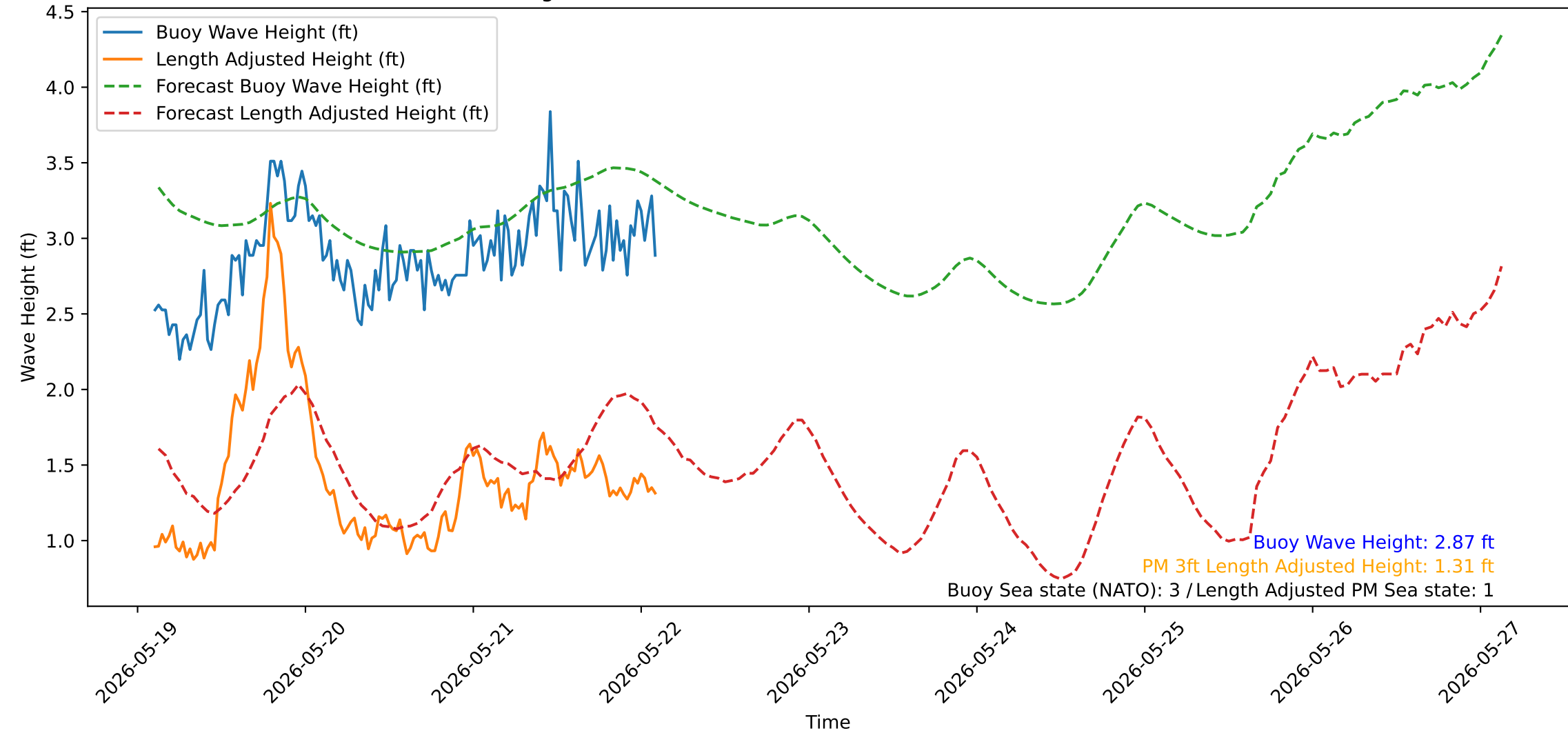
Wave Heights over Time for Oceanside Harbor at 2026-05-22 02:40:31
