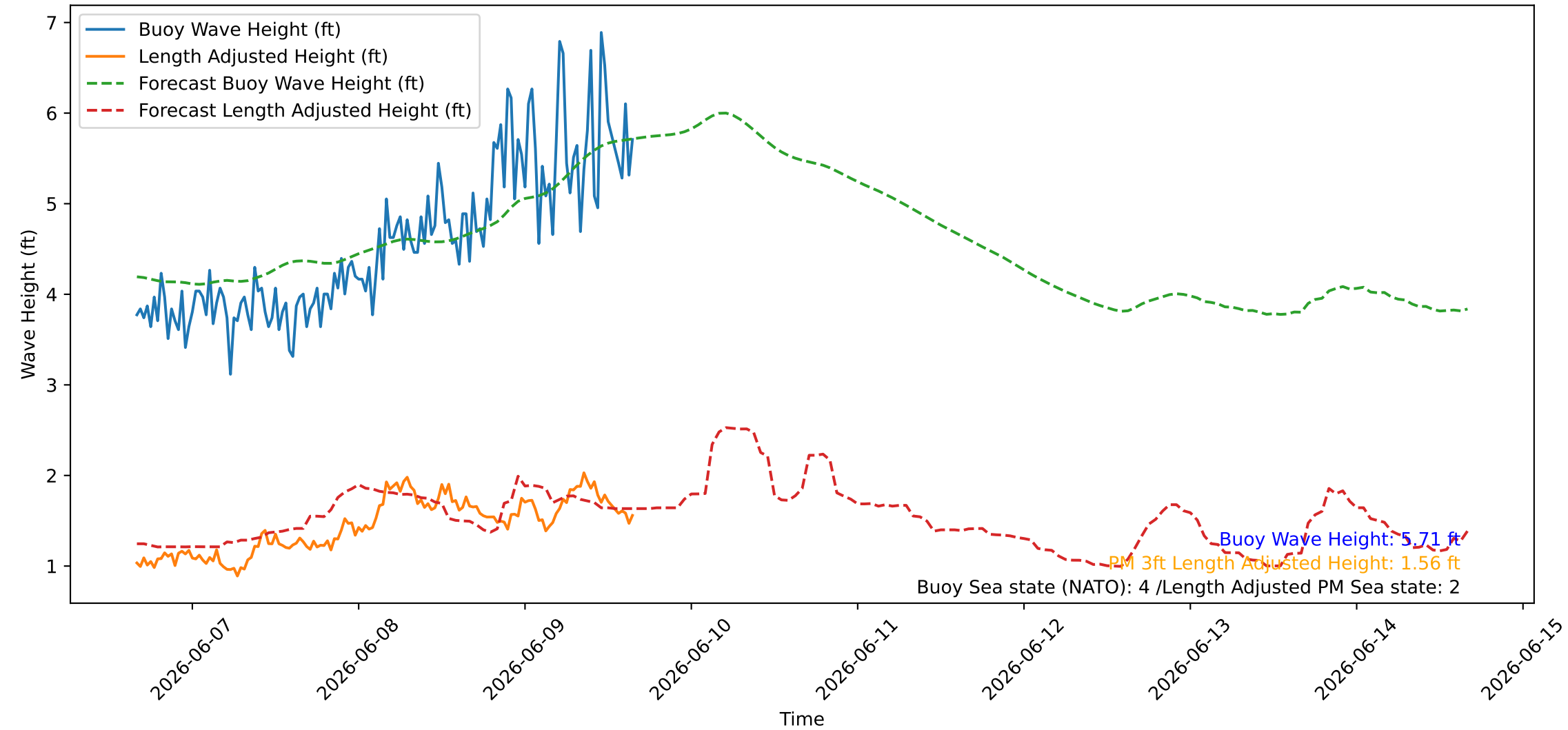
Wave Heights over Time for Green Beach at 2026-06-09 16:11:07
