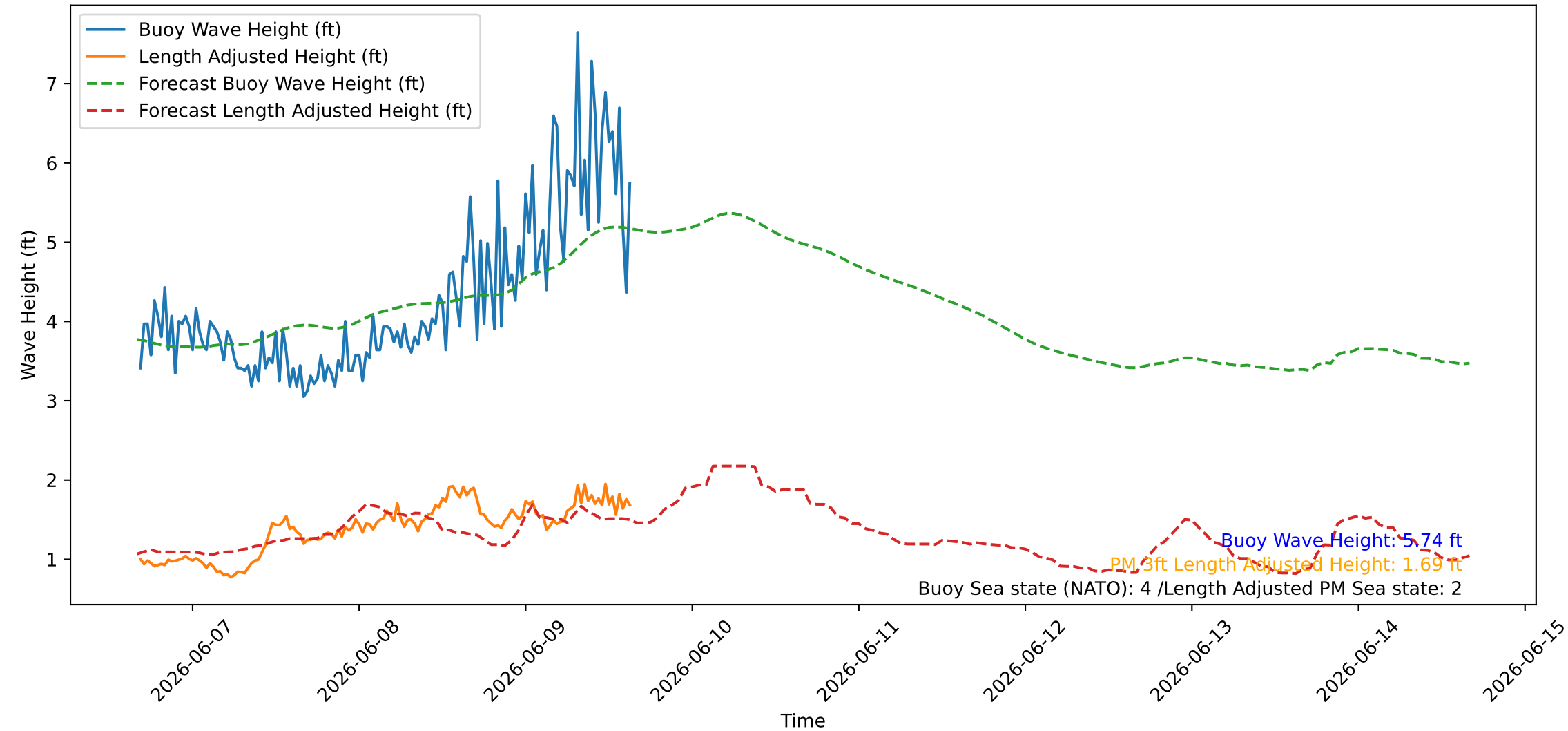
Wave Heights over Time for Red Beach at 2026-06-09 16:10:45
