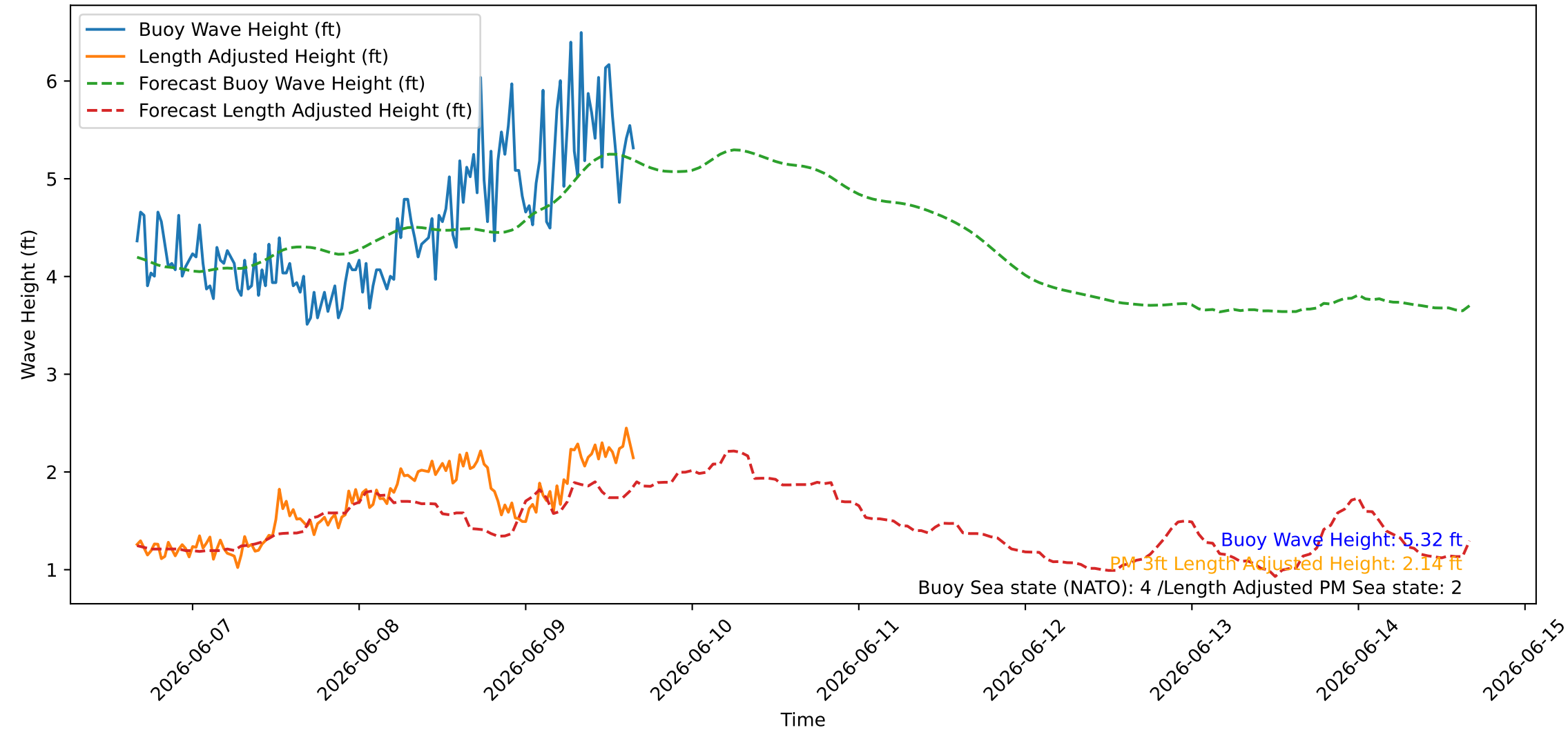
Wave Heights over Time for Oceanside Harbor at 2026-06-09 16:10:26
