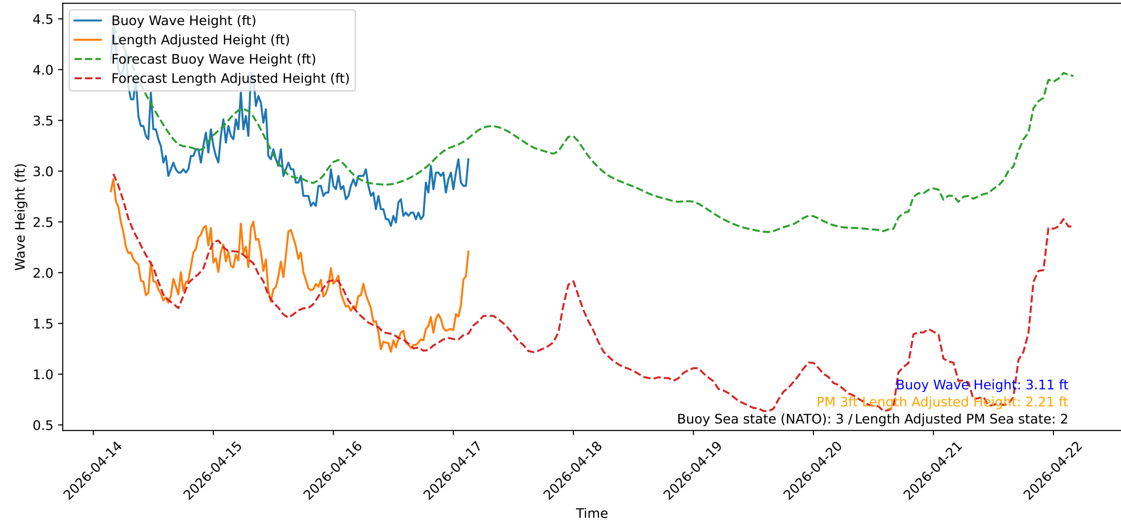
Wave Heights over Time for Green Beach at 2026-04-17 03:41:15
