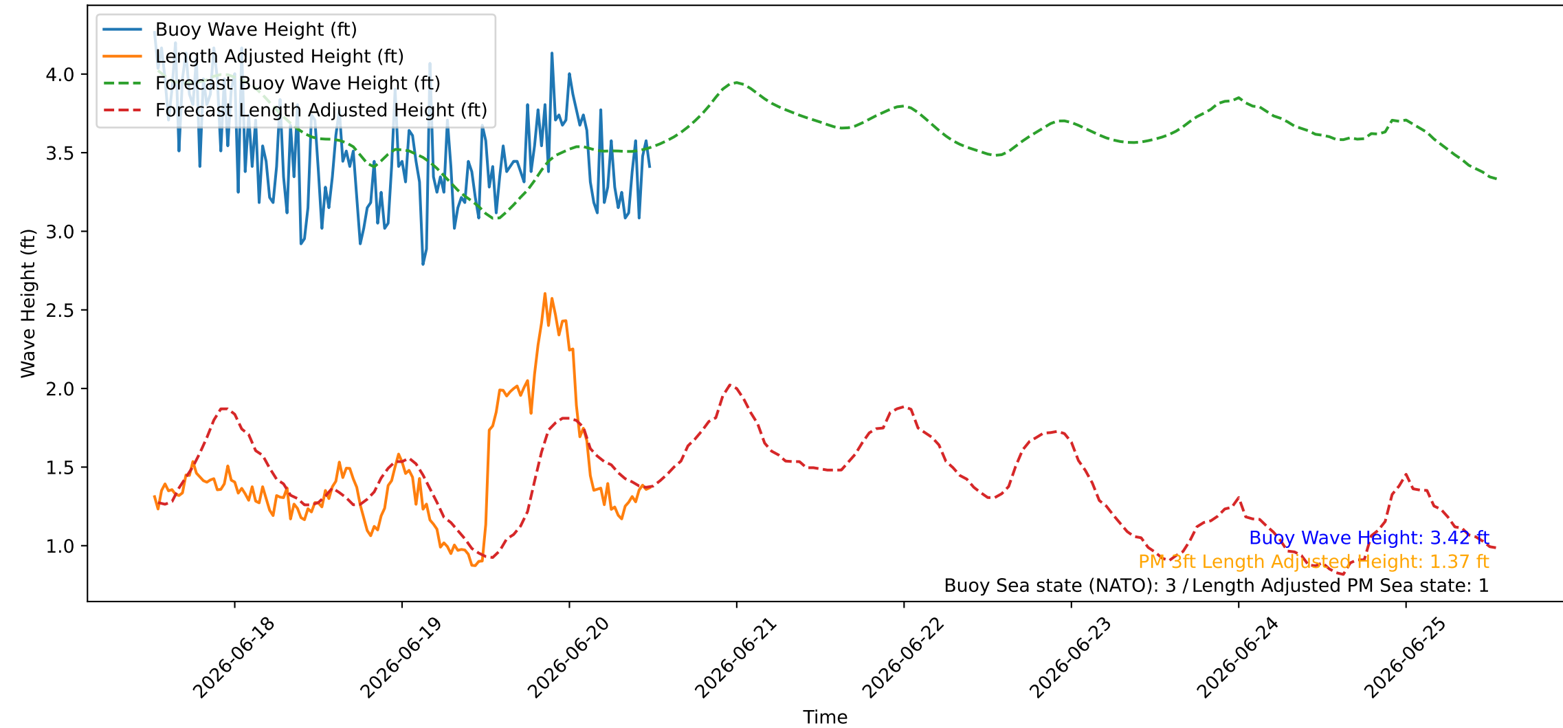
Wave Heights over Time for Oceanside Harbor at 2026-06-20 12:30:26
