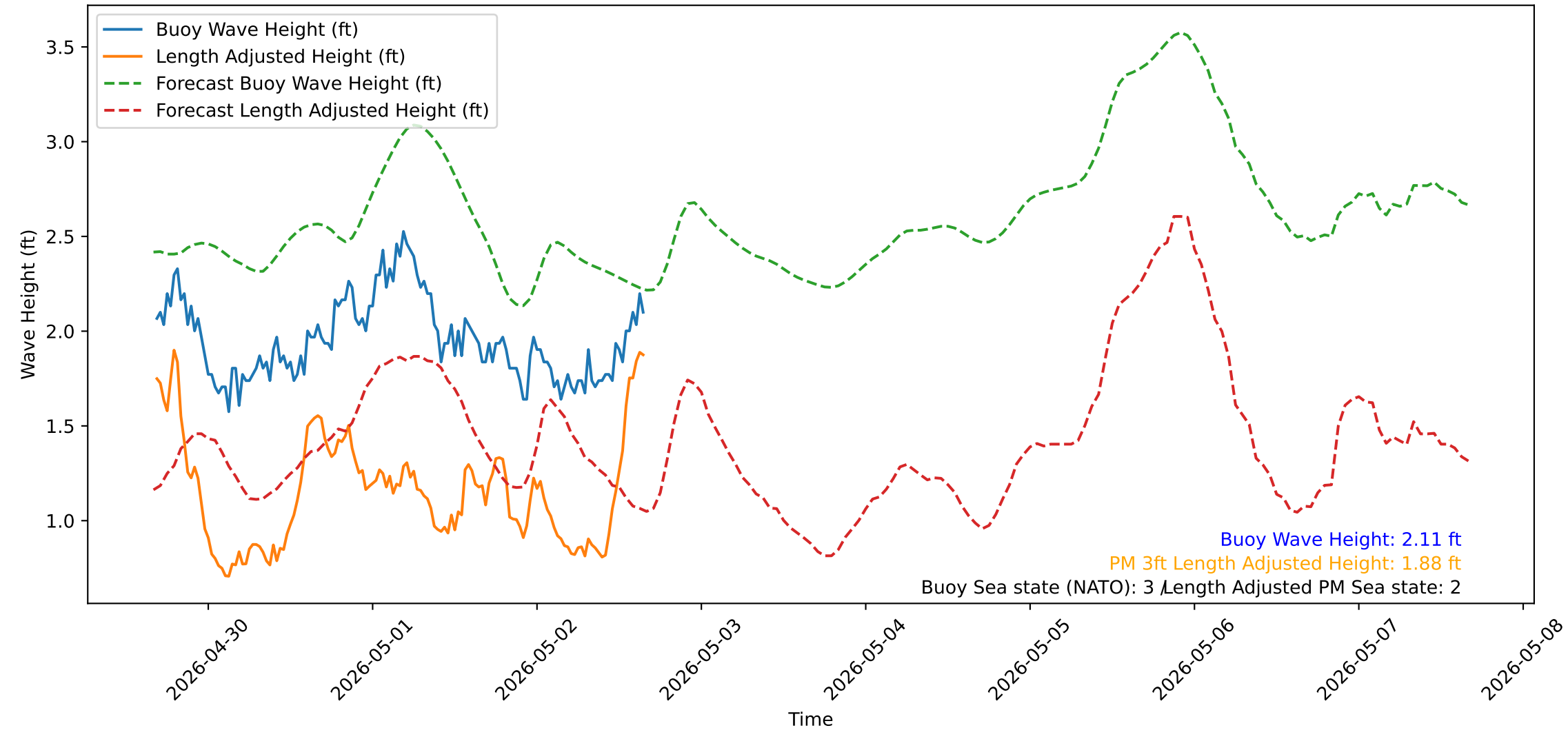
Wave Heights over Time for Red Beach at 2026-05-02 16:20:51
