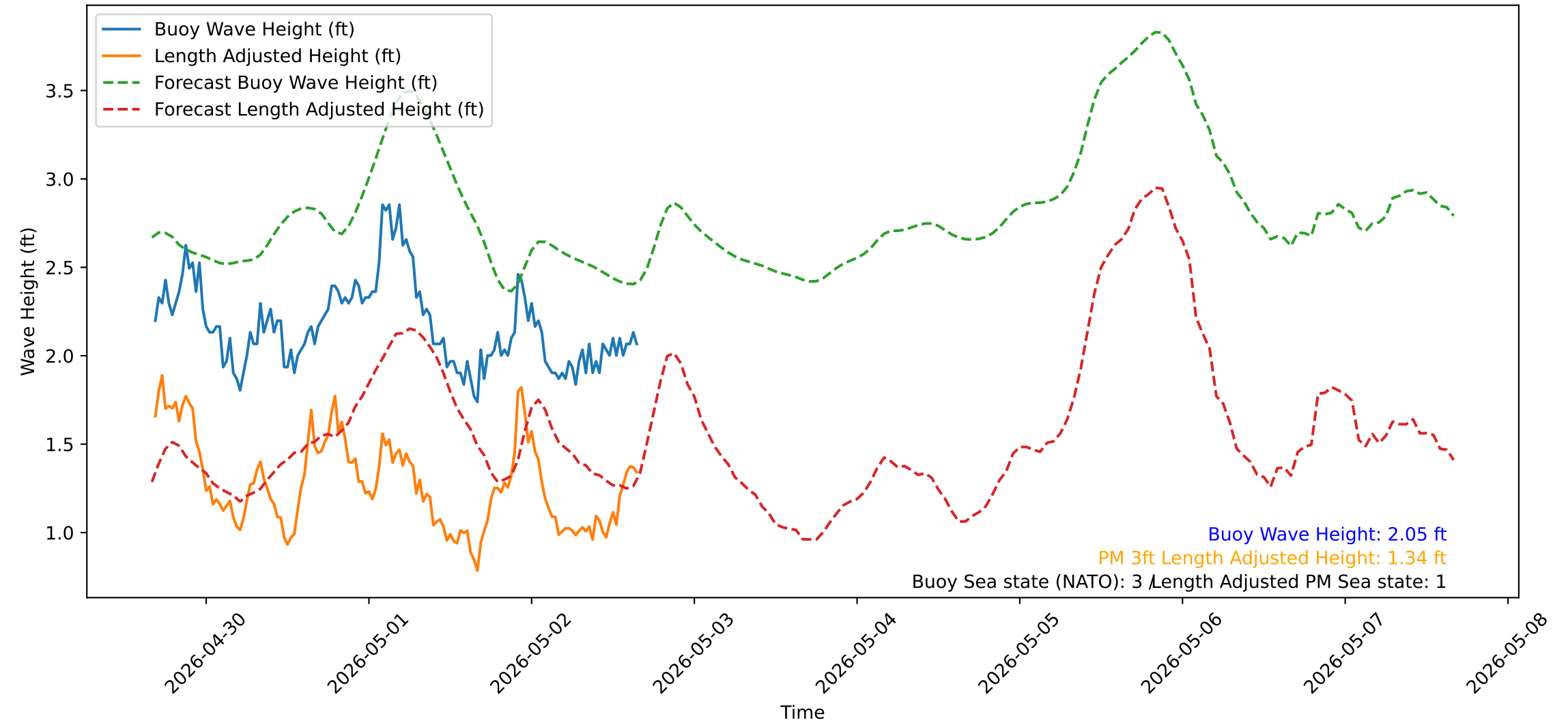
Wave Heights over Time for Green Beach at 2026-05-02 16:21:14
