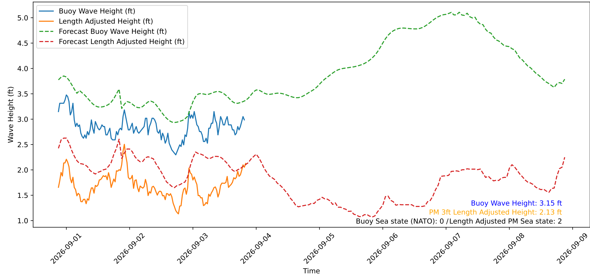
Wave Heights over Time for Red Beach at 2026-09-03 20:50:51
