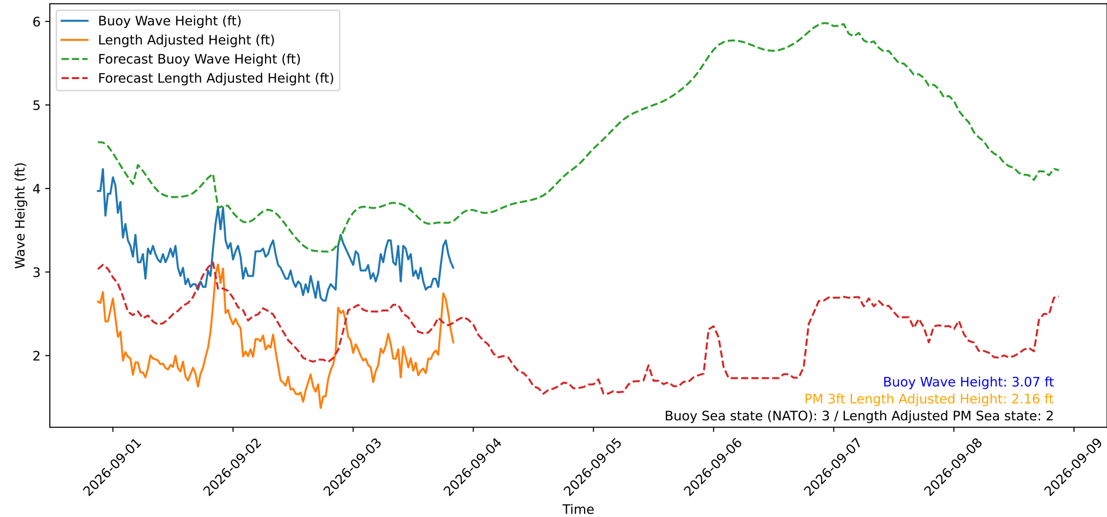
Wave Heights over Time for Green Beach at 2026-09-03 20:51:15
