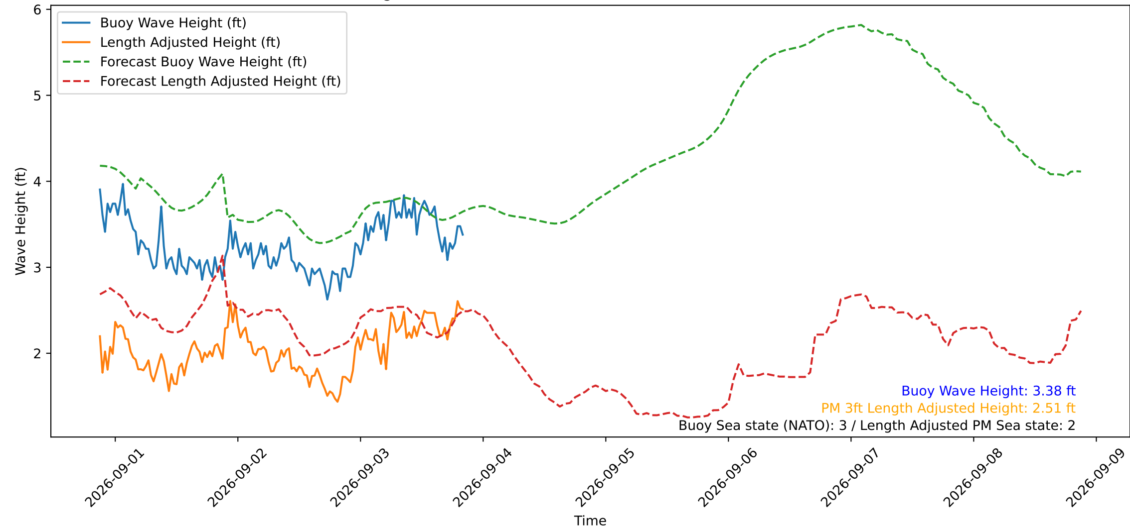
Wave Heights over Time for Oceanside Harbor at 2026-09-03 20:50:30
