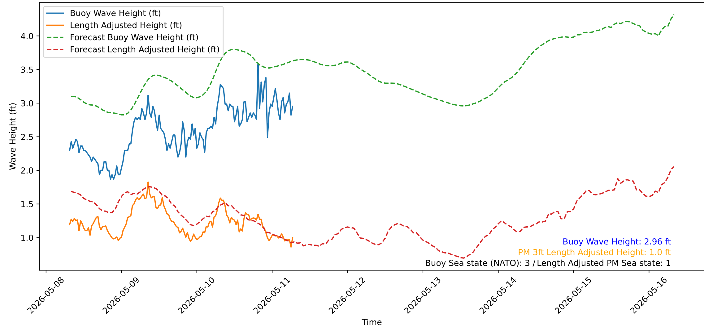
Wave Heights over Time for Oceanside Harbor at 2026-05-11 07:30:31
