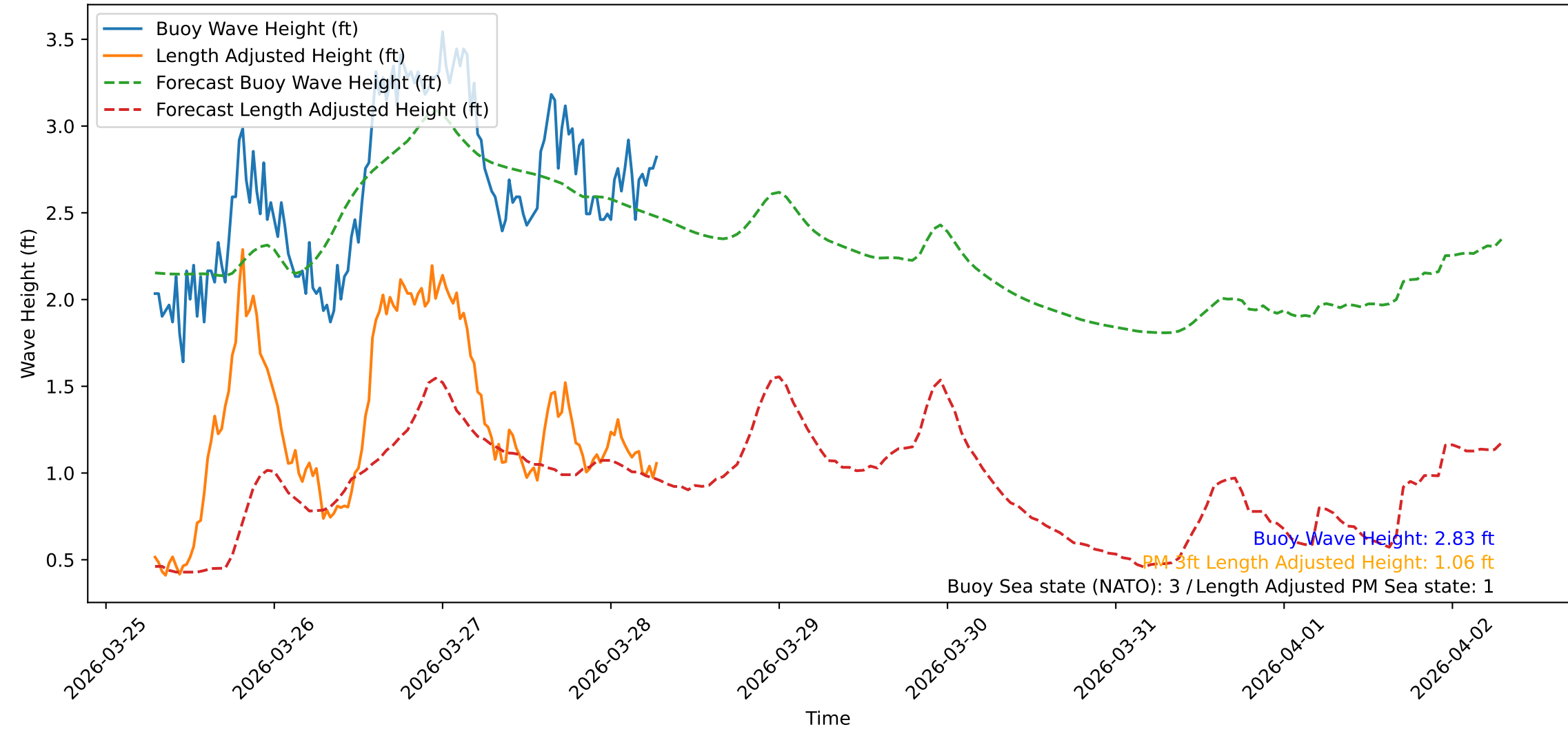
Wave Heights over Time for Green Beach at 2026-03-28 07:11:09
