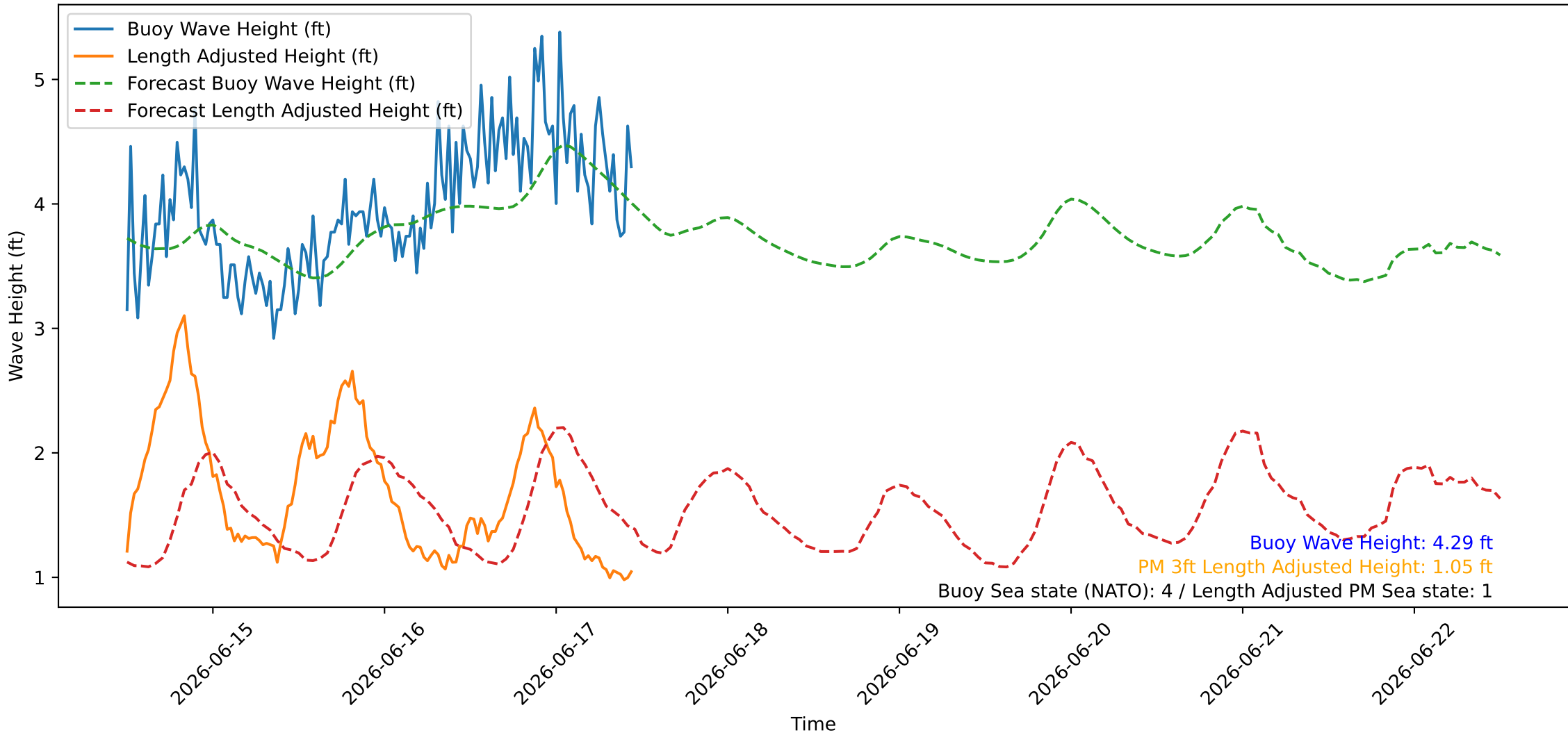
Wave Heights over Time for Red Beach at 2026-06-17 11:30:46
