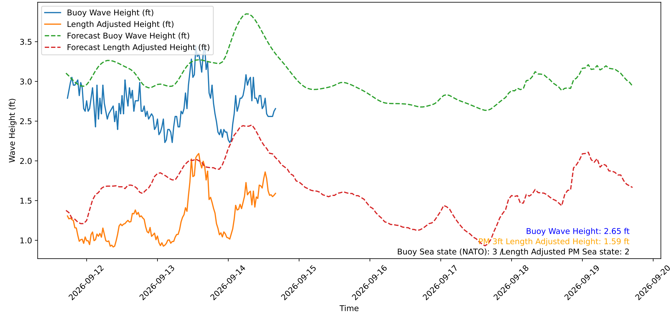
Wave Heights over Time for Red Beach at 2026-09-14 17:00:49
