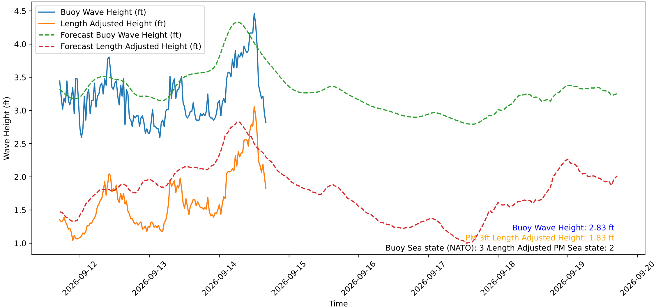
Wave Heights over Time for Oceanside Harbor at 2026-09-14 17:00:29
