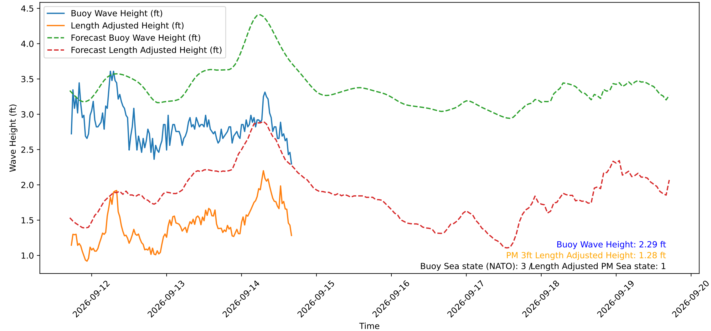
Wave Heights over Time for Green Beach at 2026-09-14 17:01:12
