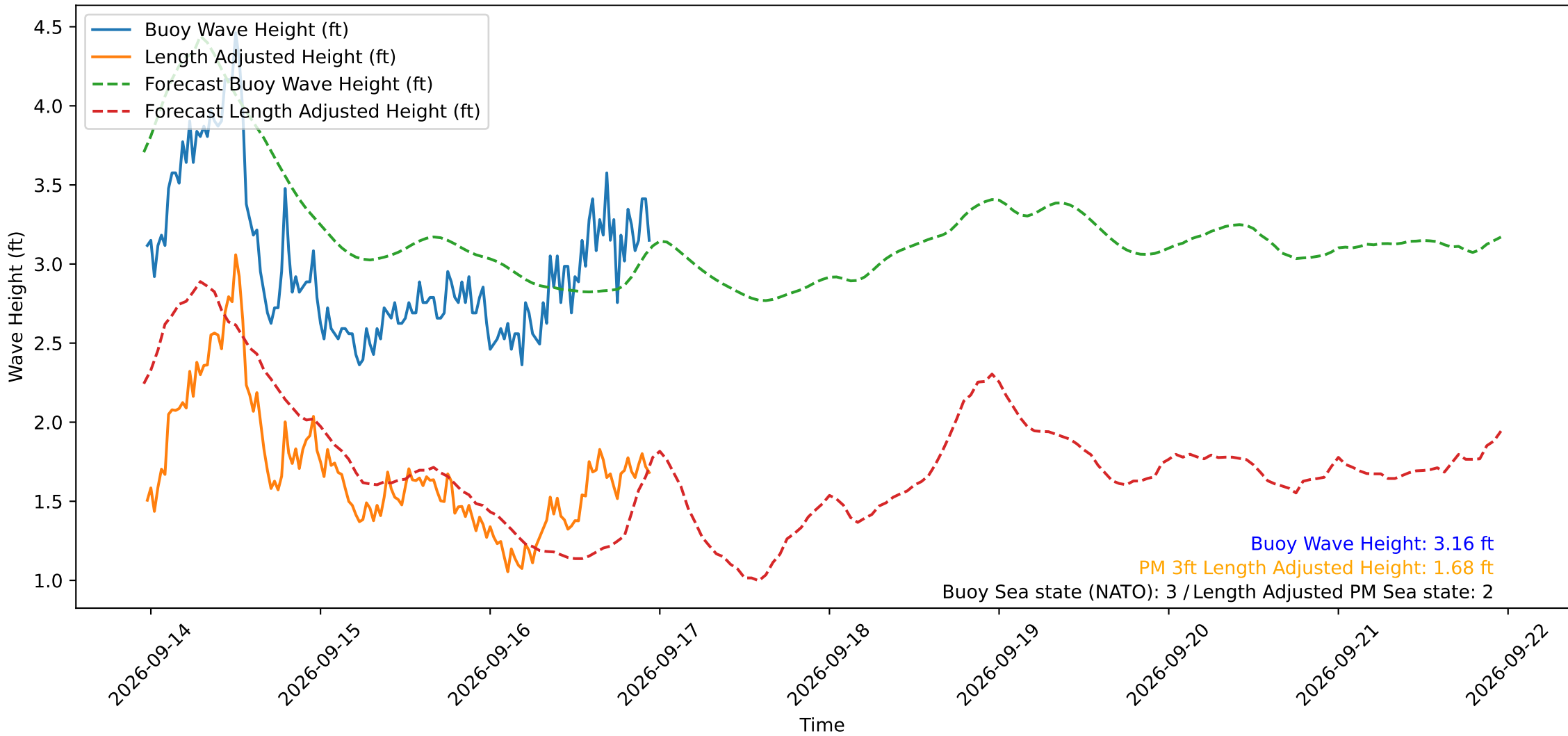
Wave Heights over Time for Oceanside Harbor at 2026-09-16 23:20:29
