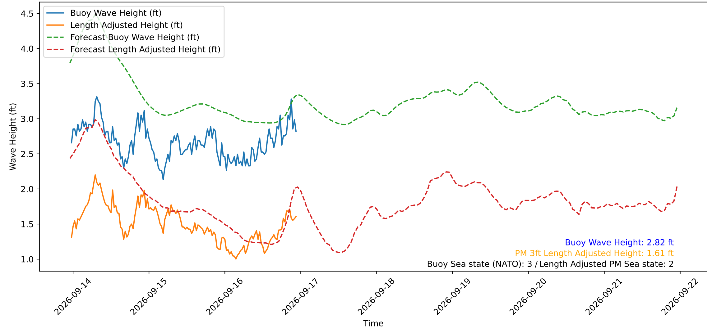
Wave Heights over Time for Green Beach at 2026-09-16 23:21:13
