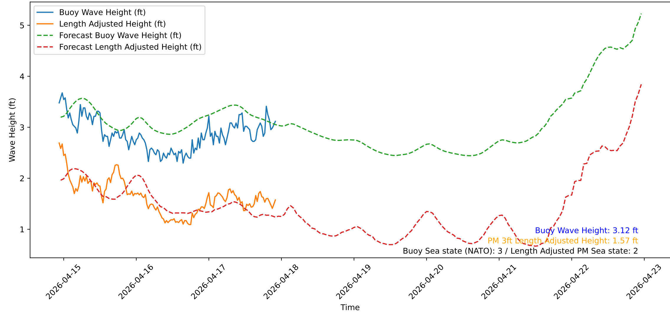
Wave Heights over Time for Oceanside Harbor at 2026-04-17 22:30:31
