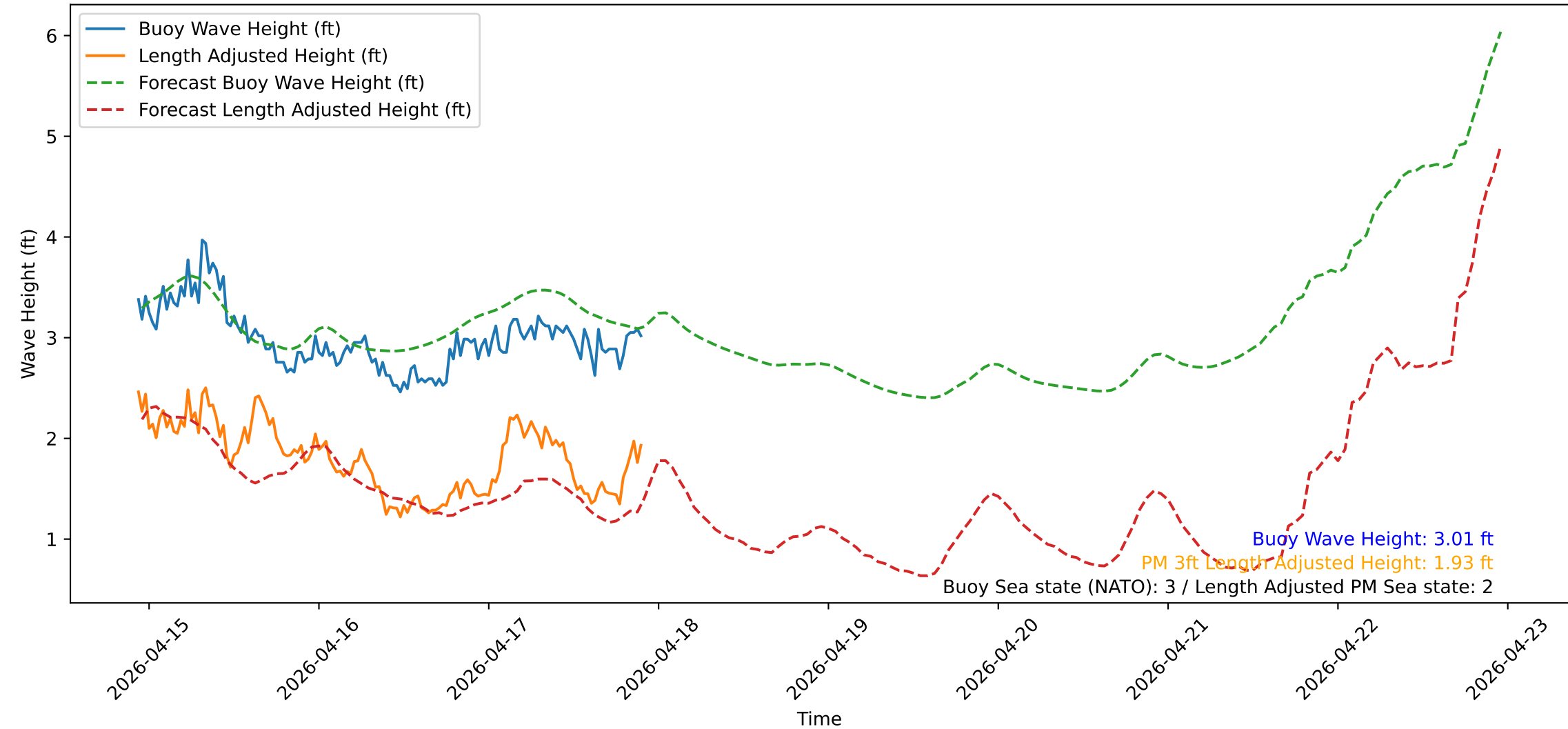
Wave Heights over Time for Green Beach at 2026-04-17 22:31:12
