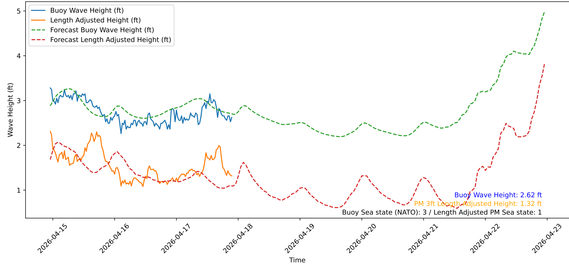
Wave Heights over Time for Red Beach at 2026-04-17 22:30:50
