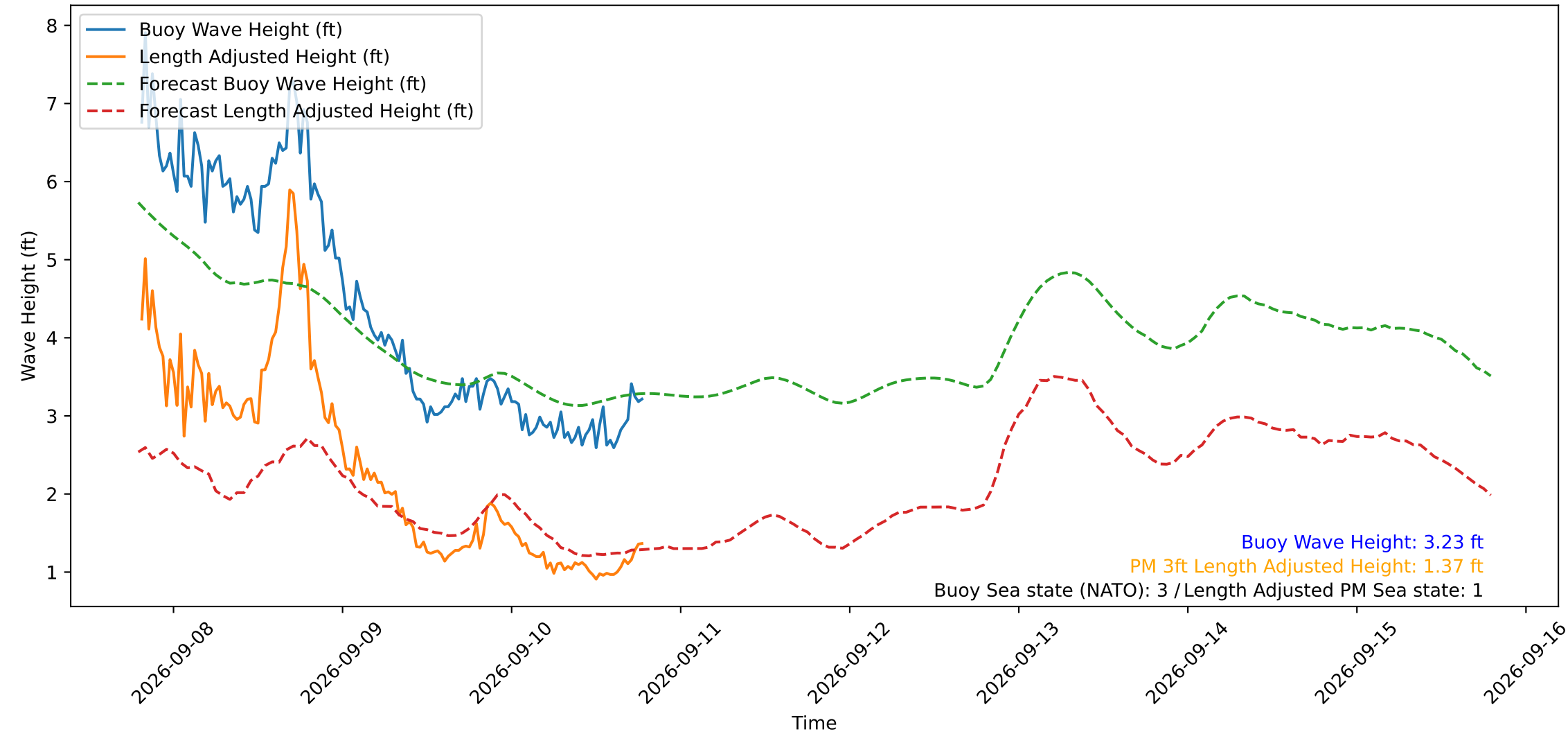
Wave Heights over Time for Green Beach at 2026-09-10 19:11:12
