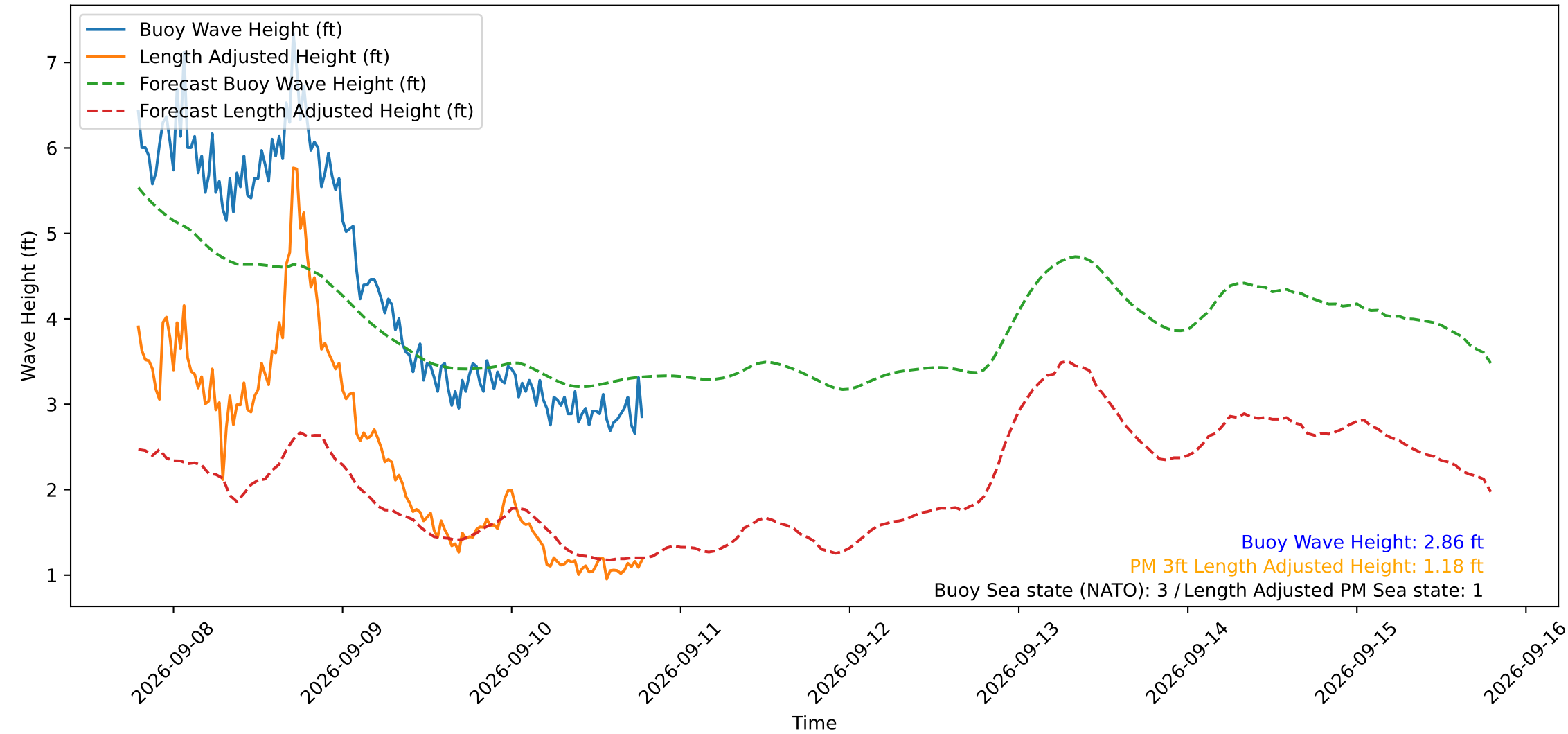
Wave Heights over Time for Oceanside Harbor at 2026-09-10 19:10:29
