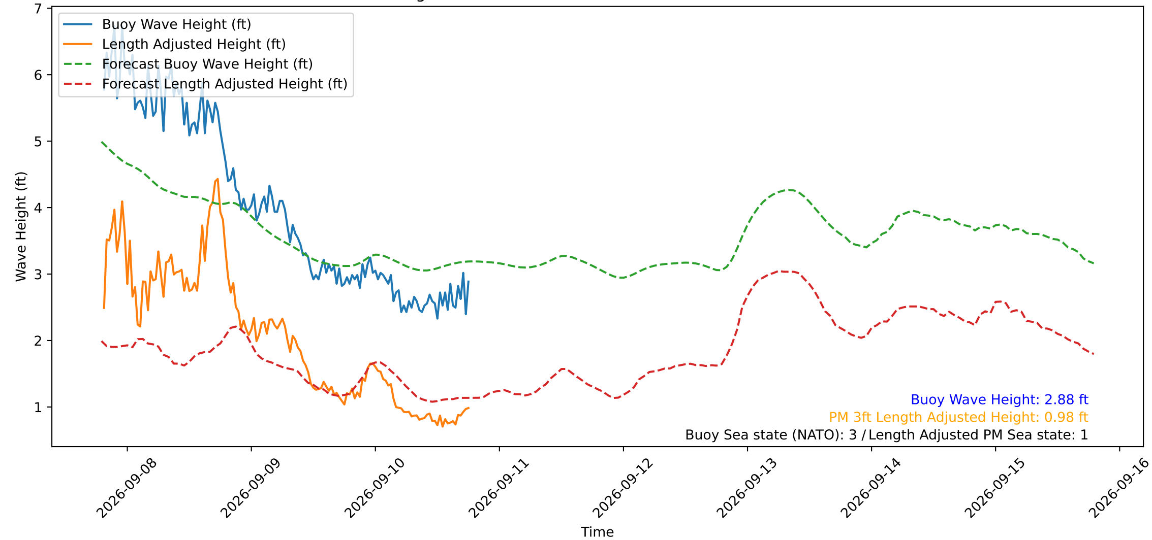
Wave Heights over Time for Red Beach at 2026-09-10 19:10:49
