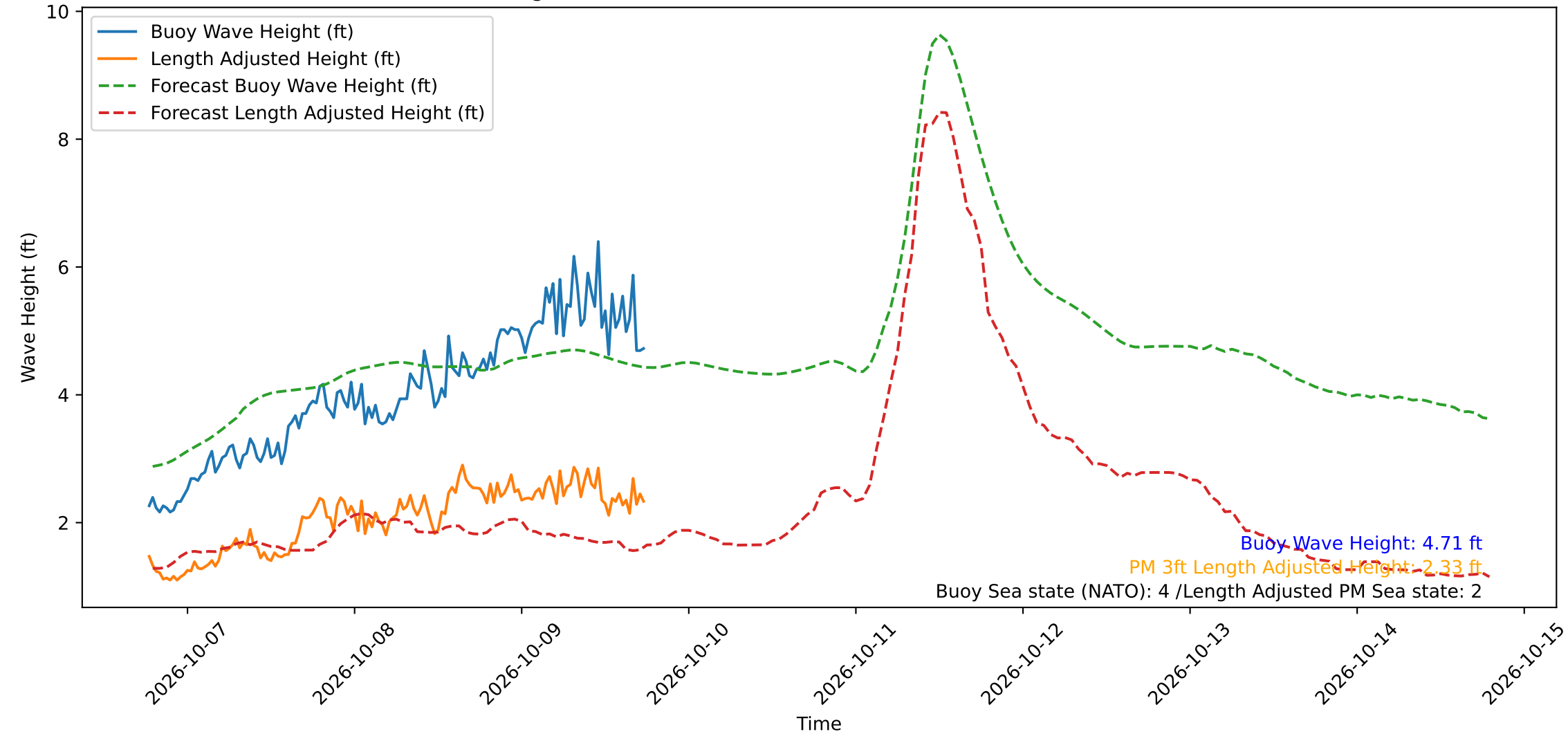
Wave Heights over Time for Oceanside Harbor at 2026-10-09 18:30:30
