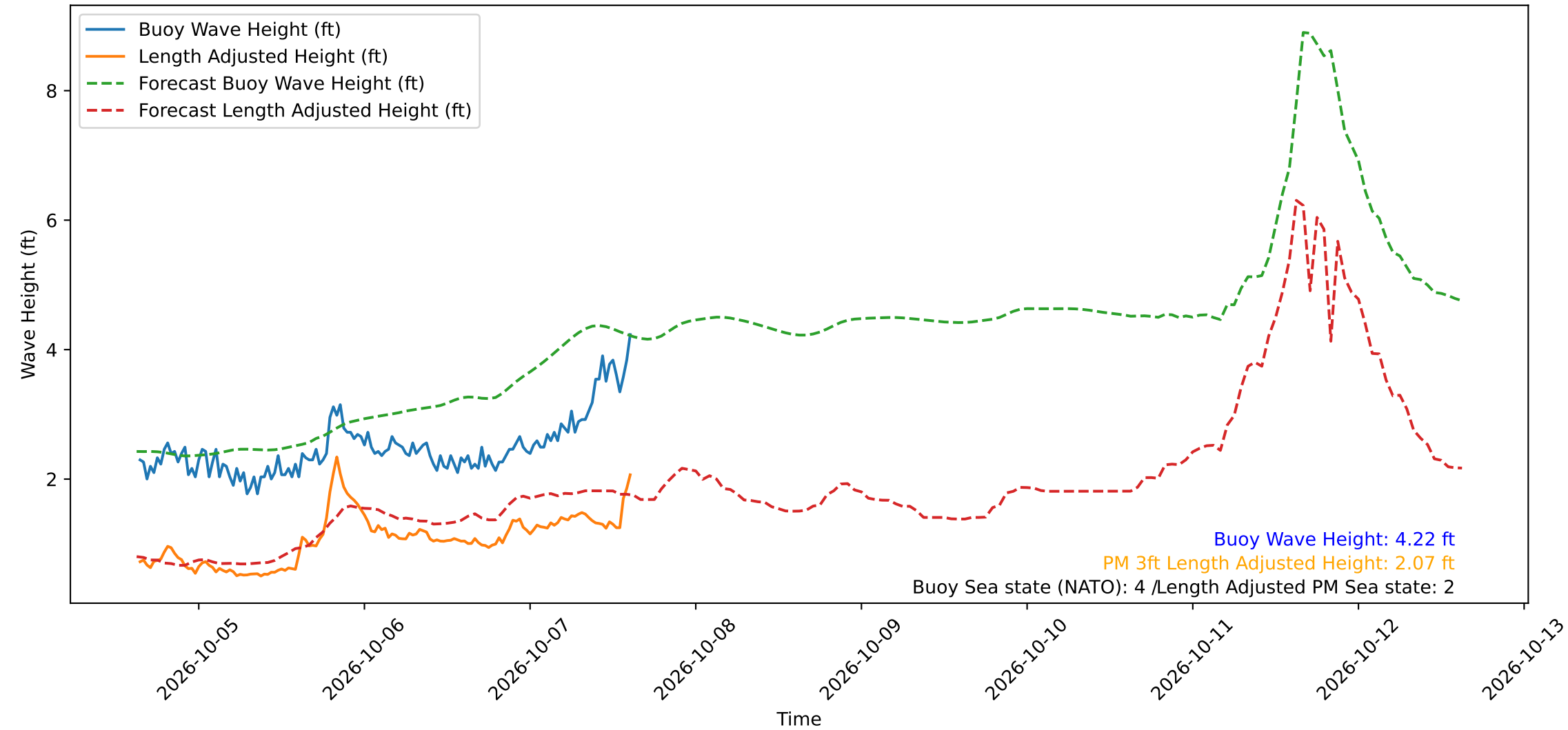
Wave Heights over Time for Green Beach at 2026-10-07 15:21:15
