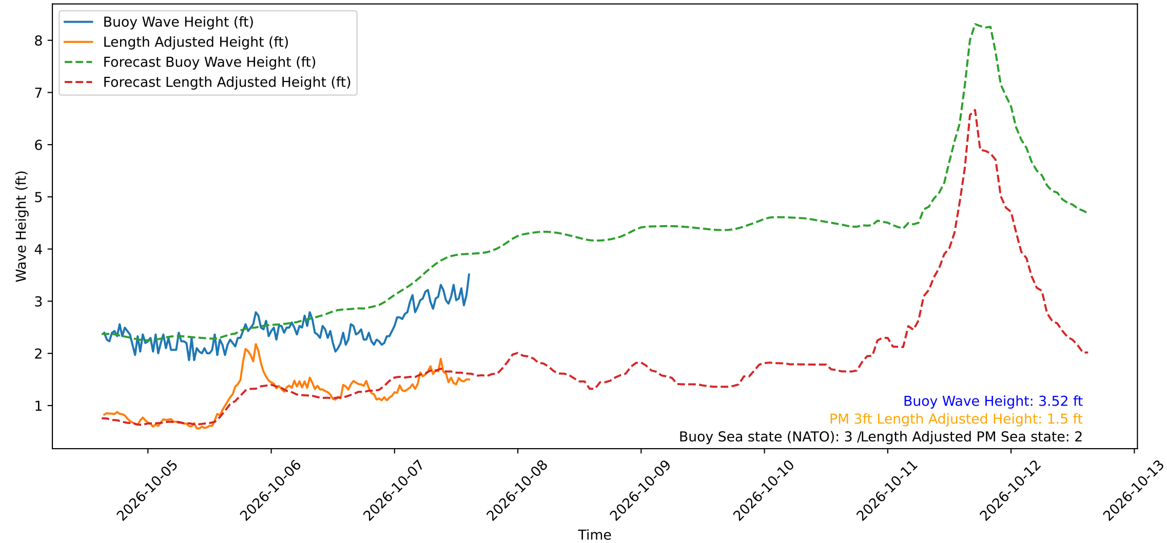
Wave Heights over Time for Oceanside Harbor at 2026-10-07 15:20:29
