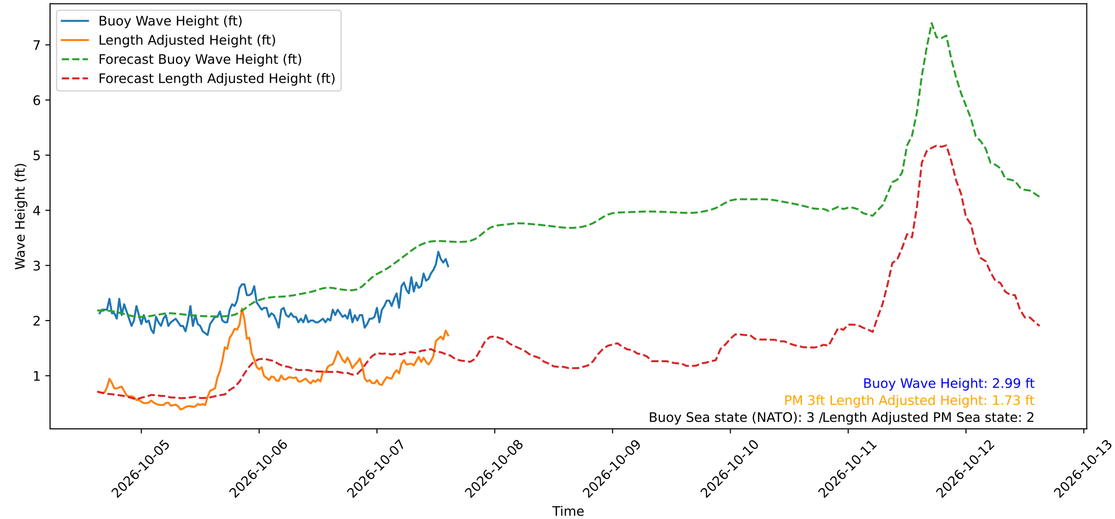
Wave Heights over Time for Red Beach at 2026-10-07 15:20:51
