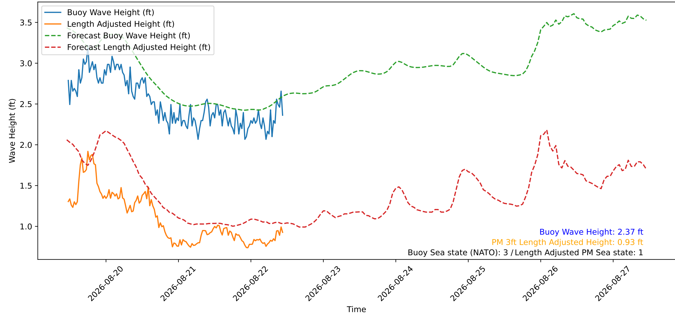
Wave Heights over Time for Red Beach at 2026-08-22 11:20:50
