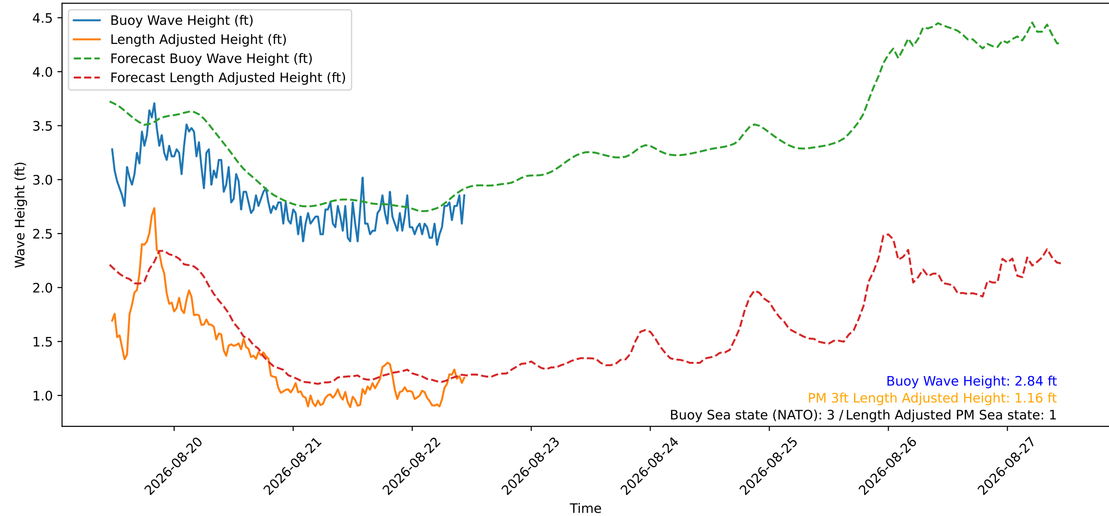
Wave Heights over Time for Green Beach at 2026-08-22 11:21:14
