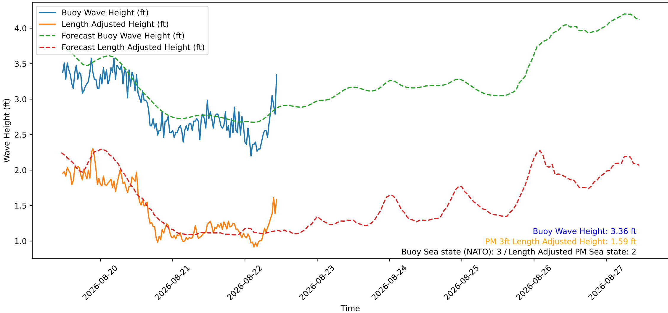
Wave Heights over Time for Oceanside Harbor at 2026-08-22 11:20:29
