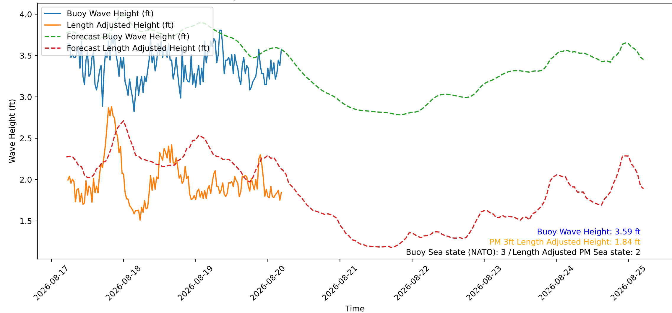
Wave Heights over Time for Oceanside Harbor at 2026-08-20 05:20:27
