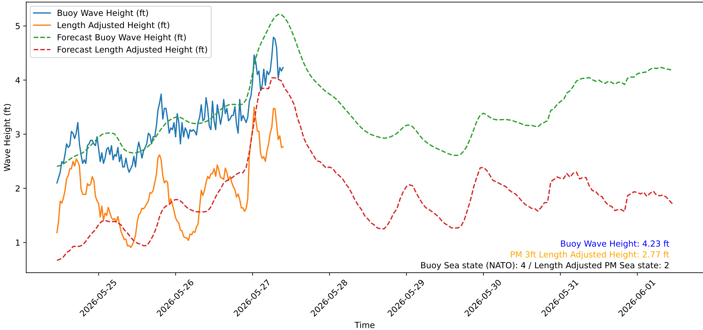
Wave Heights over Time for Red Beach at 2026-05-27 10:30:45
