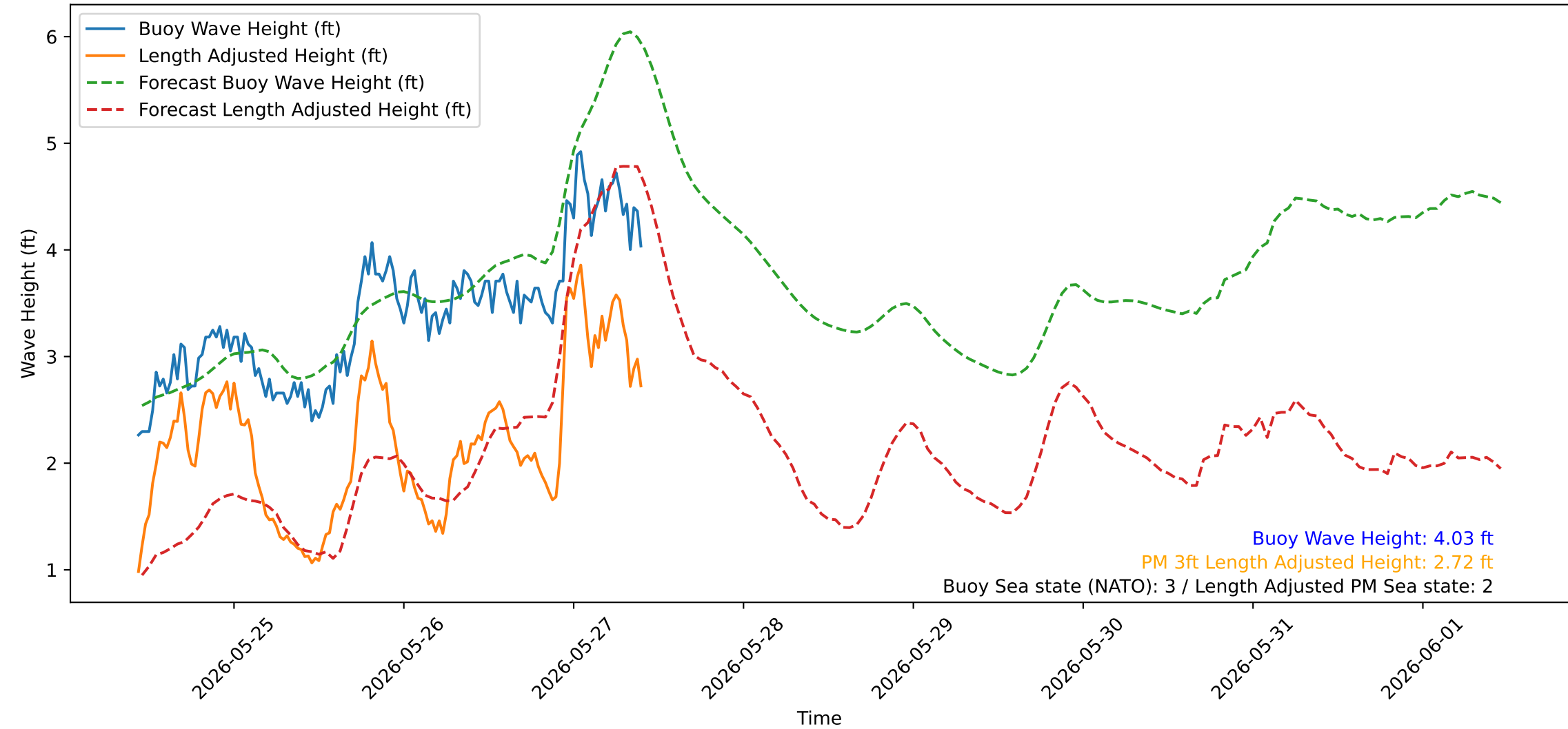
Wave Heights over Time for Green Beach at 2026-05-27 10:31:08
