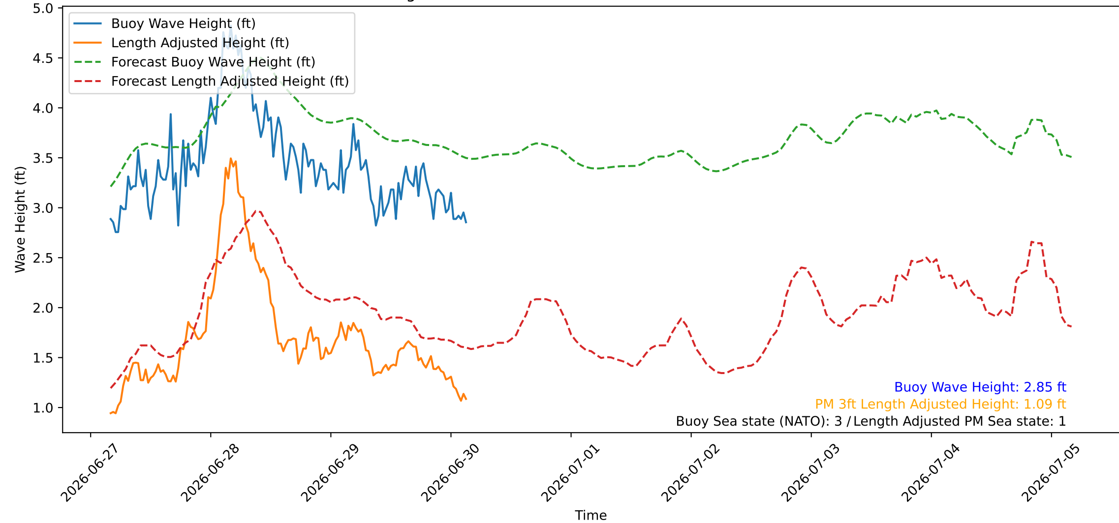
Wave Heights over Time for Green Beach at 2026-06-30 04:01:08
