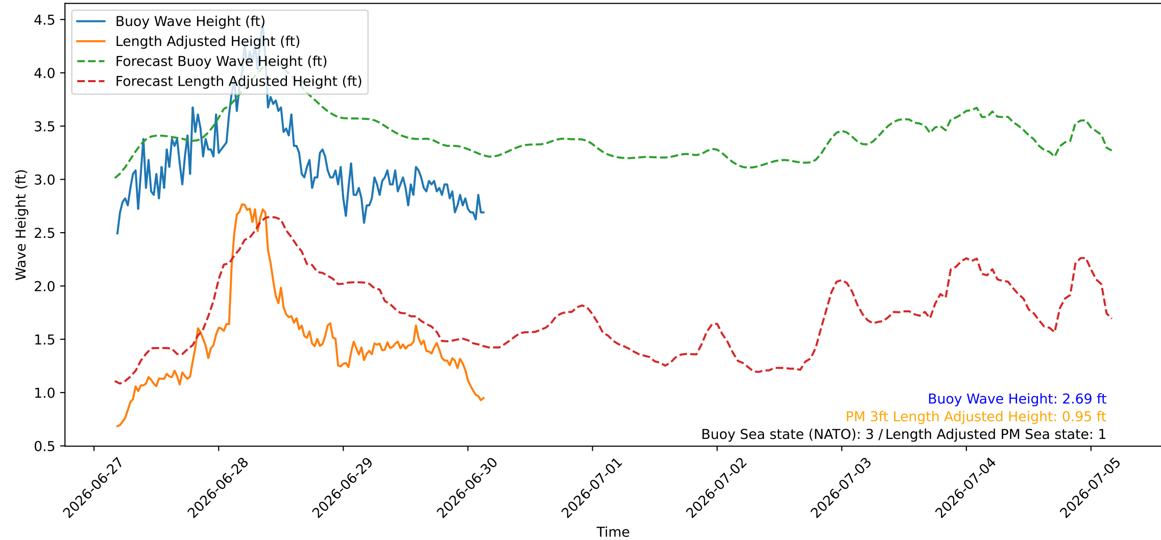
Wave Heights over Time for Red Beach at 2026-06-30 04:00:46
