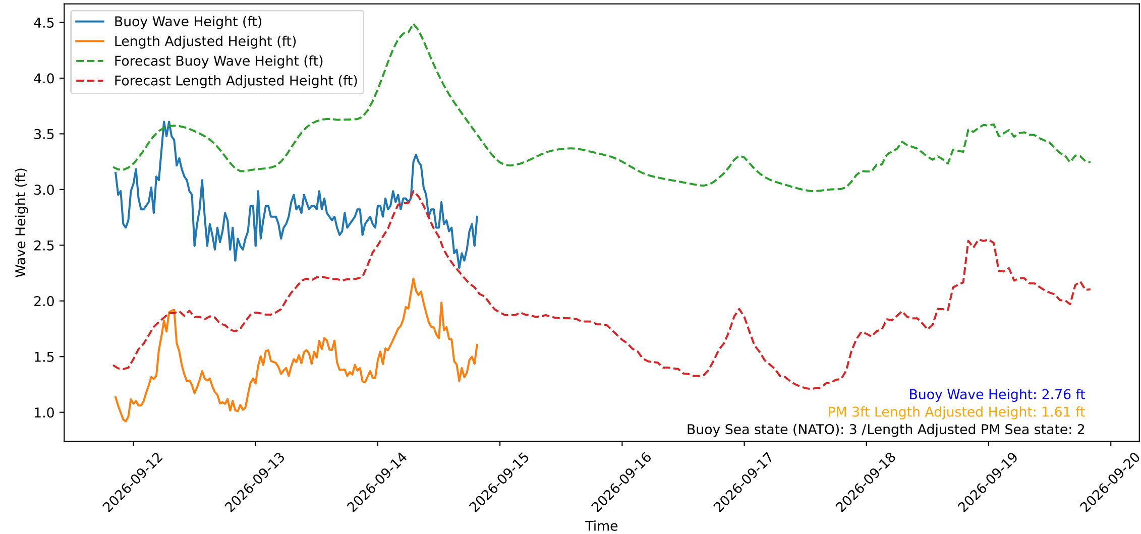
Wave Heights over Time for Green Beach at 2026-09-14 20:11:12
