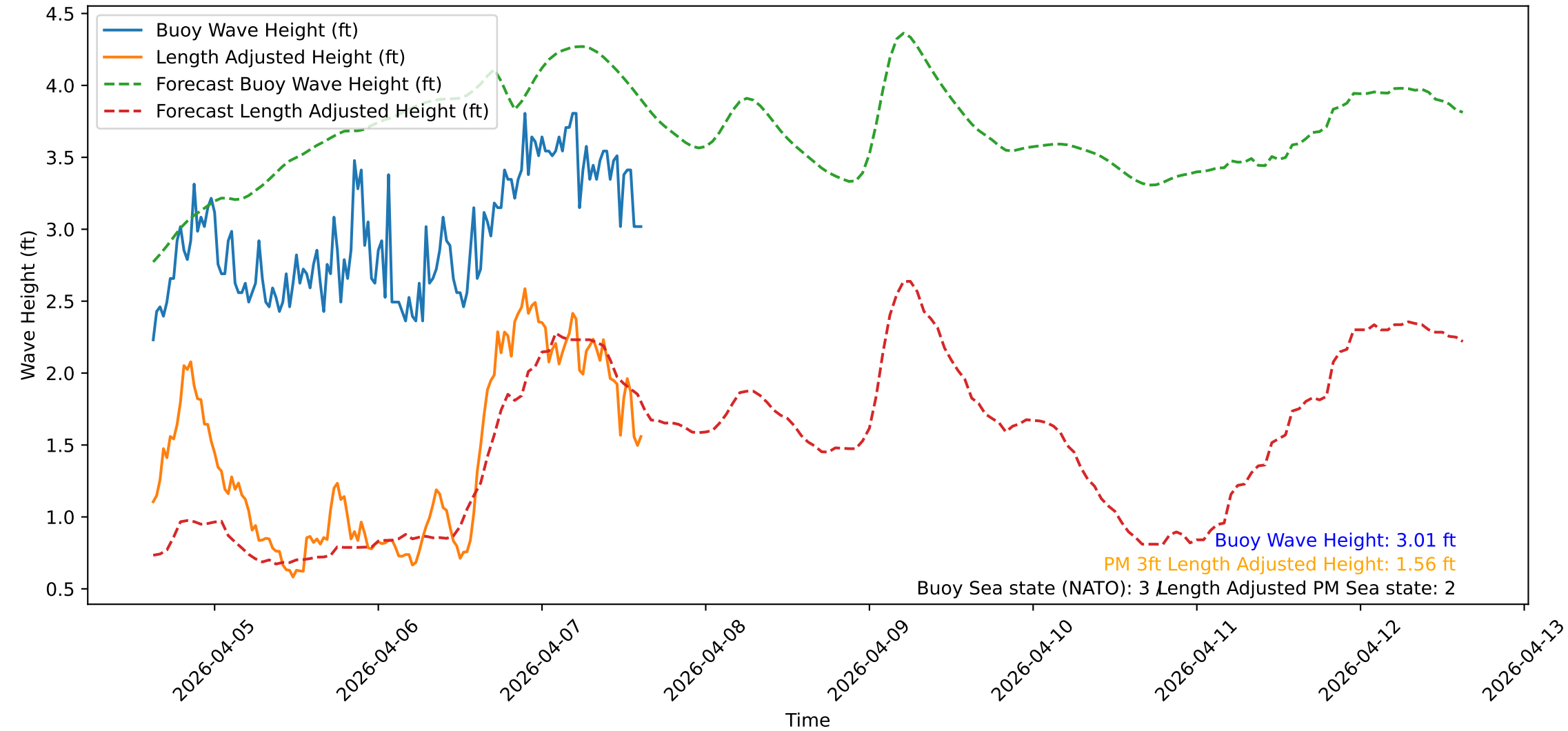
Wave Heights over Time for Green Beach at 2026-04-07 15:11:10
