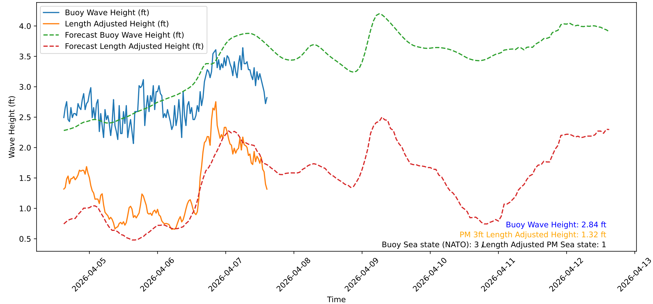
Wave Heights over Time for Oceanside Harbor at 2026-04-07 15:10:31
