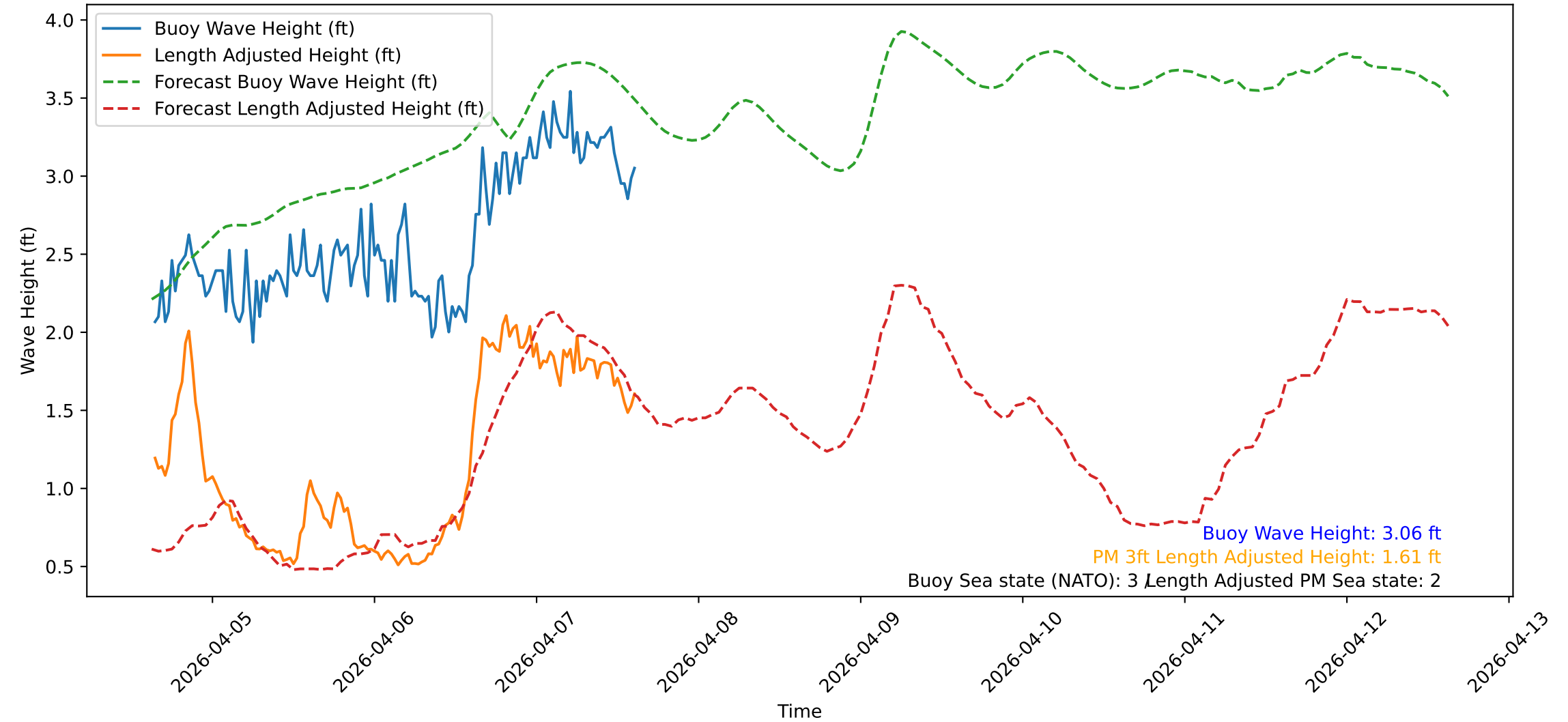
Wave Heights over Time for Red Beach at 2026-04-07 15:10:47
